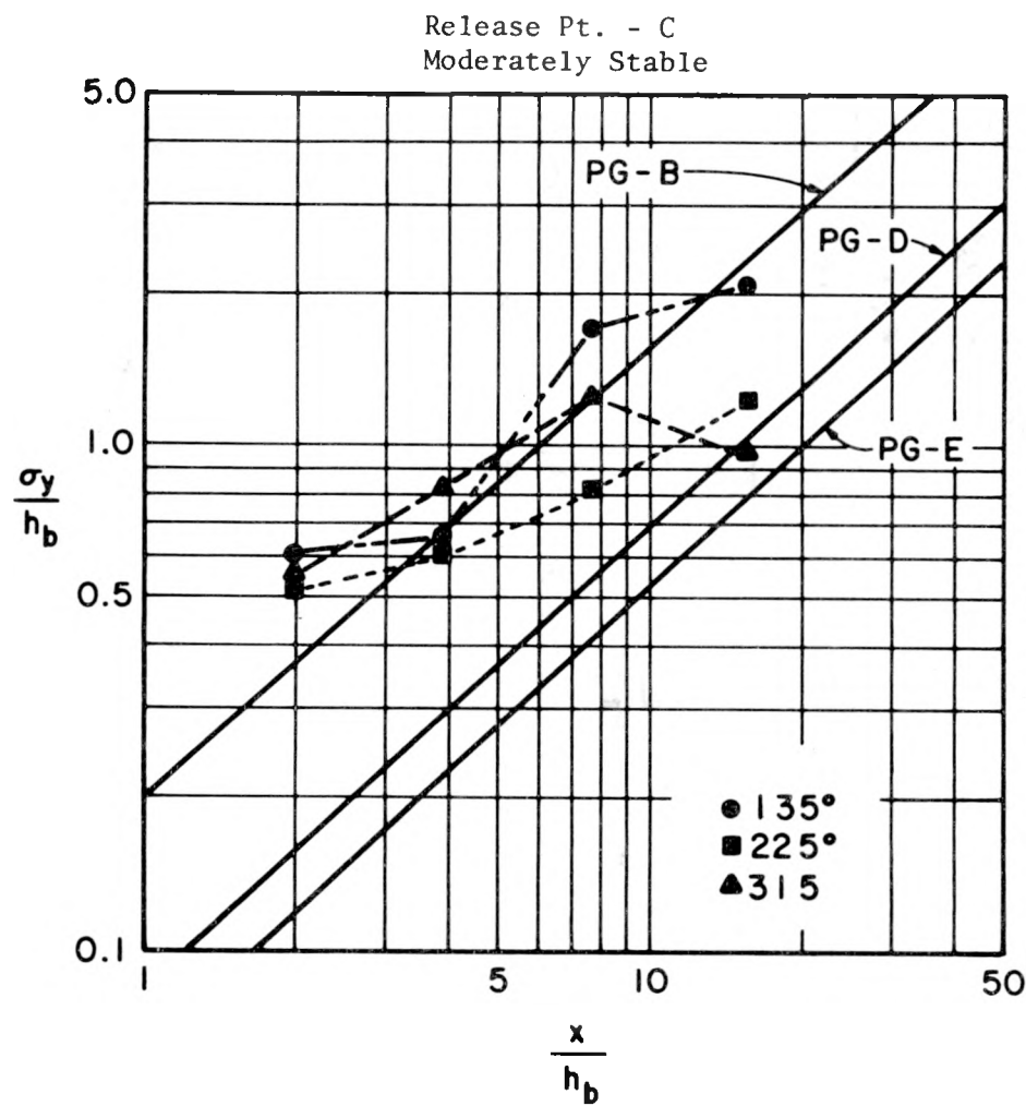
Figure 32. Plot of \sigma_y/h_b versus x/h_b for Release Point C
