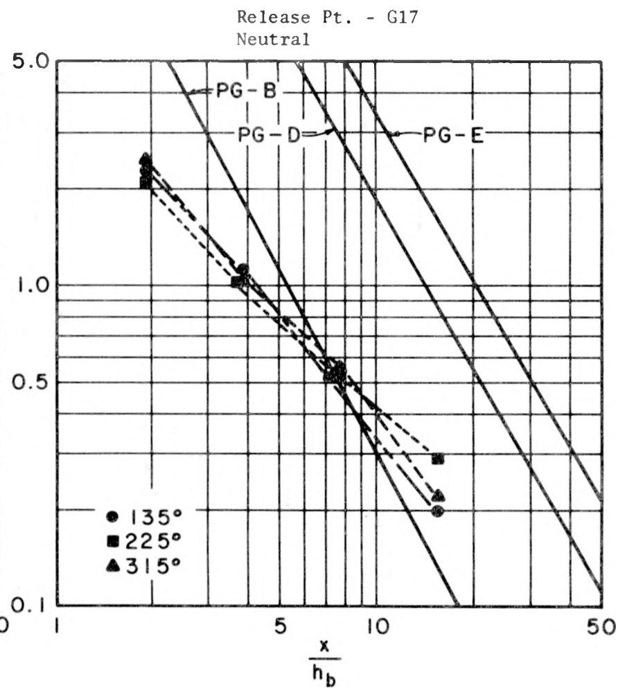
Figure 29. Plot of Maximum K_c Versus x/h_b for Release Point G17.
