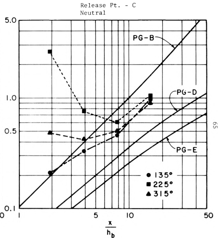
Figure 35. Plot of \sigma_z/h_b versus x/h_b for Release Point C.
