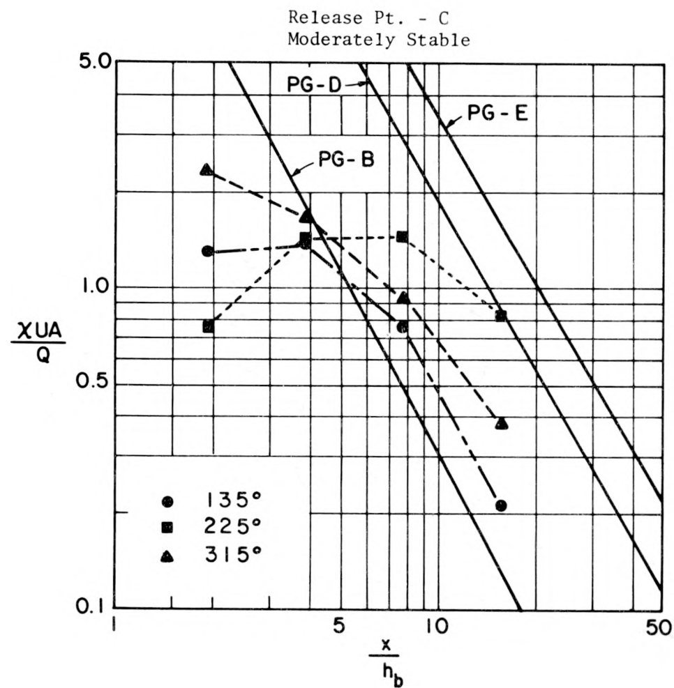
Figure 28. Plot of Maximum K_c Versus x/h_b for Release Point C
