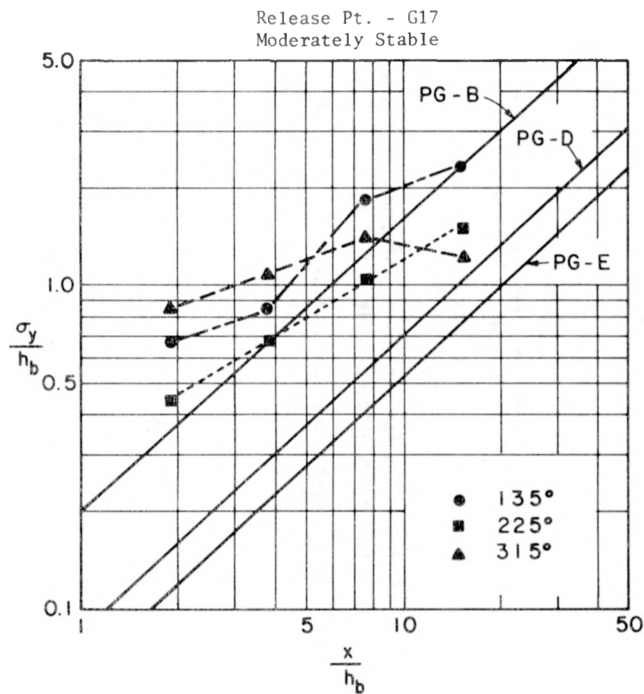
Figure 33. Plot of \sigma_y/h_b Versus x/h_b for Release Point G17
