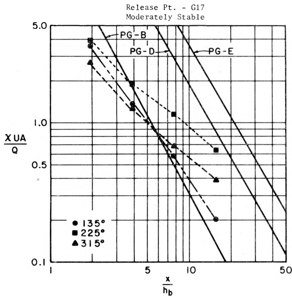
Figure 29. Plot of Maximum K_c Versus x/h_b for Release Point G17.
