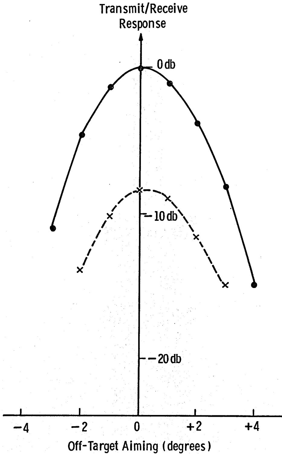
Figure 10.10 Transmit/receive beam pattern for experiemntal sensor at R.T. (solid) and at 300°F (broken).
