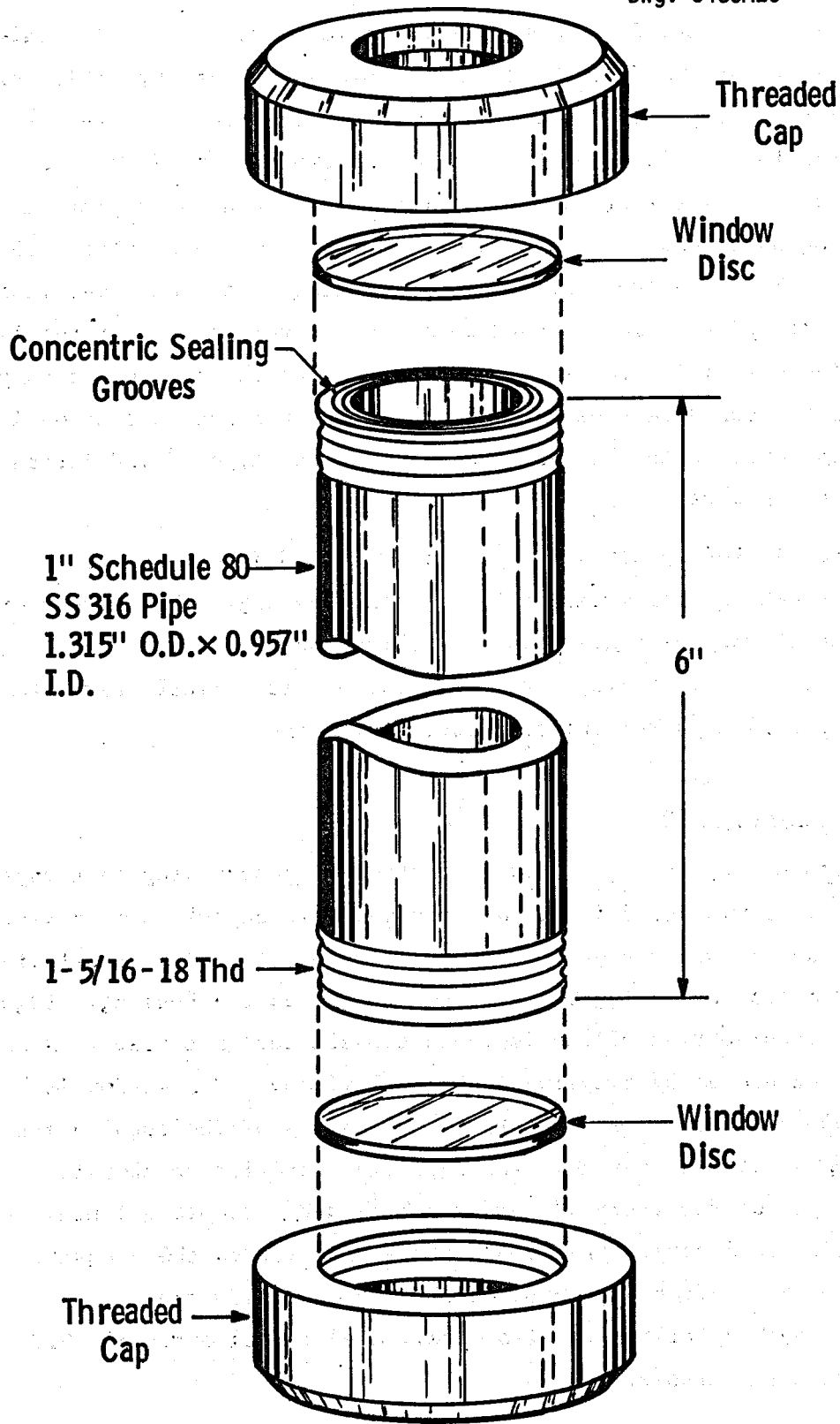
Figure 5.1. Assembly drawing of capsule for early screening tests.
