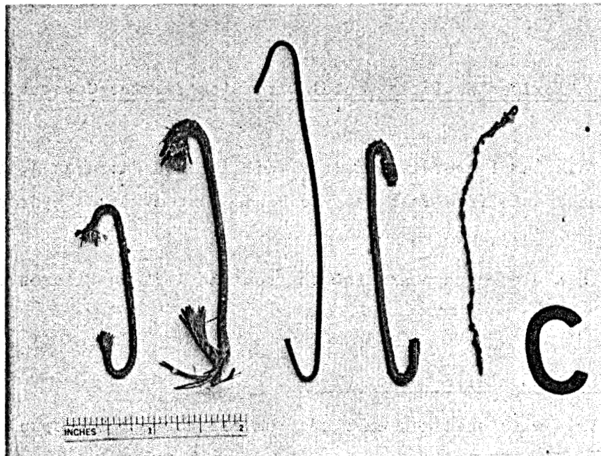
Fig. 17. Post-test Photograph of Test Capsule C Wire Samples
