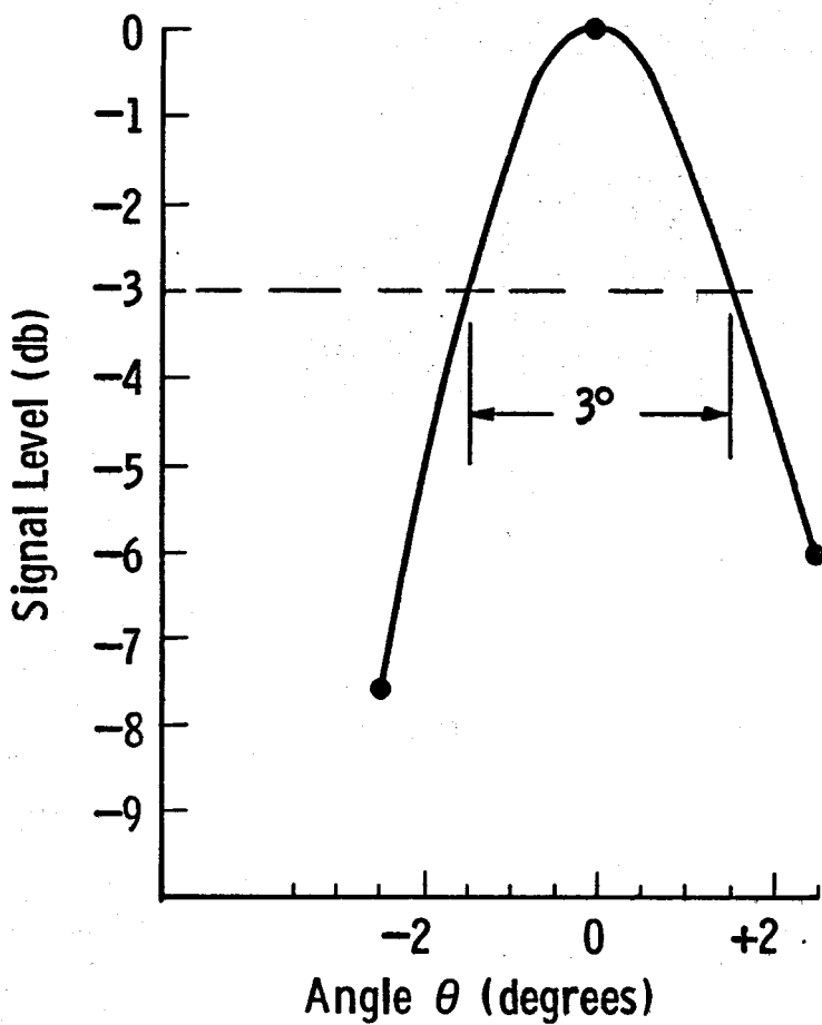
Figure 10. Transmit/receive beam pattern; 3-3/8" tool; 4.75" range.
