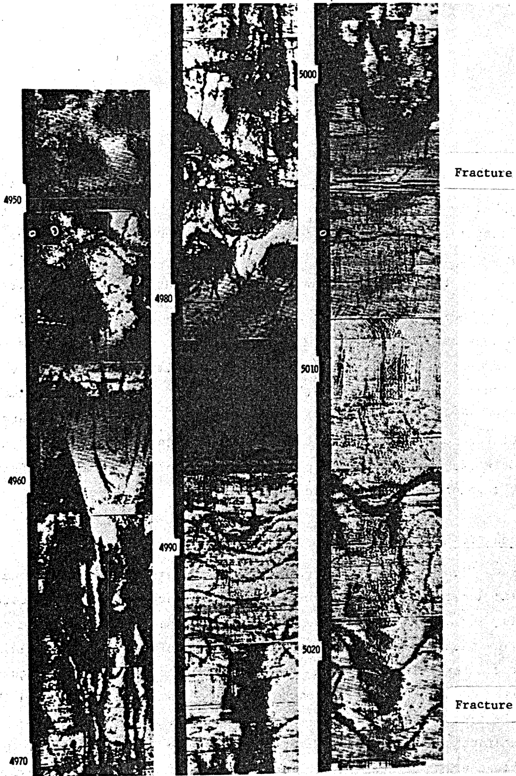
Figure 2.3. Three borehole televiwer logs in fractured West Texas Precambrian Formation. Wellbore filled with drilling mud. (Reproduced from and with permission of Journal of Petroleum Technology 3 ).
