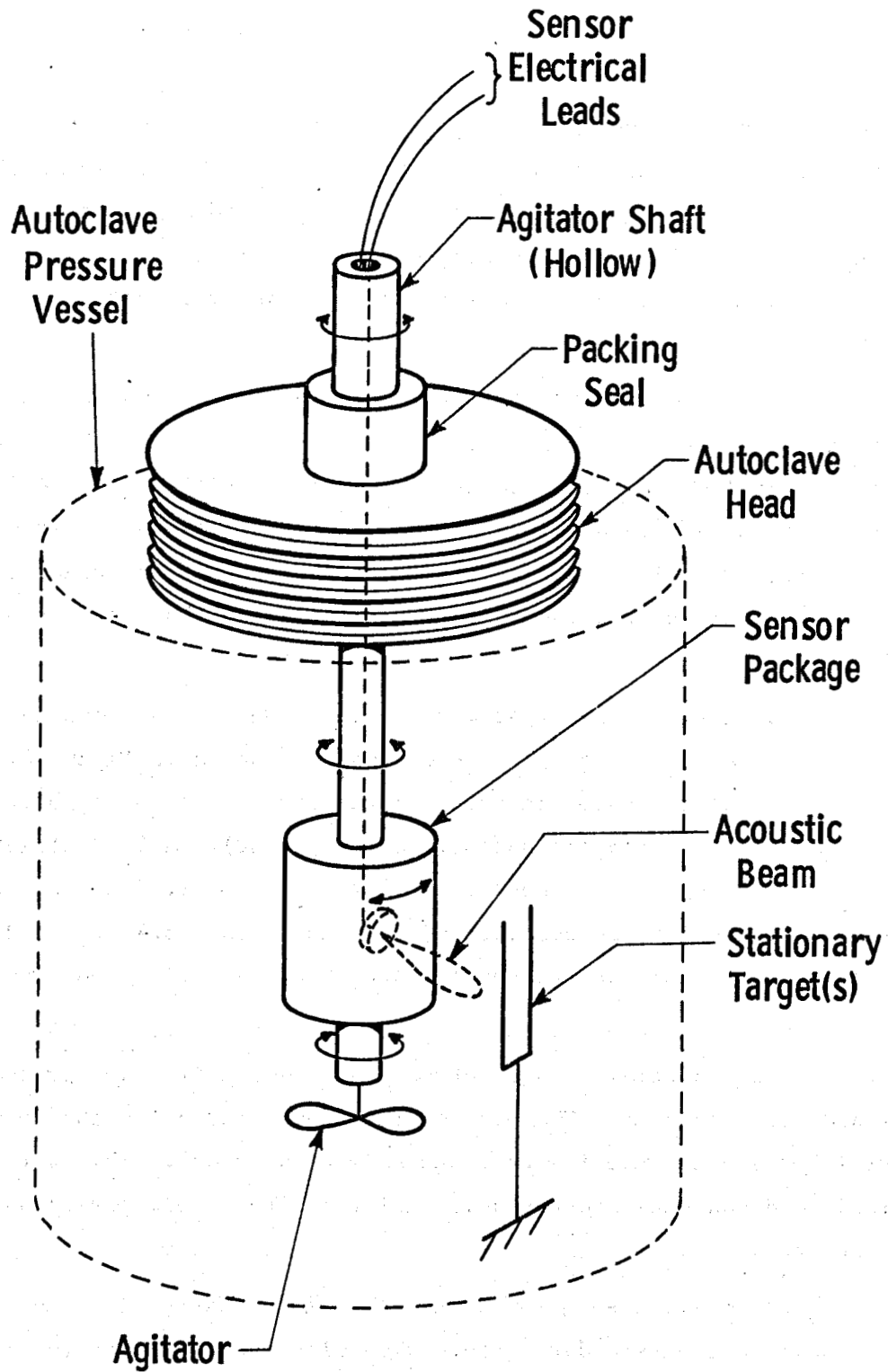
Figure 8.1. Basic test concept for evaluating experimental sensor.
