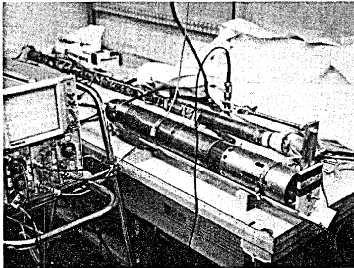
Figure 3. Fixture and Reference Sensor Installed on BHTV @ USGS.
