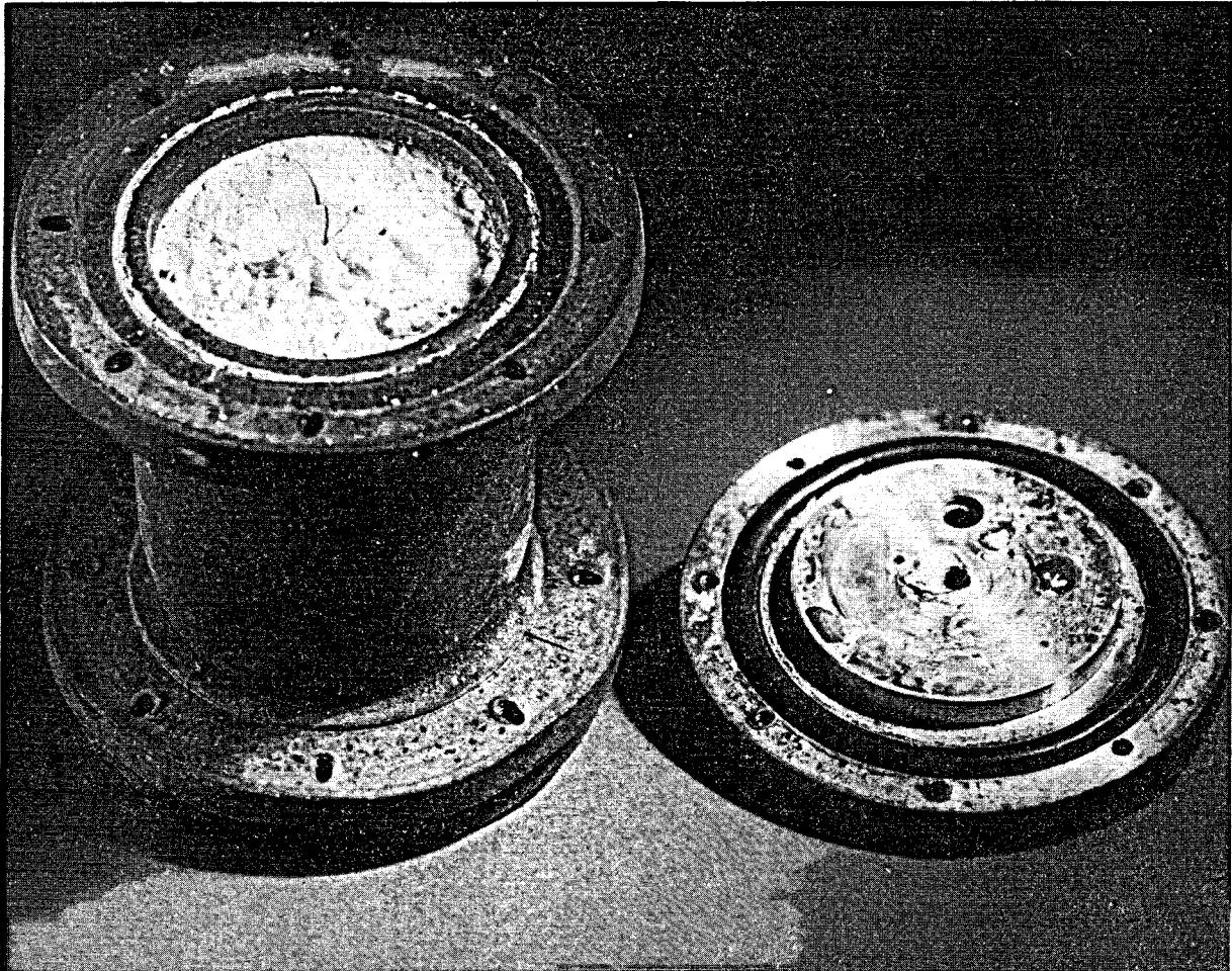
Figure 5.10 Although the Ryton window (left) remained intact, the DC-710 internal fluid apparently reacted with the window, forming the white powder shown in photo. Flange retainer screw holes and o-ring (Kalrez 1050) seal surface show evidence of considerable plastic deformation. Top flange with o-ring shown at right.
