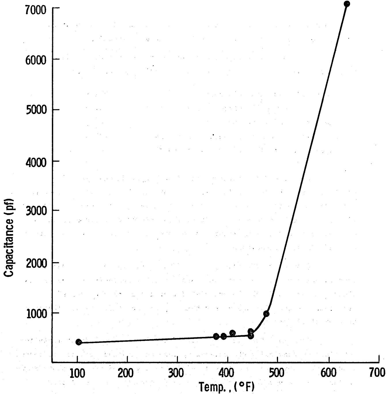
Figure 11.9. Plot of measured transducer capacitance vs. temperature.
