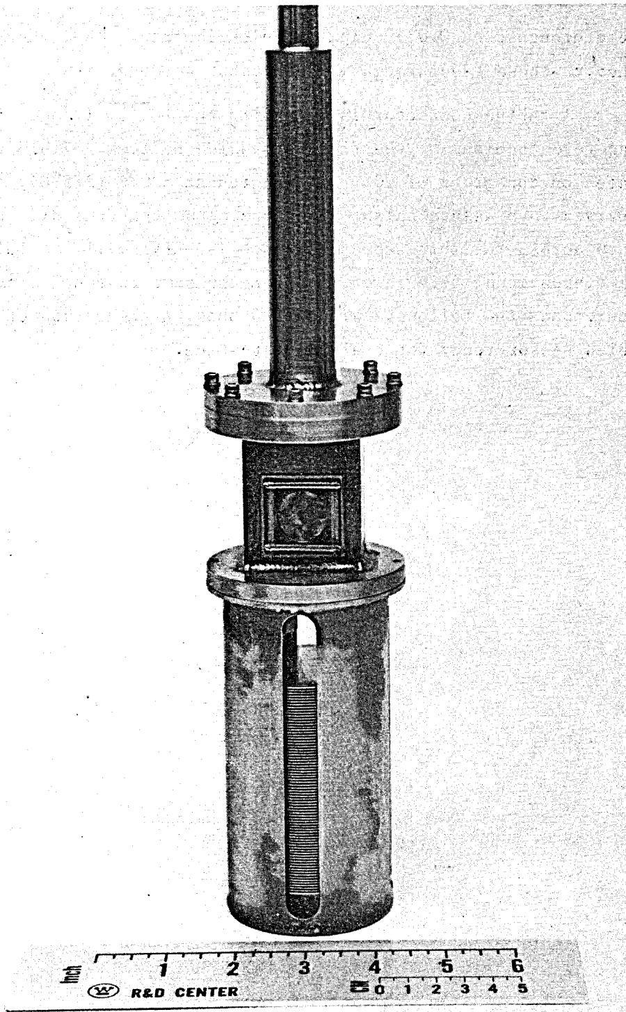
Figure 8.6. Photograph of fabricated experimental acoustic sensor concept.
