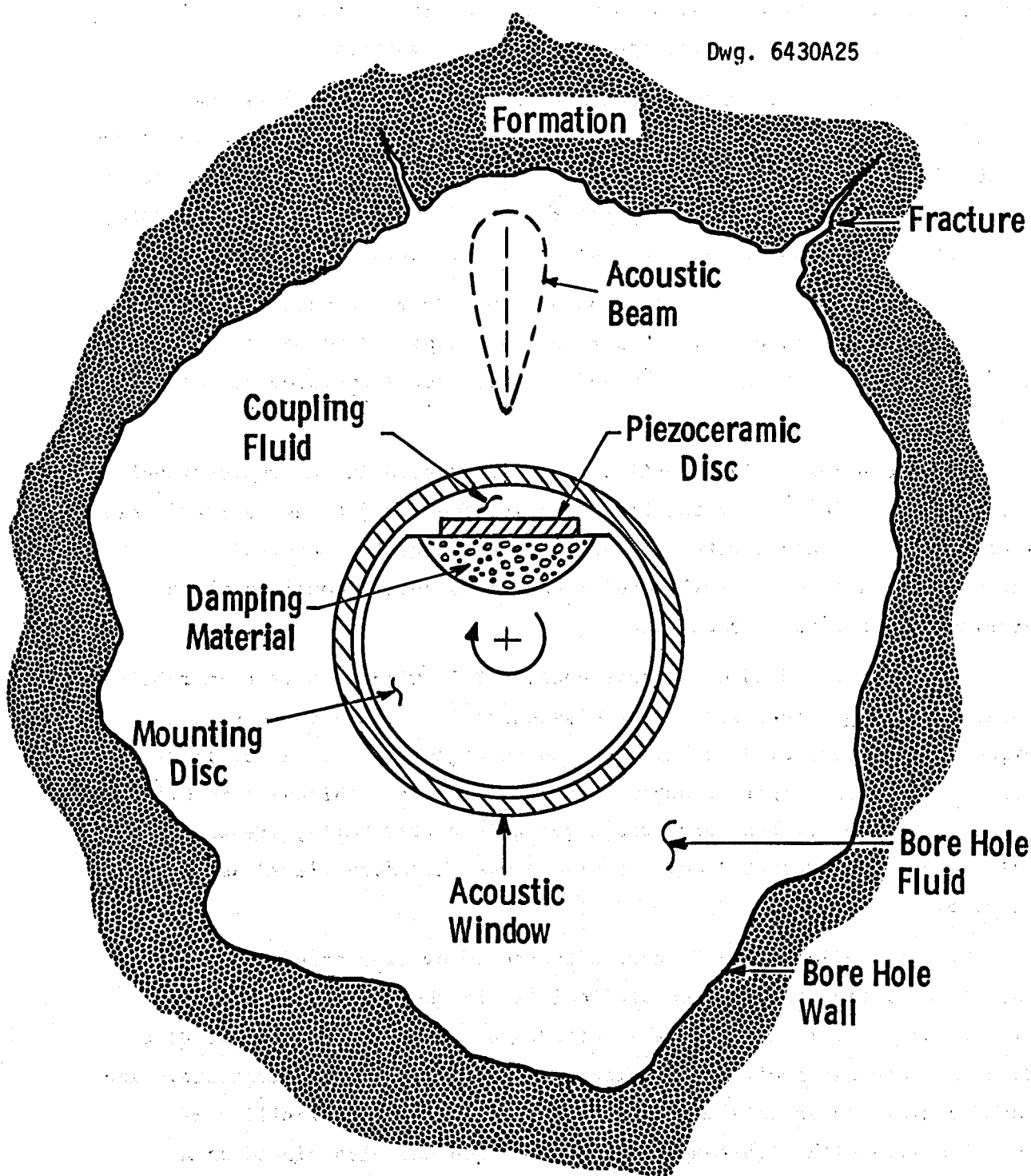
Figure 3.1. Cross-section diagram indicating construction of conventional BHTV tools.
