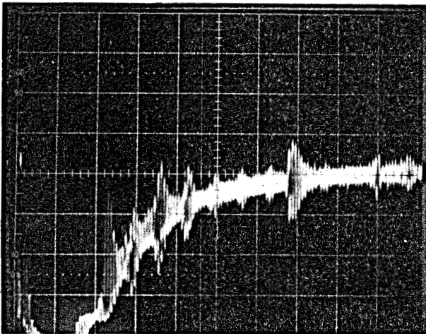
Figure 10.8. Echo pattern from 3/16" dia. rod in simulated geofluid. T = 480°F; P = 5725 psi. Horizontal = 10 \mu sec/div. Vertical = 0.5 Volt/div.
