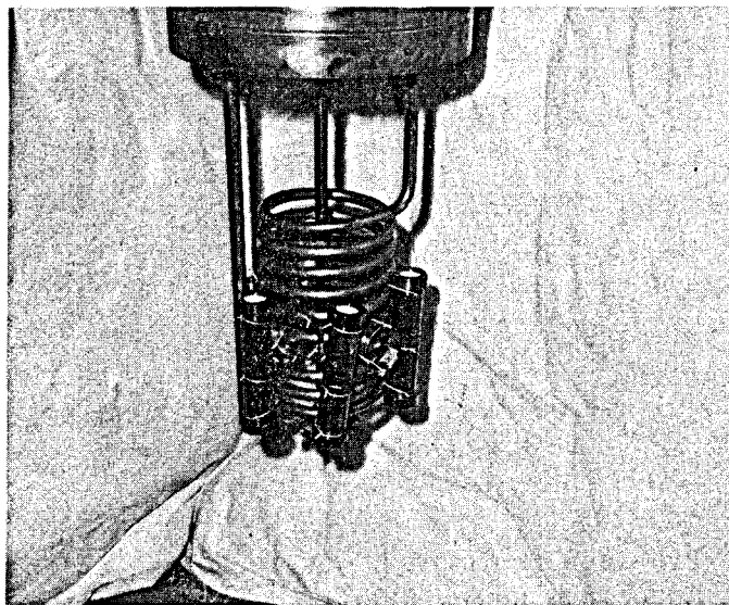
Fig. 4. Pre-Test Photograph of Test Capsules Fastened to Autoclave Cooling Coil
