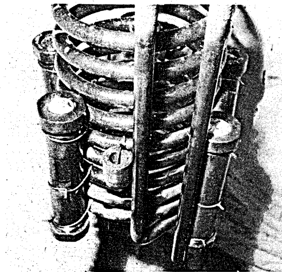
Fig. 15. Post-Test Photograph of Test Capsules Fastened to Autoclave Cooling Coil
