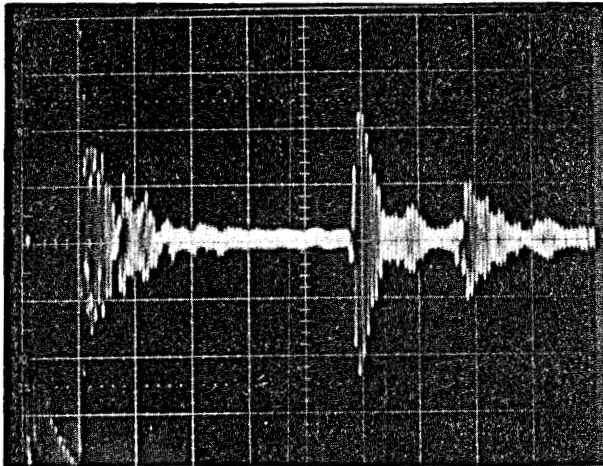
Figure 10.7. Echo pattern from 3/16" dia. rod in simulated geofluid. T = 70°F; P = 295 psi. Horizontal = 10 \mu sec/div. Vertical = 0.5 Volt/div.
