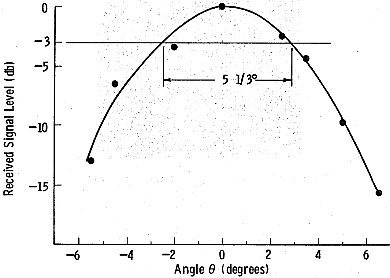
Figure 12. Transmit beam pattern; 1-3/4" tool; range - 4.75".
