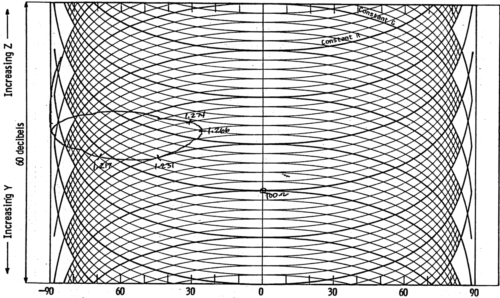
Fig. 11.17 Log Vector Impedance Plot (0.3 - 1.5 MHz) for "spare" transducer assembly of Fig. 5, at R.T., following thermal cycle test.
