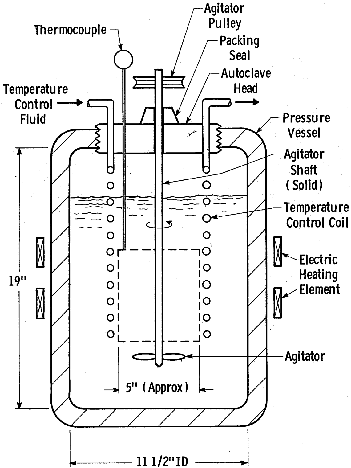
Figure 4.2 Diagram of 10-gallon autoclave vessel used for geothermal simulation testing.
