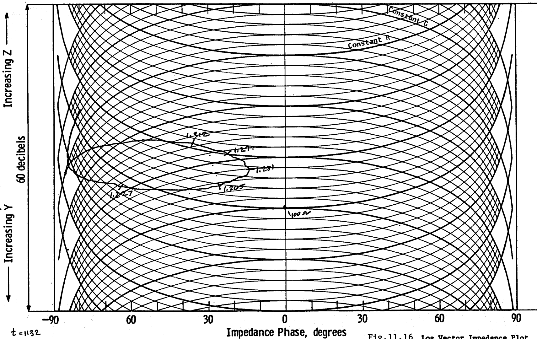
Fig. 11.16 Log Vector Impedance Plot (0.3 - 1.5 MHz) for "spare" transducer assembly of Fig. 5. Temperature = 604°F.
