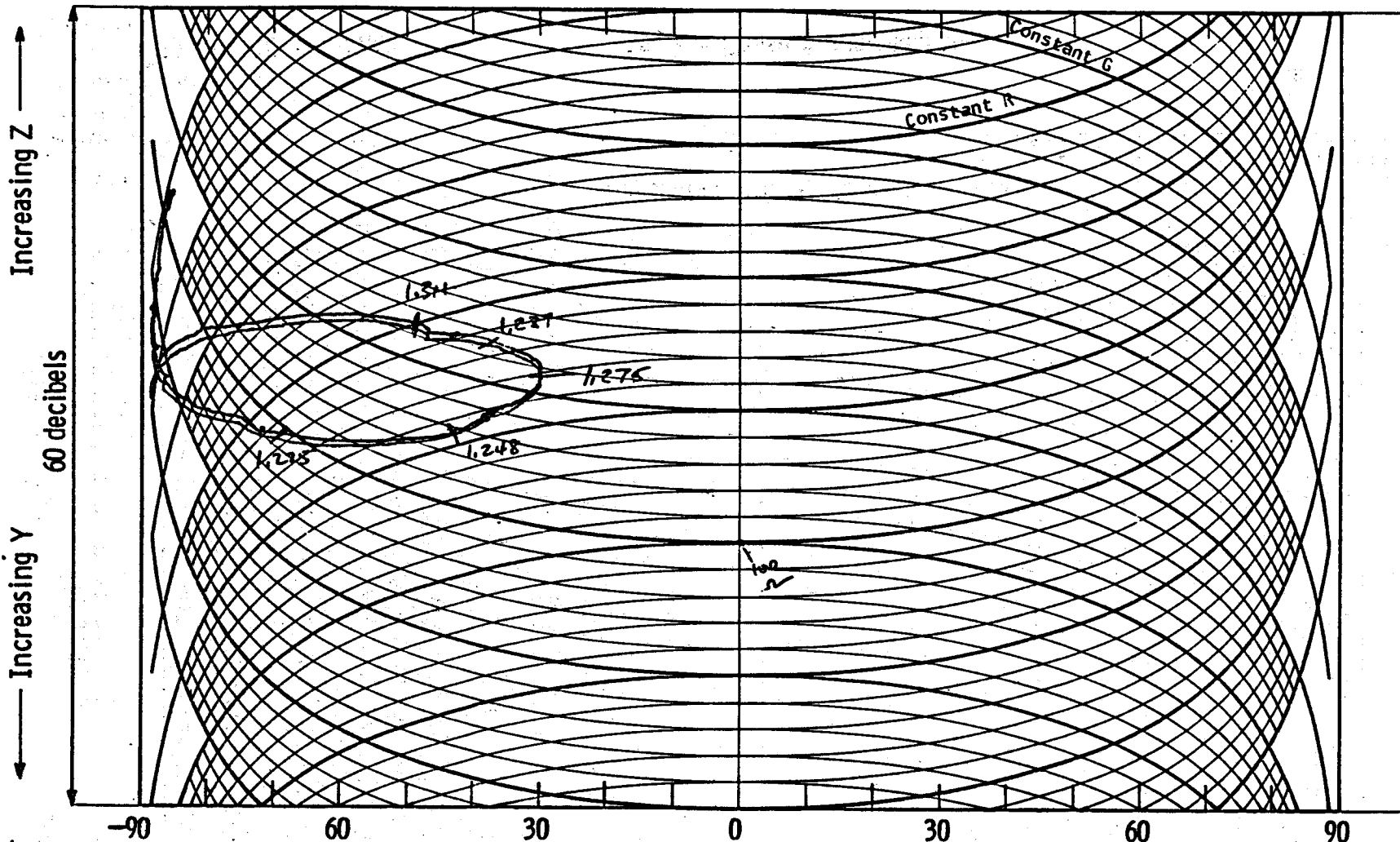
Fig.11.11 Log Vector Impedance Plot (0.3 - 1.5 MHz) for "spare" transducer assembly of Fig. 5, at R.T., before 650°F thermal cycle test.
