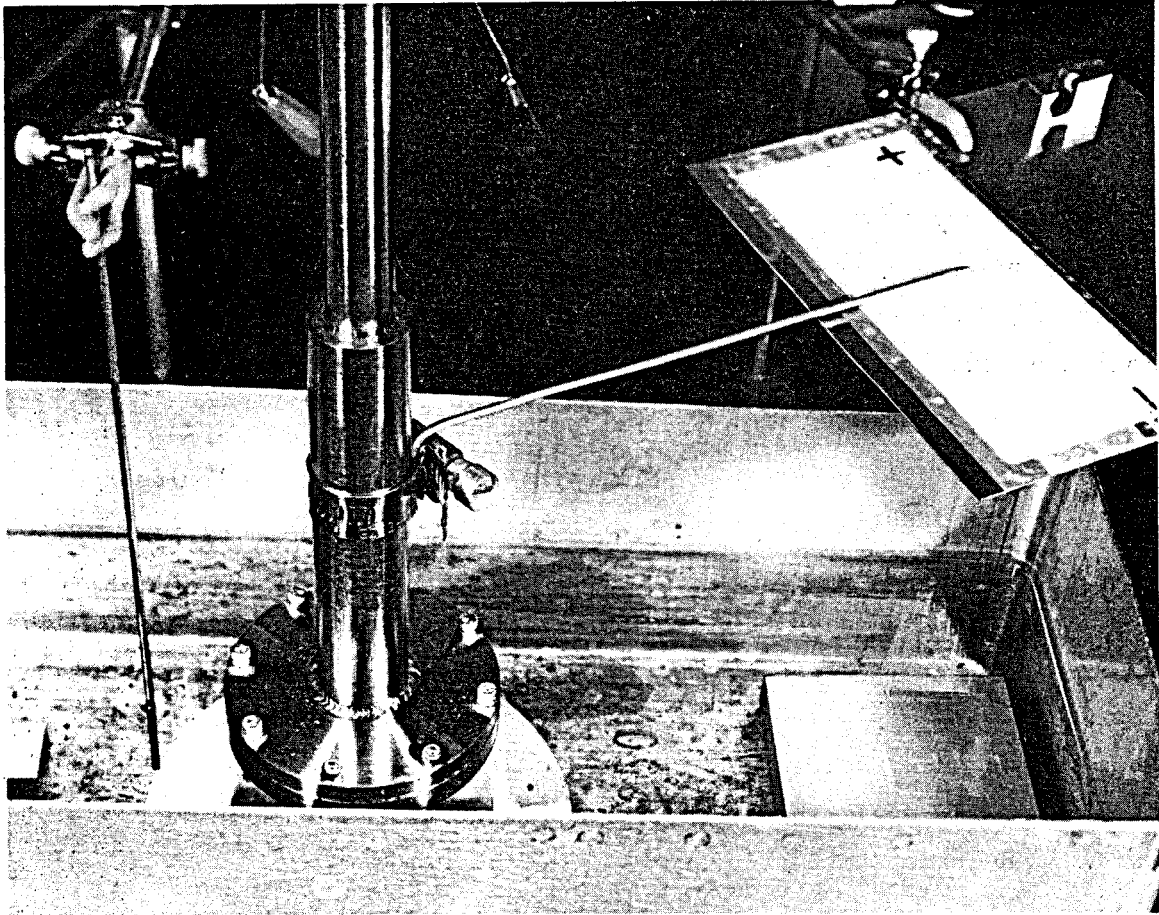
Figure 9.1. Apparatus used to measure beam pattern of Experimental Geothermal Sensor.
