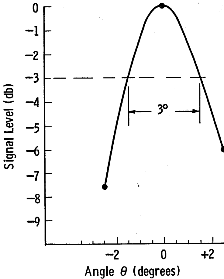
Figure 9.3. Transmit-receive pattern for a USGS BHTV sensor, measured in room-temperature water.
