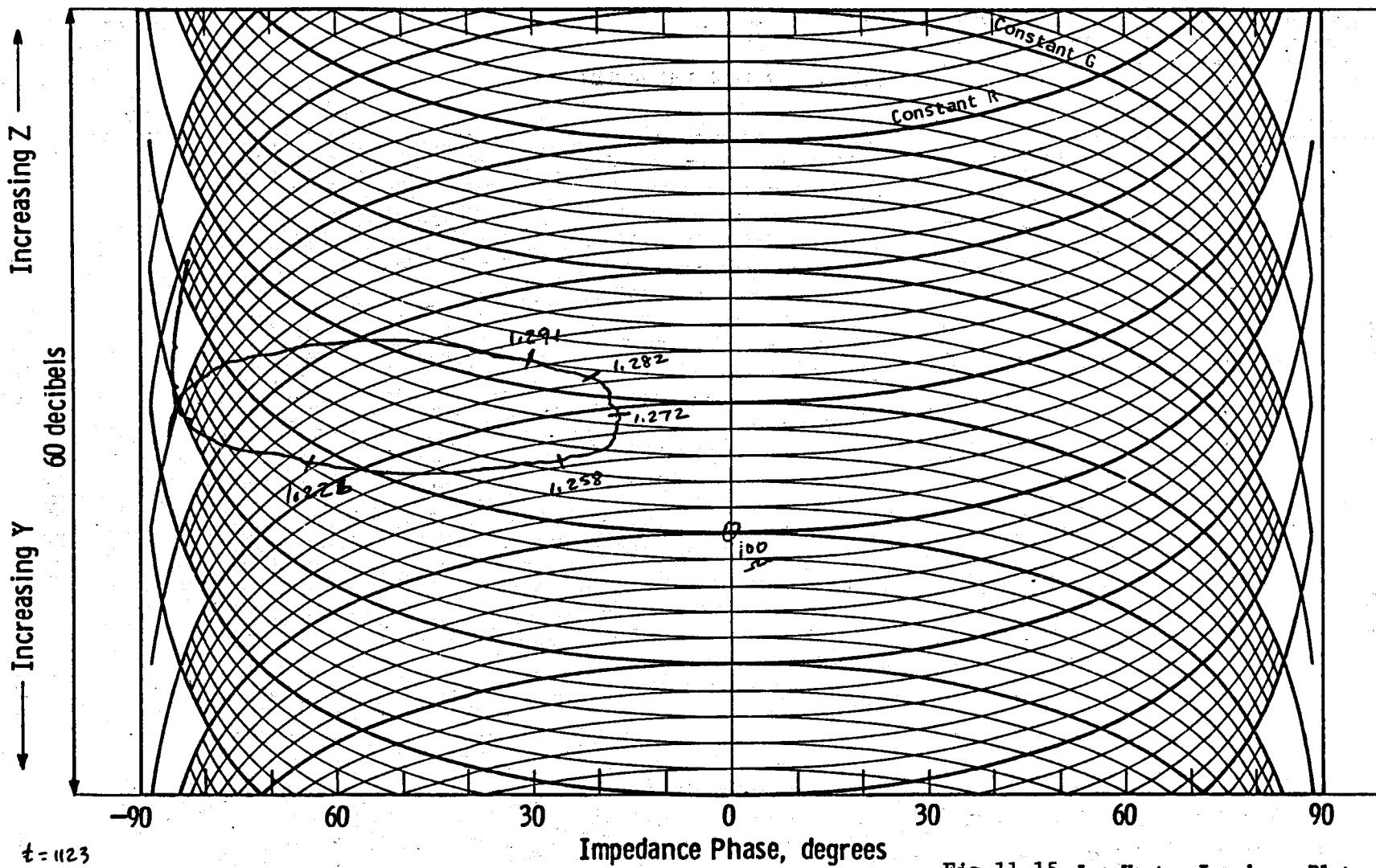
Fig. 11.15 Log Vector Impedance Plot (0.3 - 1.5 MHz) for "spare" transducer assembly of Fig. 5. Temperature = 505°F.
