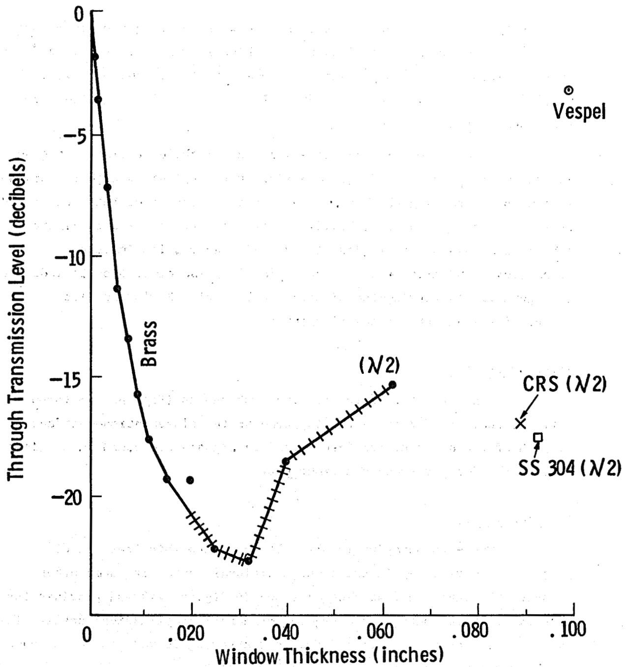
Figure 7.3 Experimental verification of window performance predicted from analytical solutions. Solid line is for brass shim-stock of various thicknesses up to 0.062-inches. Waveform phase distortions occur in region of herring-bone. Performance of half-wavelength carbon and stainless steels also plotted along with that of a commercial Vespel BHTV window.
