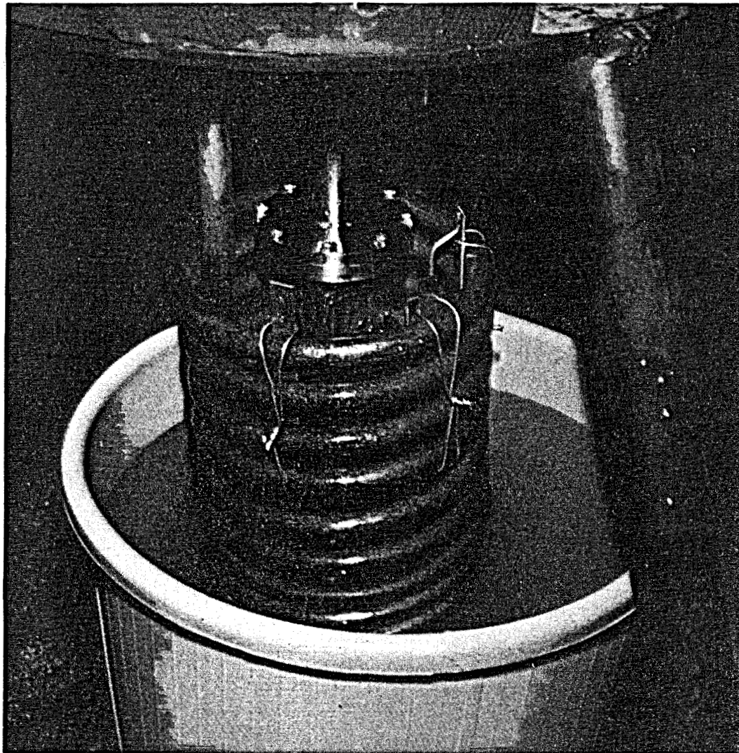
Figure 10.5. Close-up view of sensor and targets about to be immersed in water for preliminary base-line measurements.
