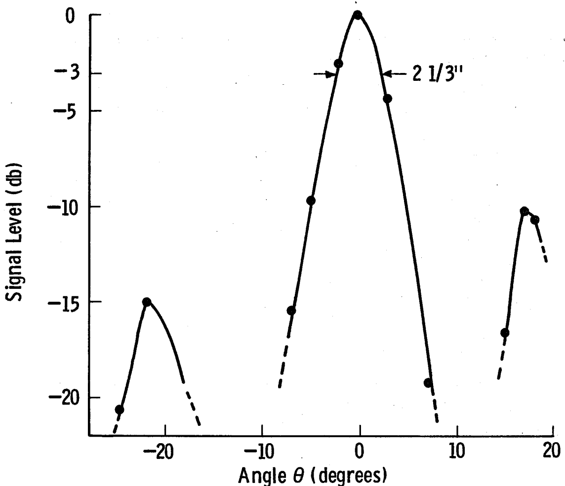
Figure 14. Transmit/receive beam pattern; 1-3/4" tool; 1.5" range.
