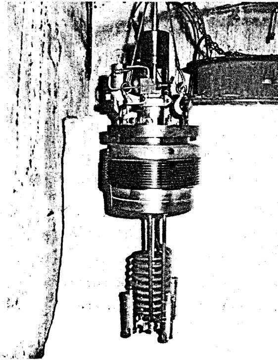
Fig. 2. Test Capsules Fastened to Autoclave Cooling Coil
