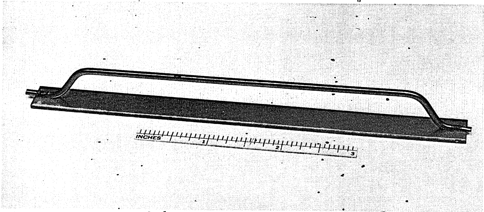
Figure 10.2. Typical acoustic target assembly designed for autoclave sensor evaluation testing. The stainless steel rod (target) is spot-welded to a stainless steel plate to provide for attachment to autoclave internals.
