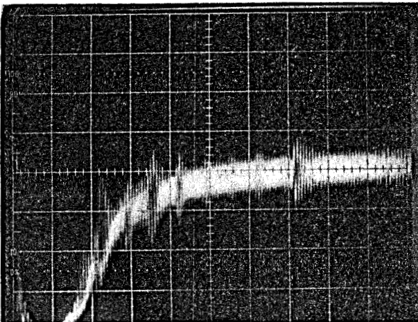
Figure 10.9. Echo pattern from 3/16" dia. rod in simulated geofluid. T = 350°F (275°C) P = 6500 pss. Horizontal = 10 \mu sec/div. Vertical = 0.5 Volt/div.
