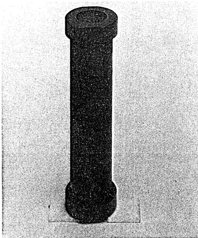
Fig. 20. Post-Test Photograph of Free-Flooding Test Capsule D, End Cap D1 Facing Upward
