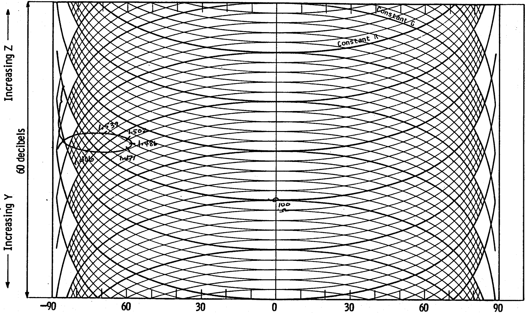
Fig. 11.18 Log Vector Impedance Plot (0.3 - 1.5 MHz) for autoclaved sensor, in air, at R.T.
