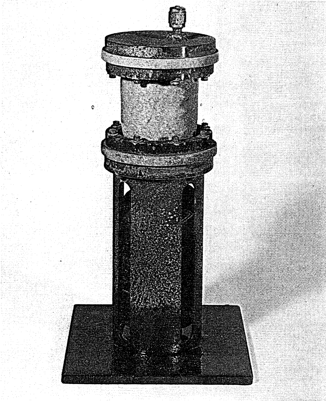
Figure 5.6 Photo showing the post-autoclave condition of the Ryton window. Note deformed bellows top and swollen window.
