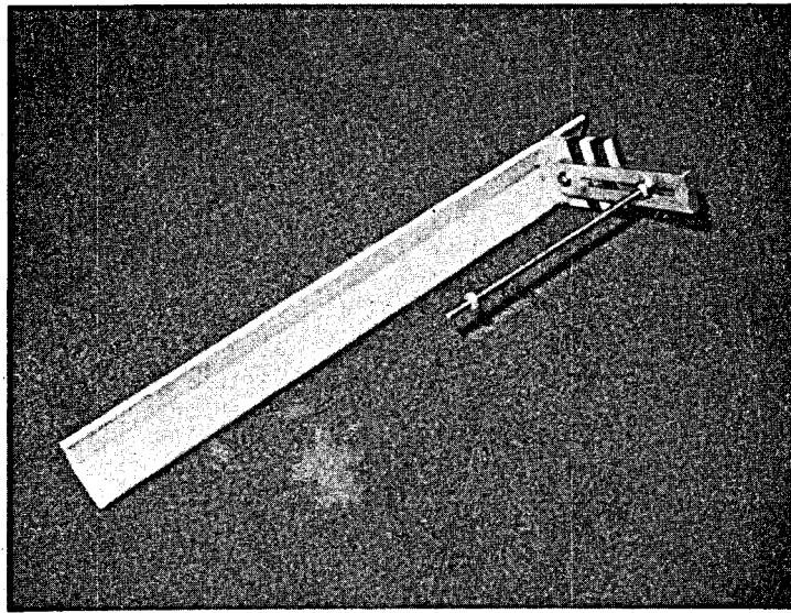
Figure 2. Scanning Fixture
