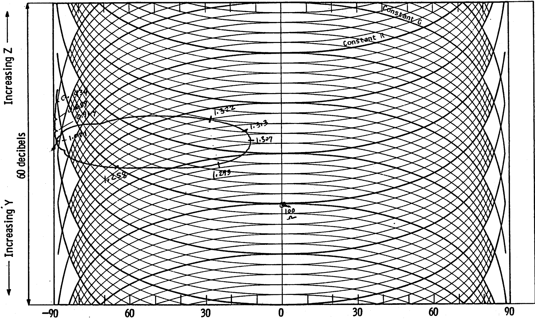
Fig.11.10 Log Vector Impedance plot for unmounted lead metaniobate disc (1/2" dia. x 1.3 MHz). Frequency Sweep Range: 0.3 MHz to 1.5 MHz.
