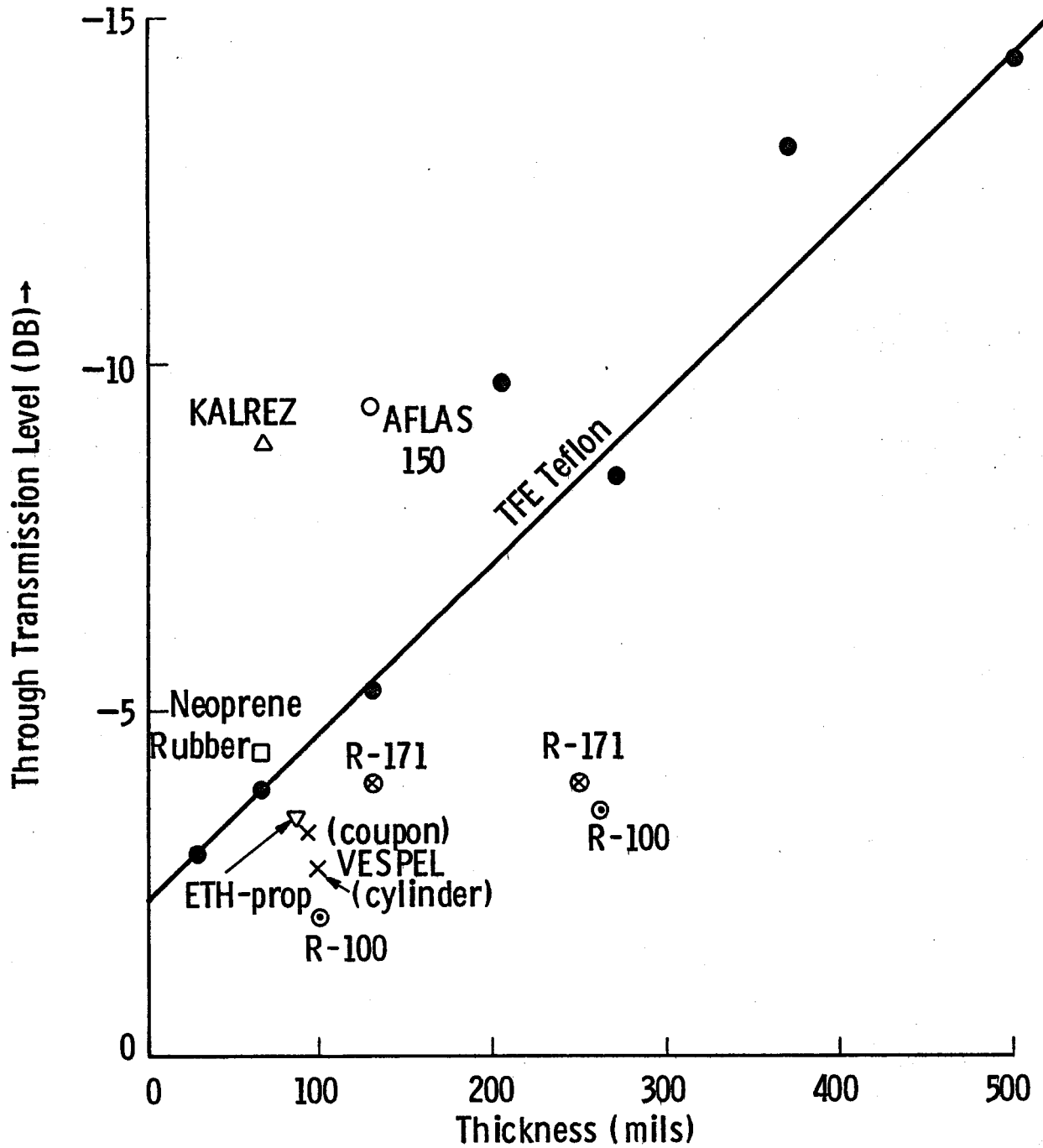
Figure 5.11 Data showing signal drop through certain window materials of various thicknesses. Solid line depicts drop through TFE Teflon. Measured with specimens immersed in transformer oil. Data generally indicates Ryton is low-loss, high temperature material.
