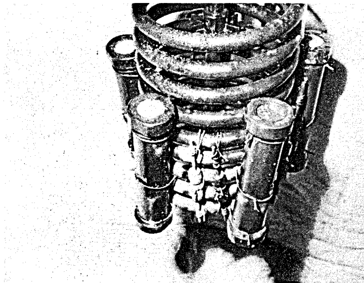
Fig. 13. Post-Test Photograph of Test Capsules Fastened to Autoclave Cooling Coil
