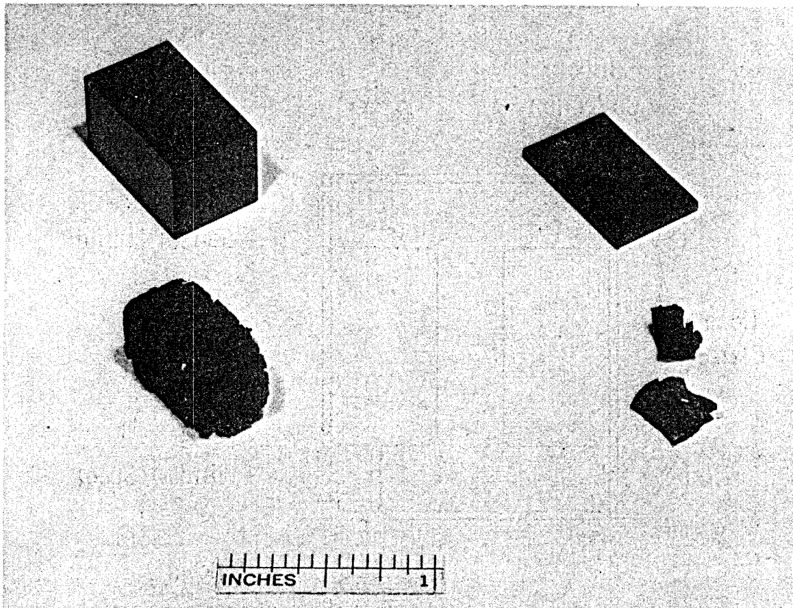
Figure 5.2 Photograph showing decomposition of Vespel after exposure to simulated geothermal conditions. Block and coupon control specimens (above) are compared with their autoclaved counterparts (below).
