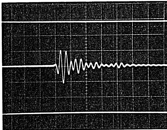
Figure 9. On-Axis Pressure Pulse; 3-3/8" Tool; With Teflon Tape. (H = 2 \mu sec/div; V = 0.2 Volts/div.)
