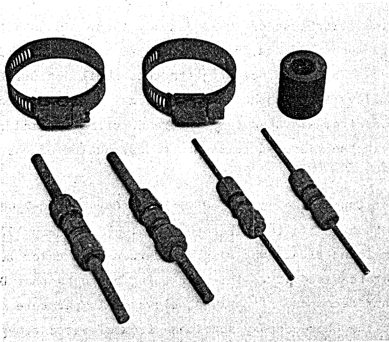
Fig. 22. Post-Test Photograph of Component Assortment Subjected to Direct-Exposure Testing Within Autoclave Liquid Environment
