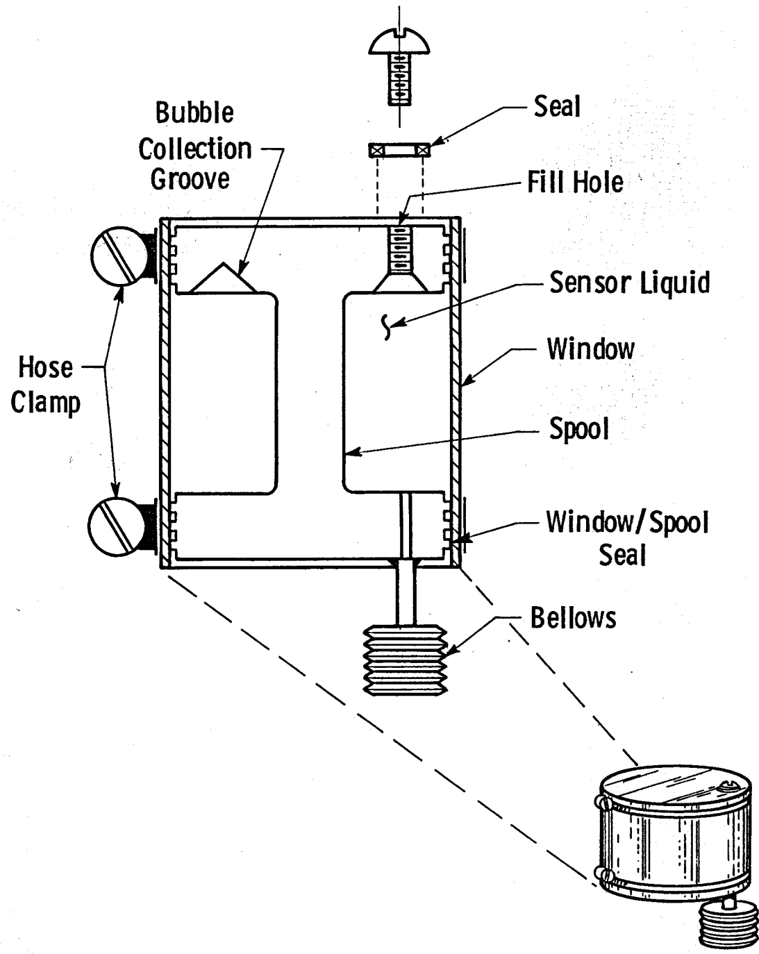
Figure 5.3 Diagram of improved capsule for advanced screening tests.
