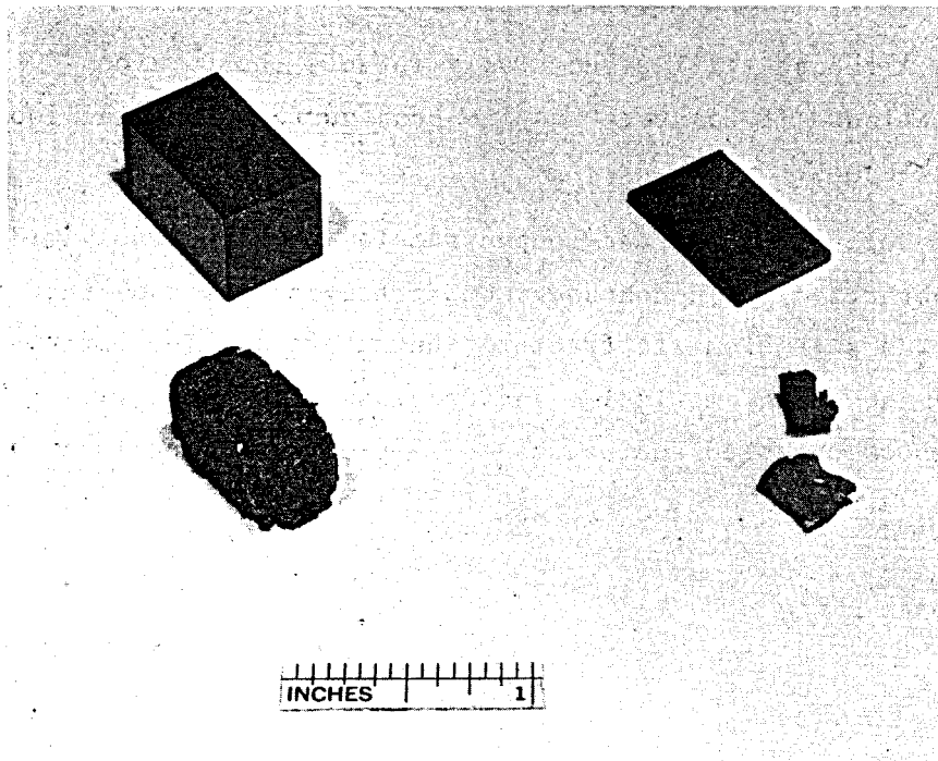
Figure 2.3 — Top: Untested (control) block and coupon samples of Vespel. Bottom: Vespel block and coupon samples after autoclave testing.
