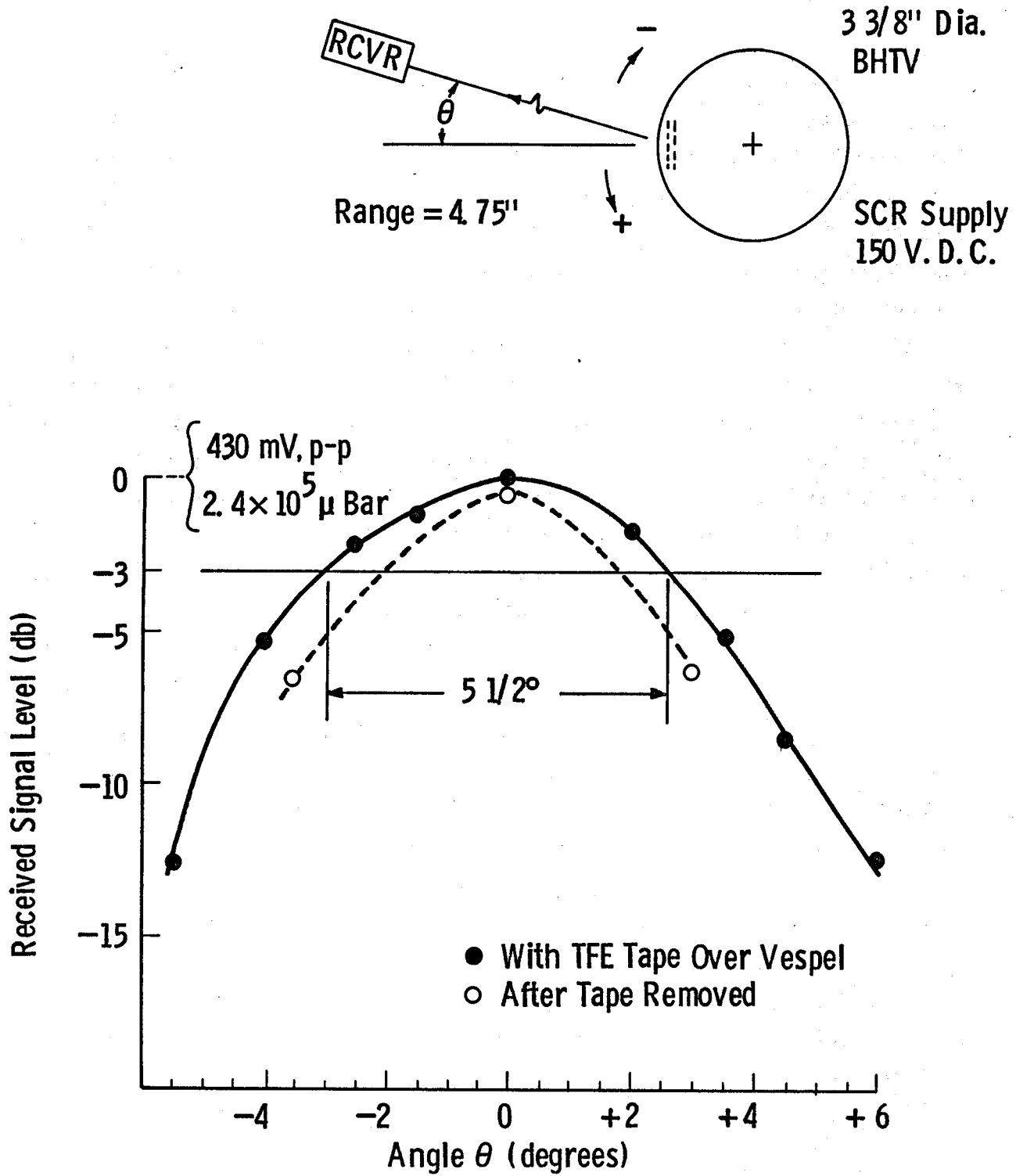
Figure 8. Transmit beam pattern; 3-3/8" tool; 4.75" range, with and without Teflon tape over Vespel window.
