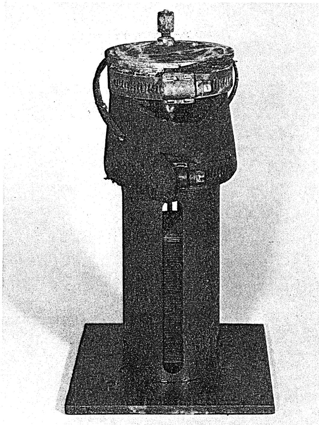
Figure 5.5 Photo showing the post-autoclave condition of the Kalrez window.
