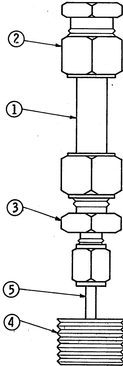
Figure 6.1 Diagram of advanced fluid screening test capsule design.
