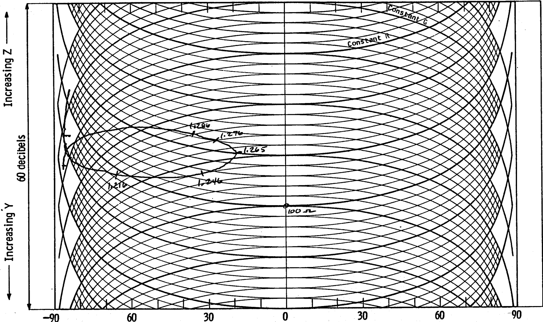
Fig. 11.14 Log Vector Impedance Plot (0.3 - 1.5 MHz) for "spare" transducer assembly of Fig. 5. Temperature = 401°F.
