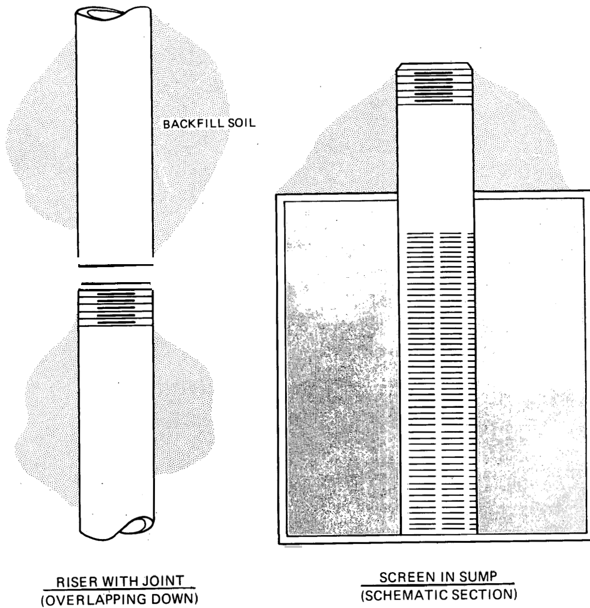
Figure 2.6.1. Features of sump monitoring wells
