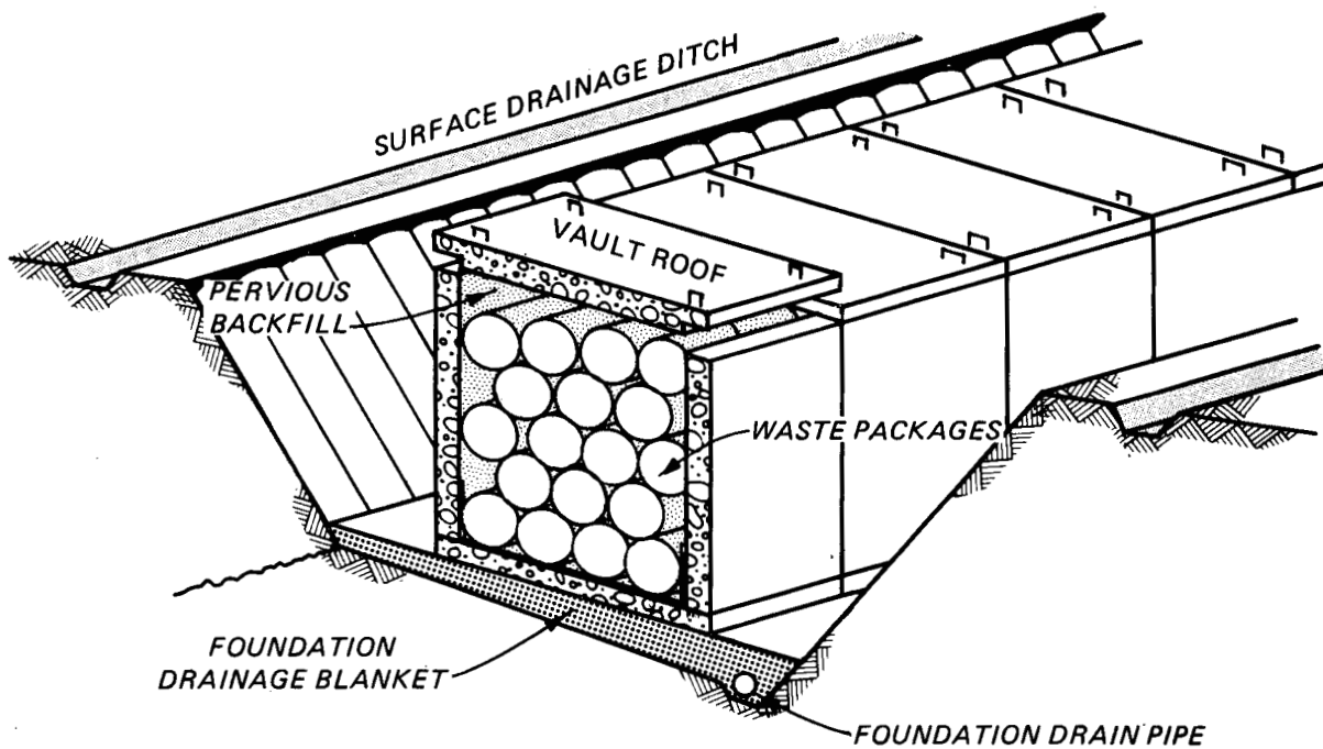
Figure 2.4.3. Top loading concept of waste emplacement in an EMCB
