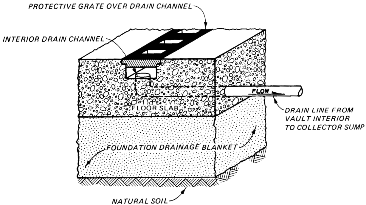
(b) Section view detail of interior collector system
