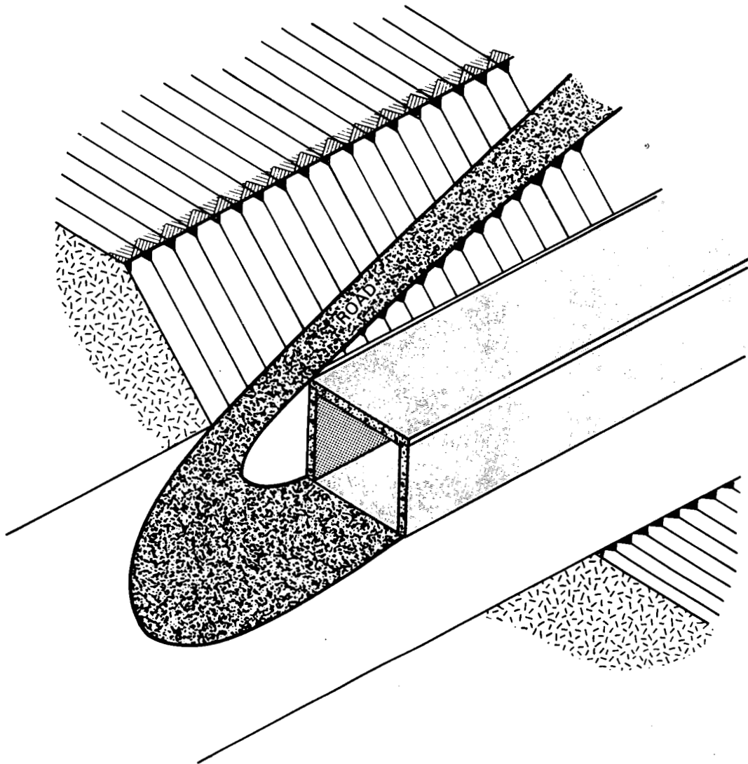
Figure 2.4.2. Side loading concept of waste emplacement in an EMCB
