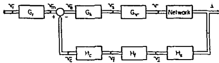
Figure 2. A block diagram of the closed loop current control system.
