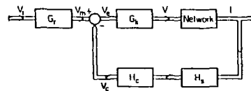
Figure 3. A block diagram of the closed loop system for the dc steady state. This diagram also represents the simplified system.
