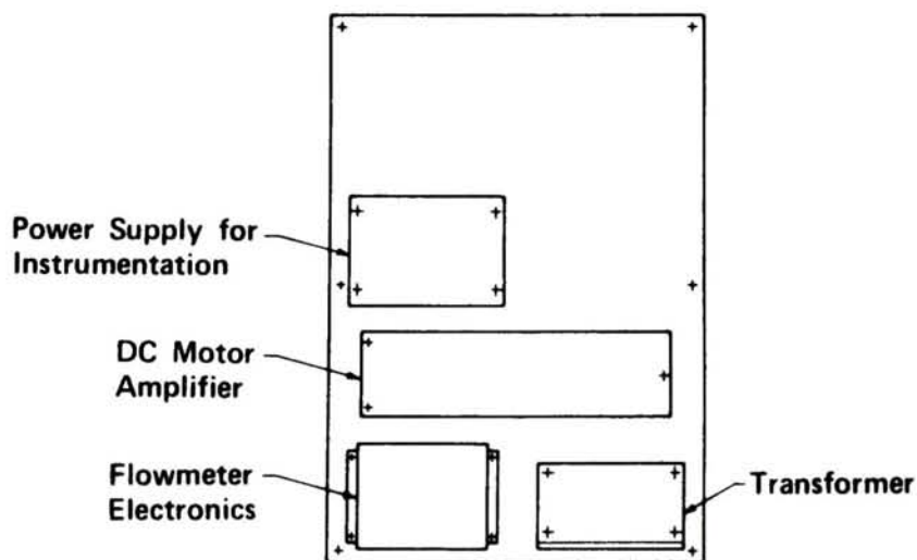
INTERNAL CONTROL PANEL LAYOUT
