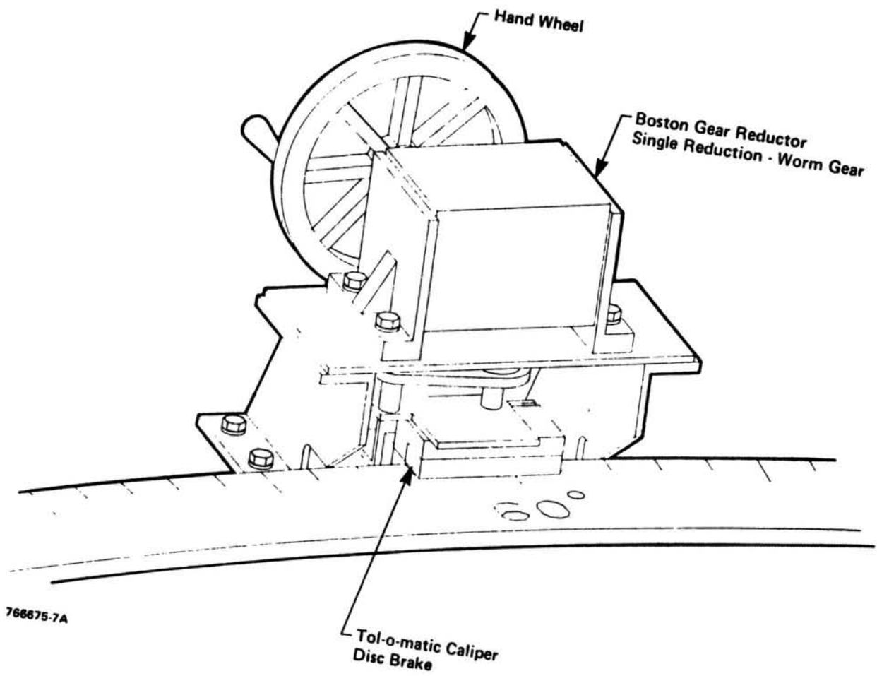
Figure 7. Manual brake.
