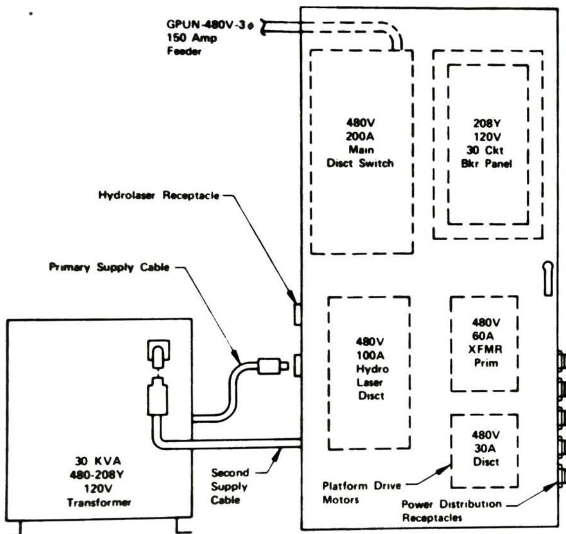
Figure 35. Electrical power distribution.
