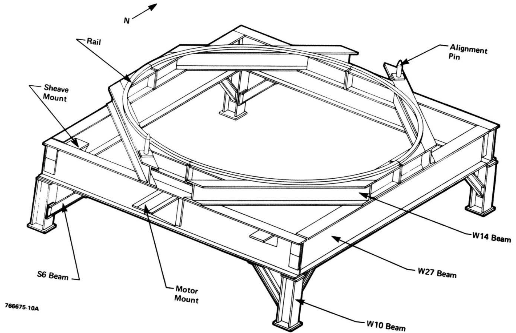
Figure 10. Main structure.
