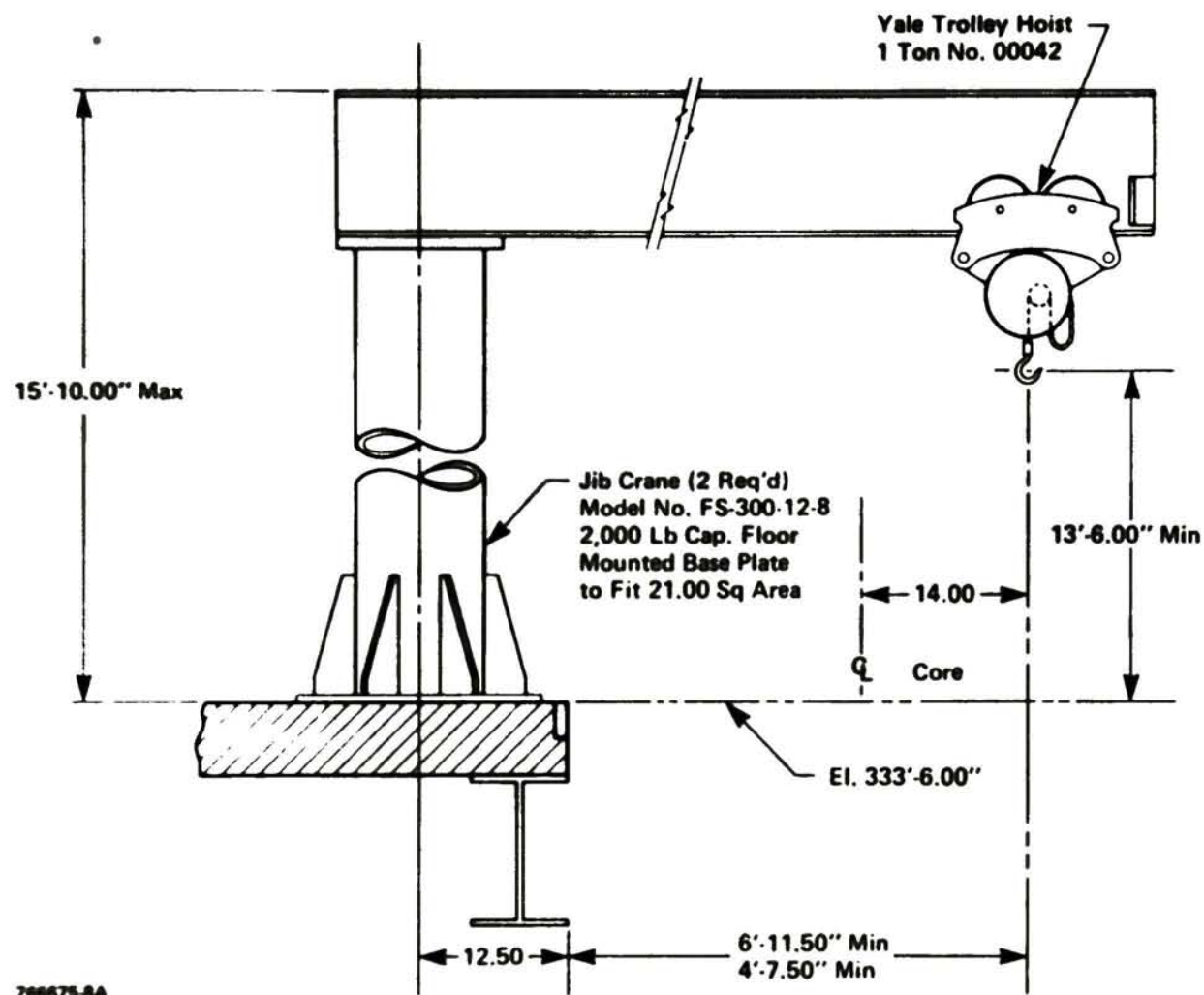
Figure 8. Jib crane.
