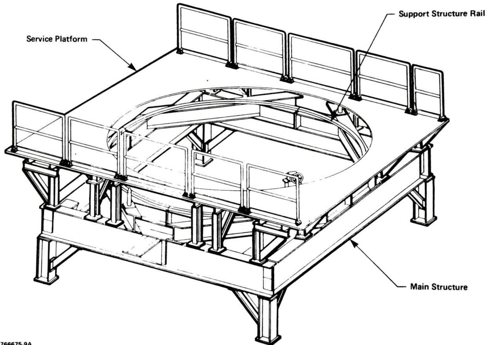
Figure 9. Shielded support structure.
