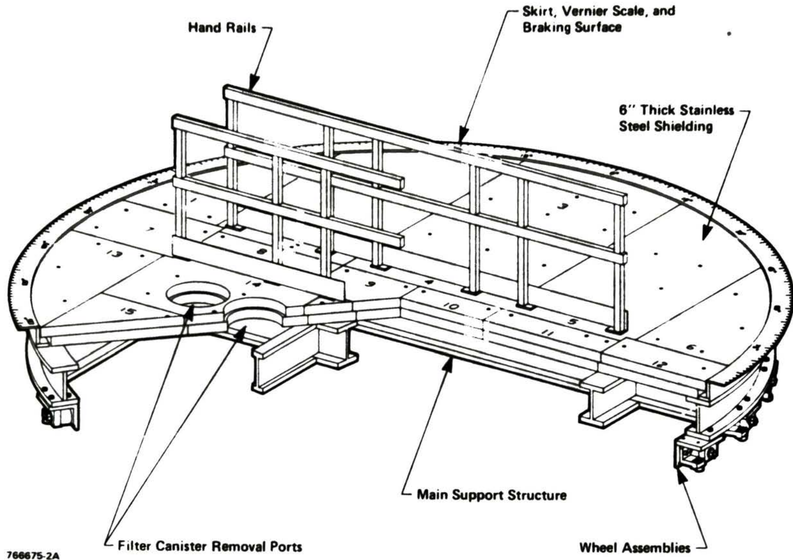
Figure 2. Shielded work platform.
