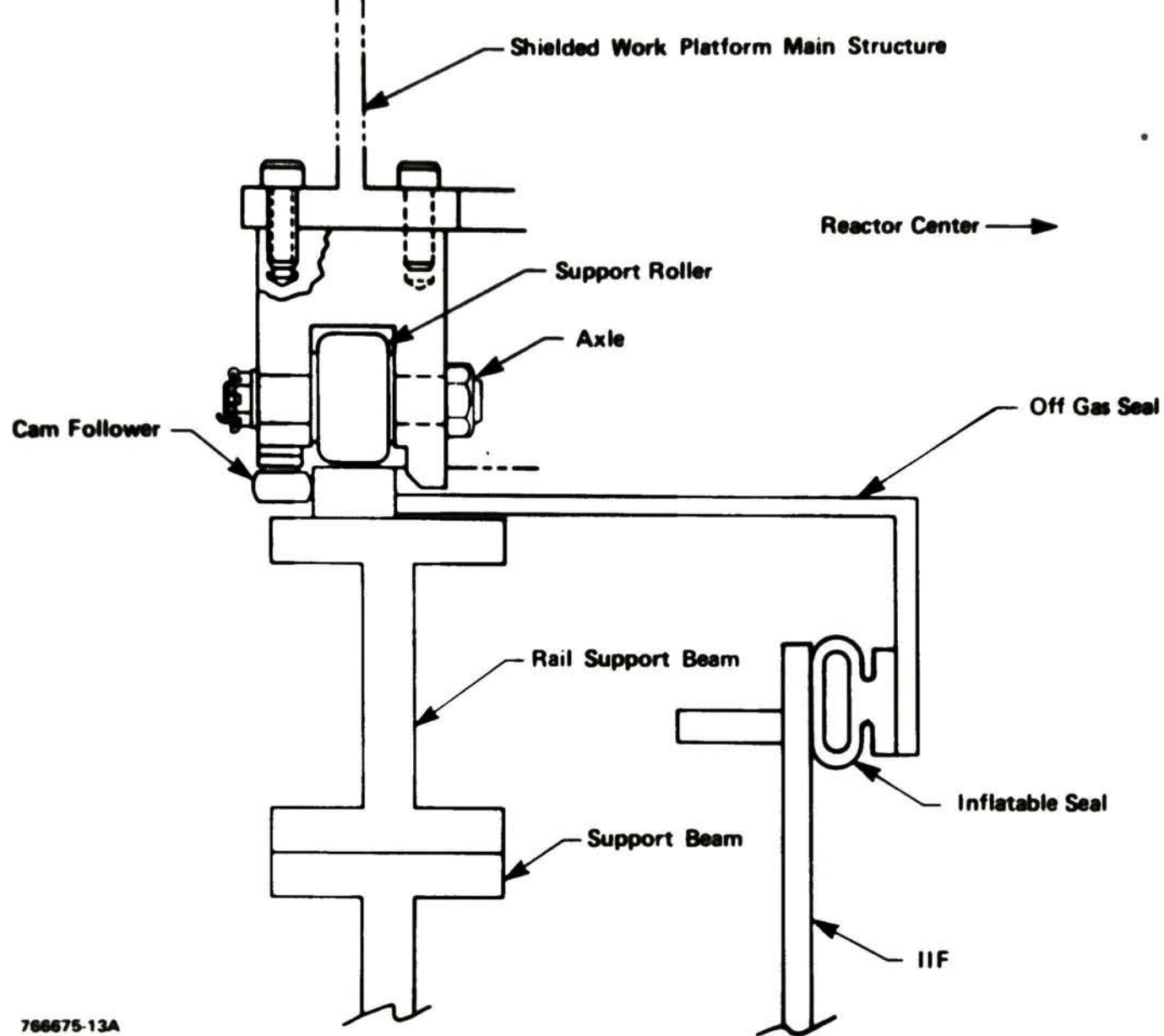
Figure 13. Off-gas seal cross-section.
