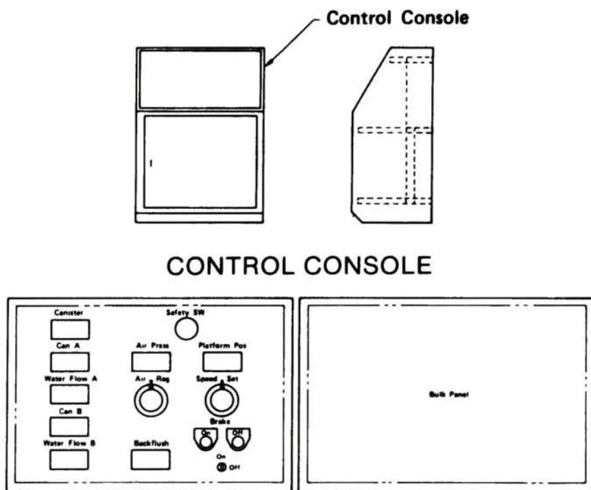
CONTROL CONSOLE PANEL LAYOUT
