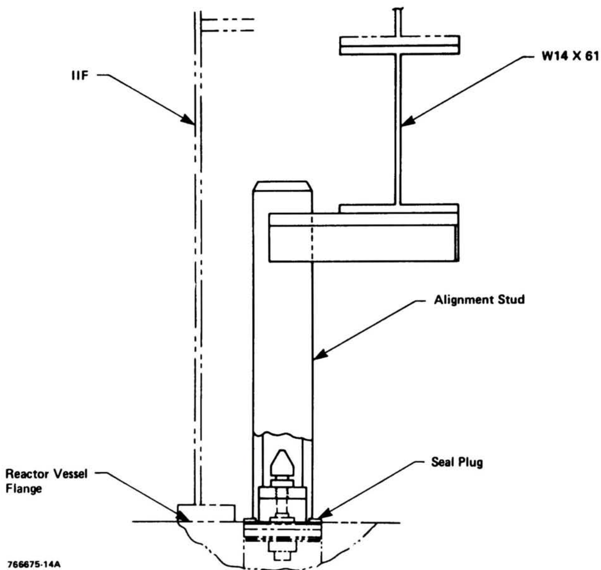
Figure 14. Alignment stud.
