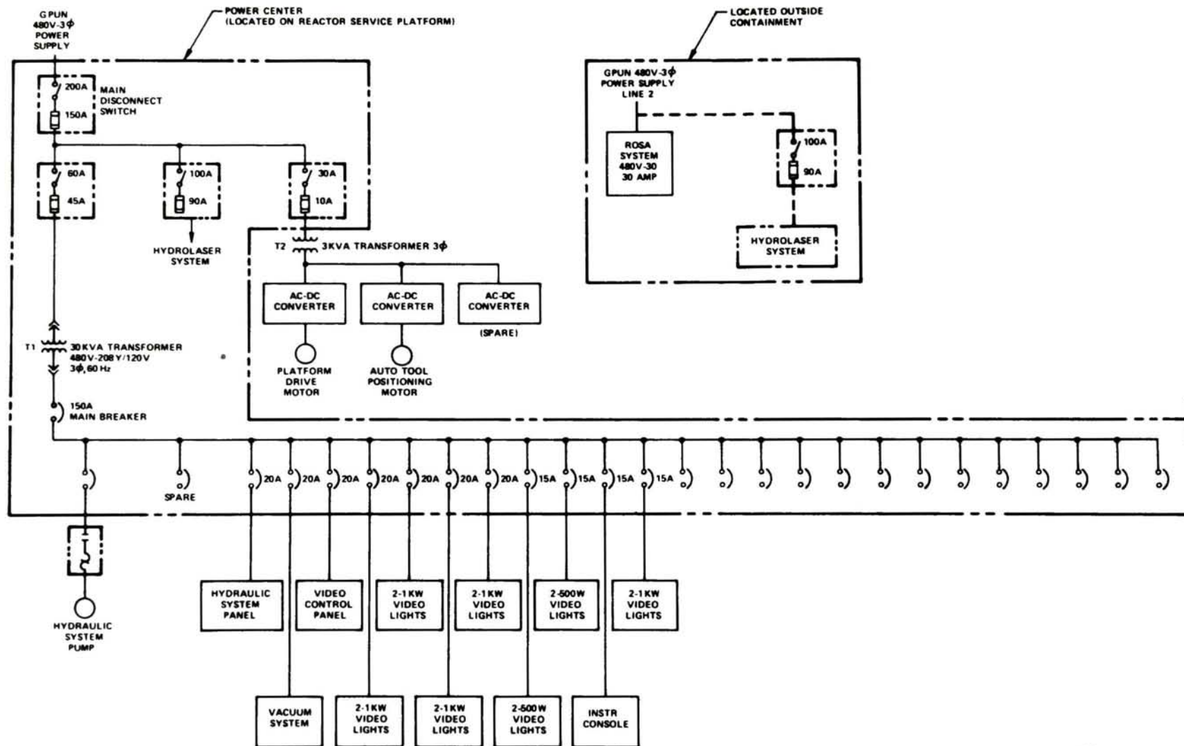
Figure 34. Single line diagram - electrical power distribution.
