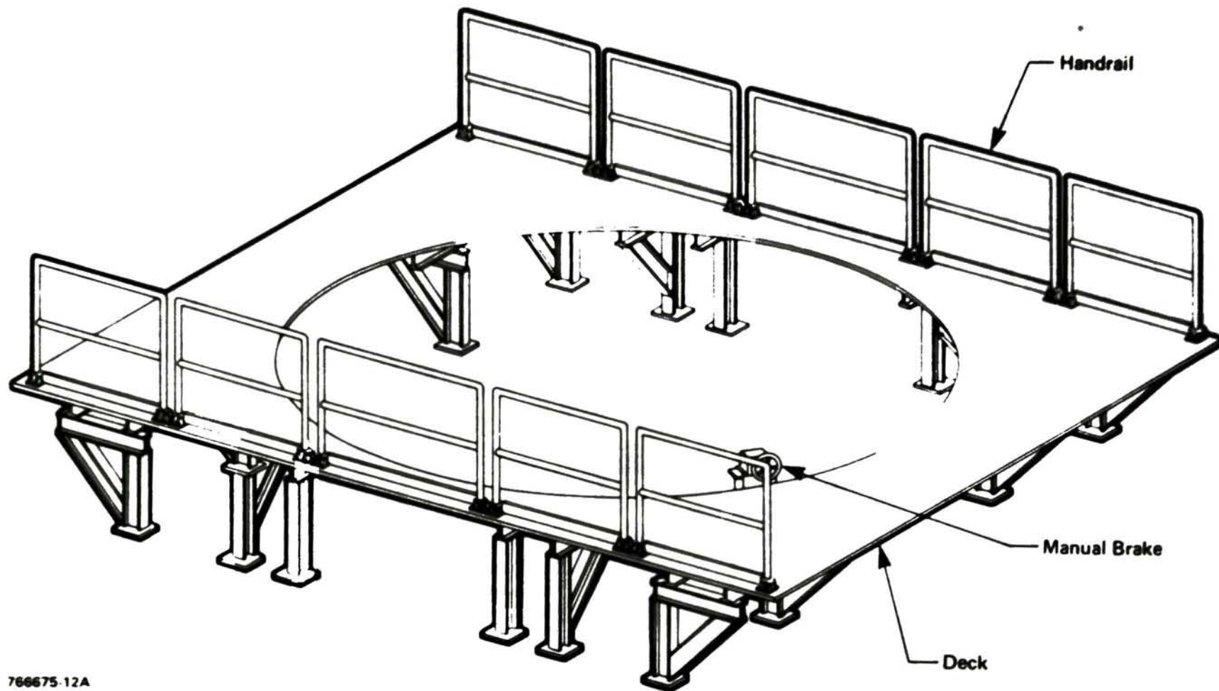
Figure 12. Service platform.
