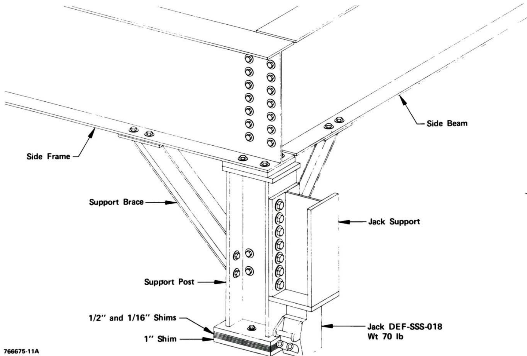
Figure 11. Leveling jack.
