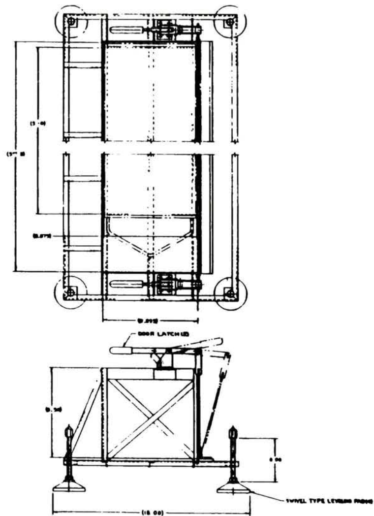
Strongback for Side Loading Debris Bucket
