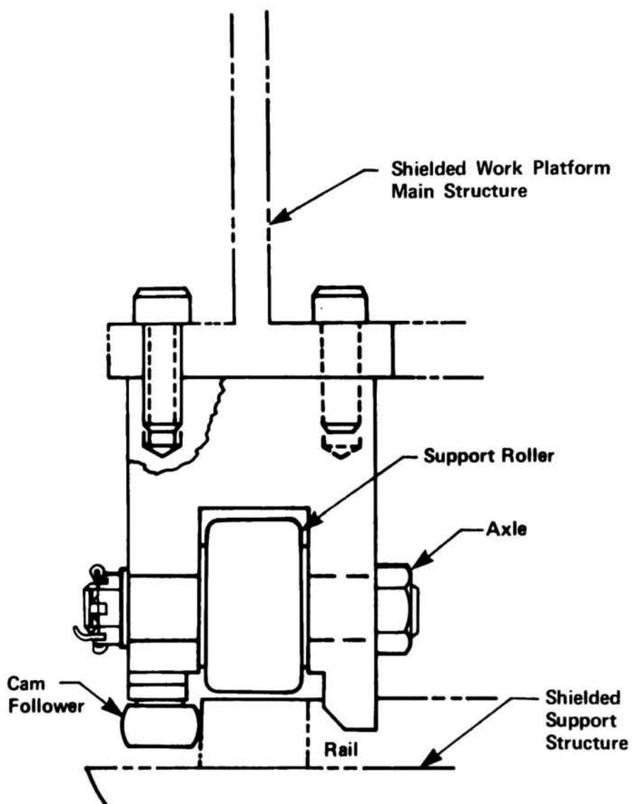
Figure 4. Roller assembly.
