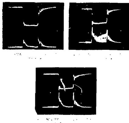
Fig. 3. Forward (top) and reflected (bottom) rf wave shapes under various input conditions.
