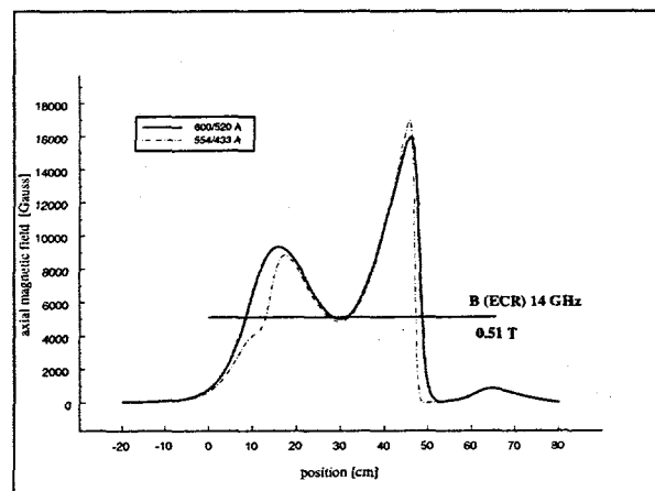
Fig. 2: Axial field distribution with different iron yoke configurations
