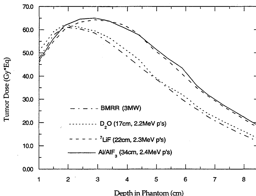
Fig. 2: Depth distributions of total equivalent tumor doses for \text{D}_2\text{O} , ^7\text{LiF} and \text{Al/AlF}_3 moderated neutron beams from a ^7\text{Li(p,n)} source and the BMRR beam.
