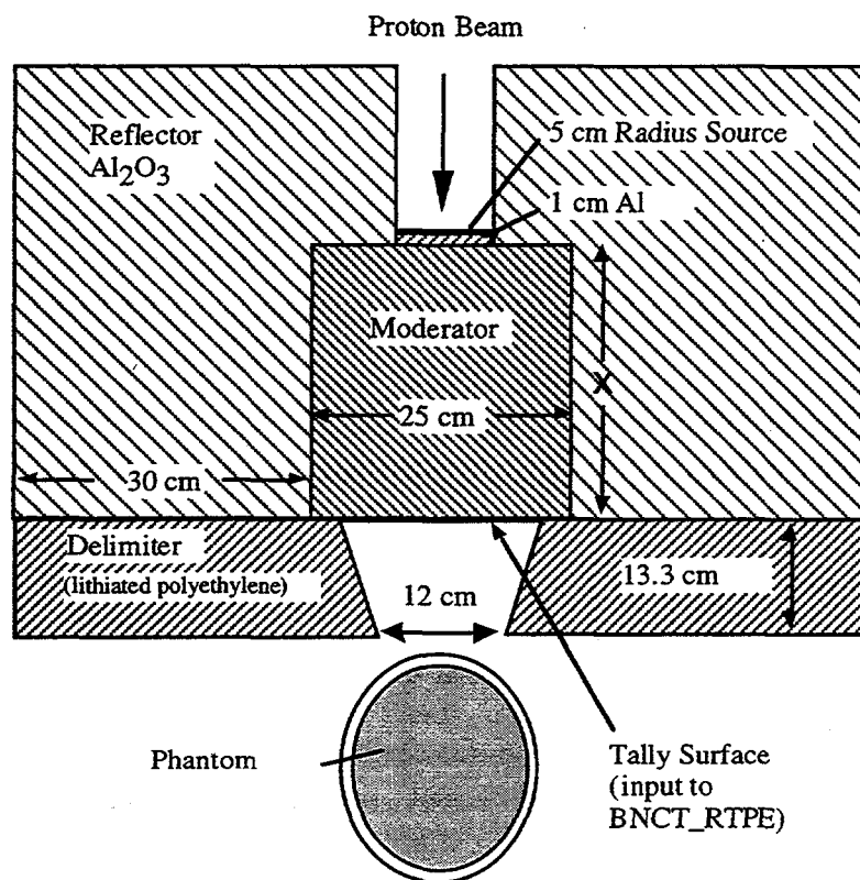
Fig. 1 Cross section of moderator and filter assembly.
