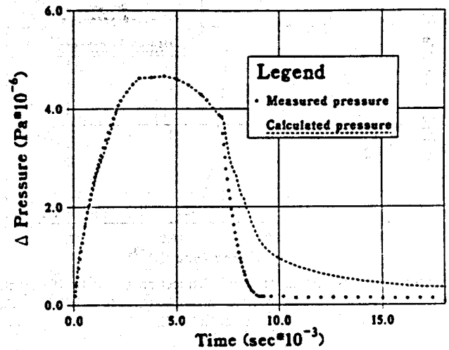
Figure 12. One possible match of the A-7 injection test data. Note the good match of the buildup data and the poor match of the falloff data. Parameters for this match are k_r h/\mu_i = 2.8 \times 10^{-9} m 3 /Pa*s, \phi c_i h = 2 \times 10^{-8} m/Pa, and s = -2 .
