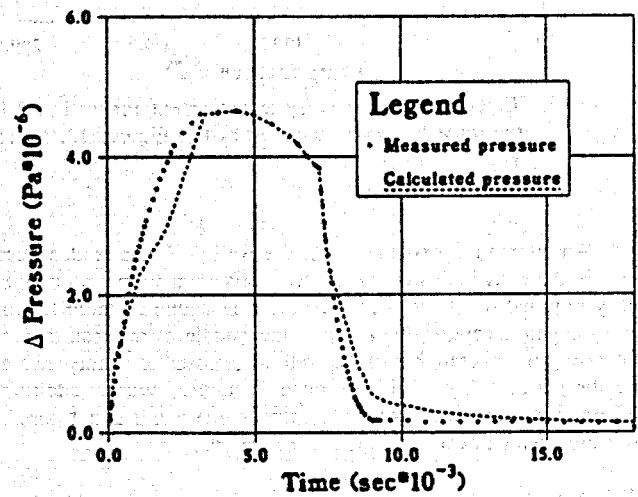
Figure 13. One possible match of the A-7 injection test data. Note the poor match of the buildup data and the better match of the falloff data. Parameters for this match are k_r h/\mu_i = 7.0 \times 10^{-9} m 3 /Pa*s, \phi c_i h = 2 \times 10^{-9} m/Pa, and s = 0 .
