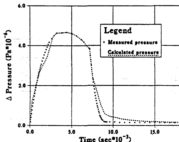
Figure 14. Best match of the A-7 injection test data. Parameters for this match are k_f h / \mu_i = 6.5 \times 10^{-9} \text{ m}^3/\text{Pa}\cdot\text{s} , \phi C_f h = 7 \times 10^{-10} \text{ m}^3/\text{Pa} , and s=0 .
