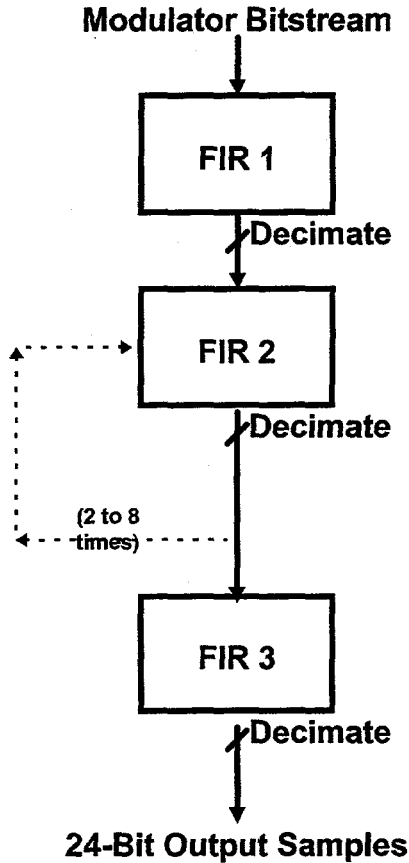
Figure 1 – CS5322 FIR Digital Filter Ensemble
