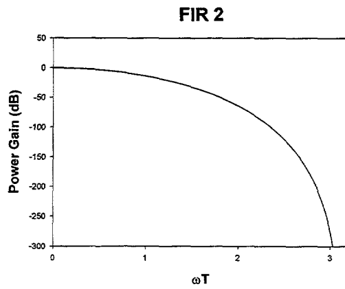
Figure 3 - Stage 2 Transfer Function
