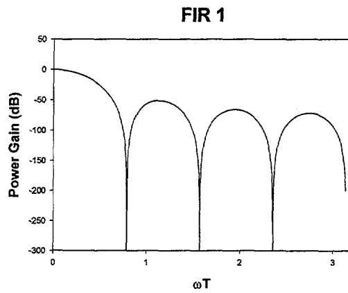
Figure 2 - Stage 1 Transfer Function
