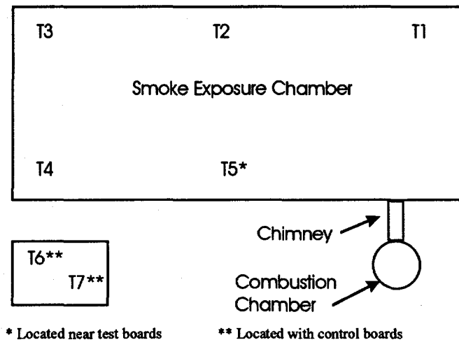
Figure 12. Thermocouple locations.
