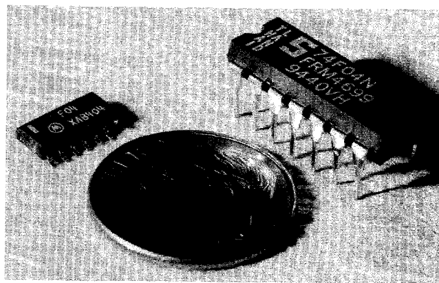
Figure 4. Comparison of PTH and SMT packages for the same device.
