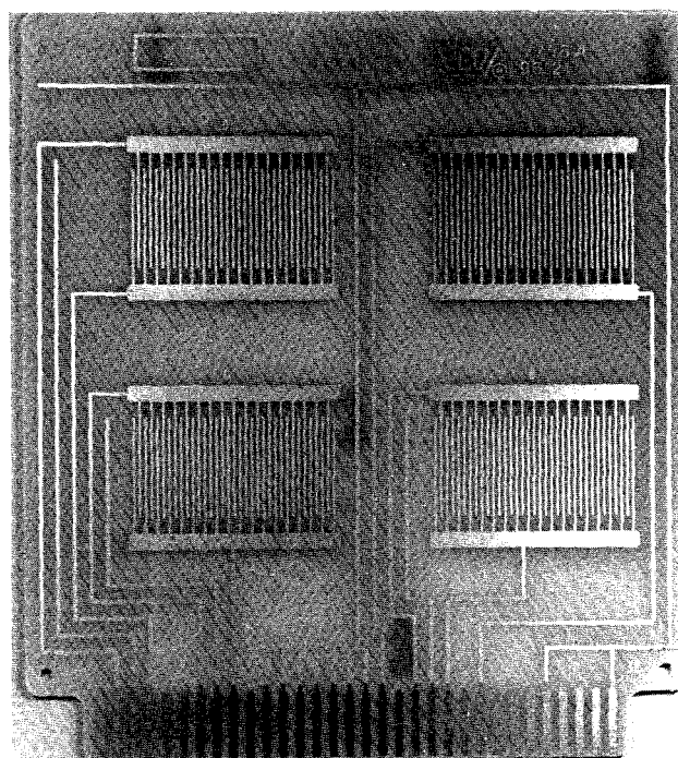
Figure 26. IPC-B-24 board for surface insulation resistance.
