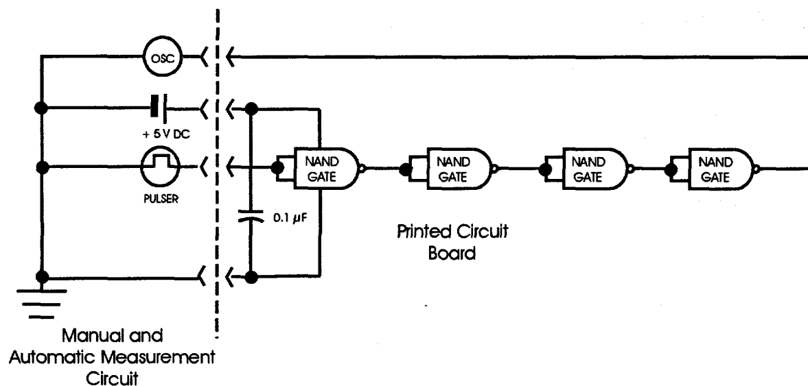
Figure 17. HSD SMT measurement circuit.
