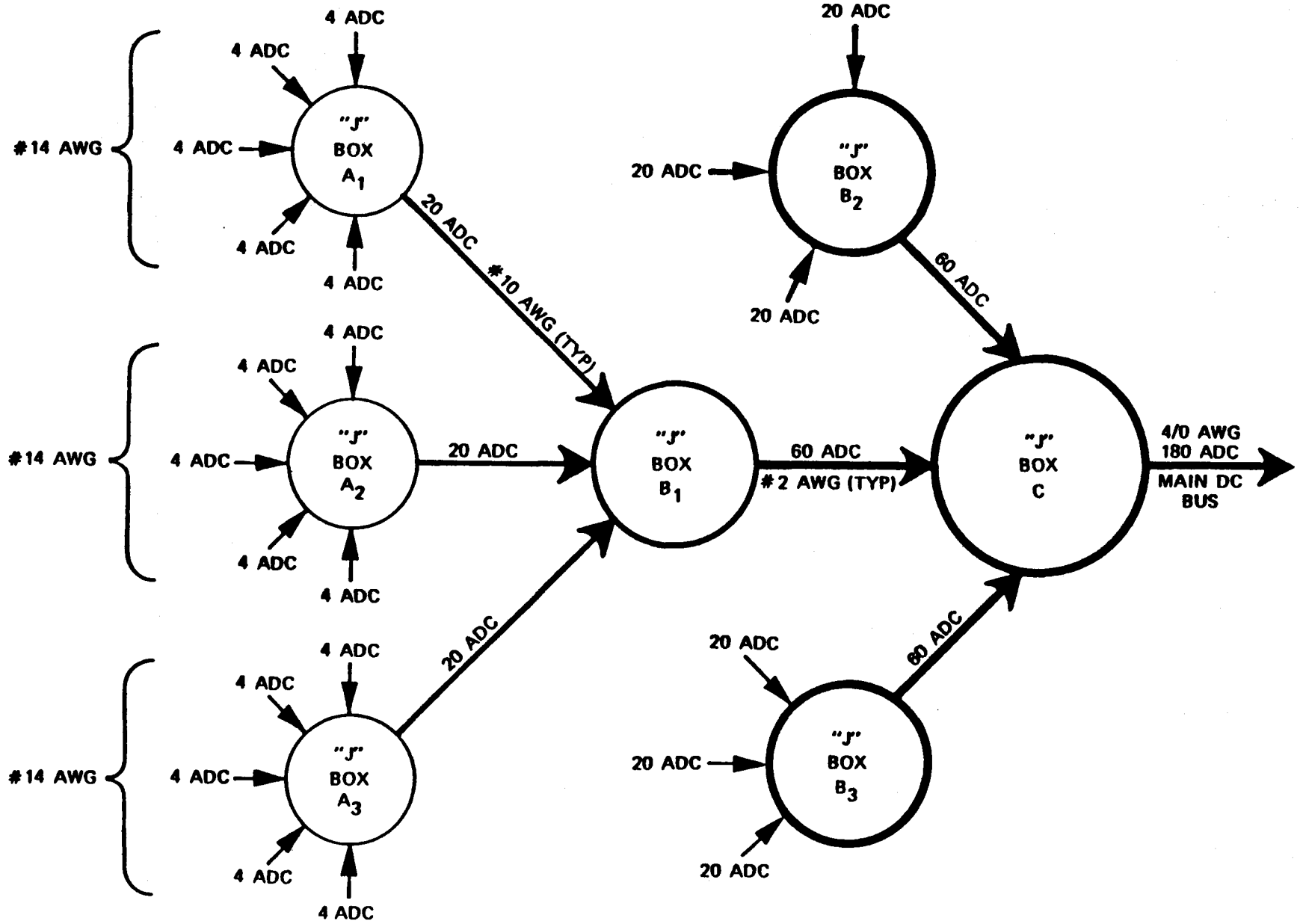
Figure 3.4-7 ARRAY FIELD WIRING: TAPERED AMPACITY BUS.
