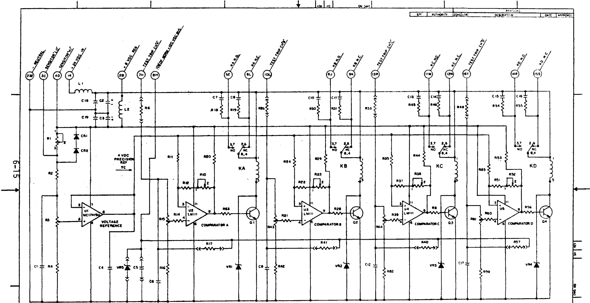
CHARGE/REGULATOR CONFIGURATION - 02 FIGURE 6.4-8. SCHEMATIC OF UNIVERSAL CONTROL PRINTED CIRCUIT BOARD
