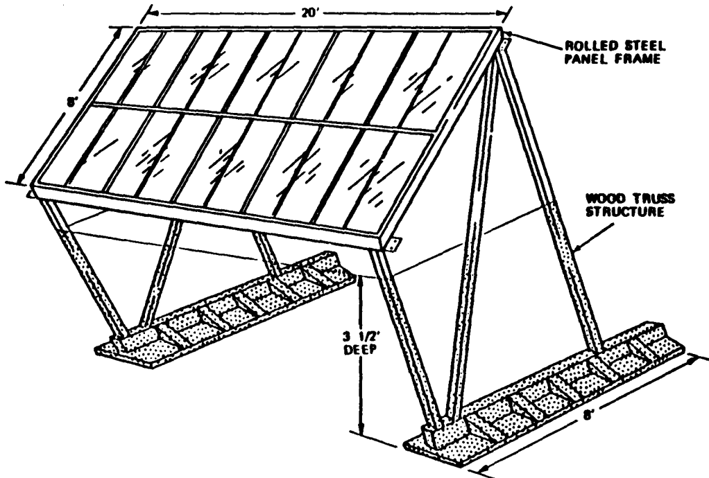
JPL Low Cost Structure/Foundation Concept FIGURE 3.3-1
