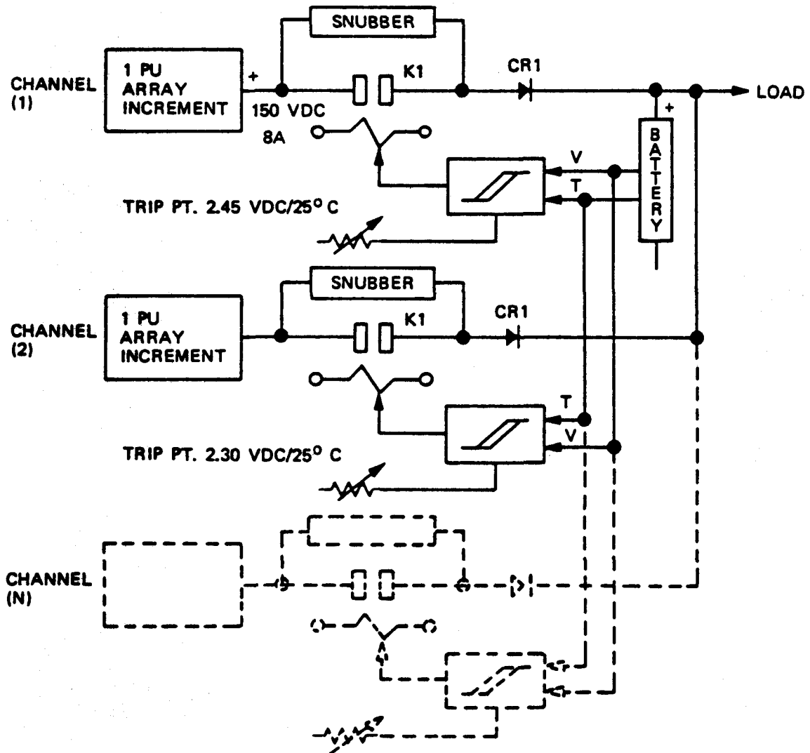
FIGURE 3.5-8 BATTERY CHARGER REGULATOR MULTI-LEVEL SERIES (OFF-ON)
