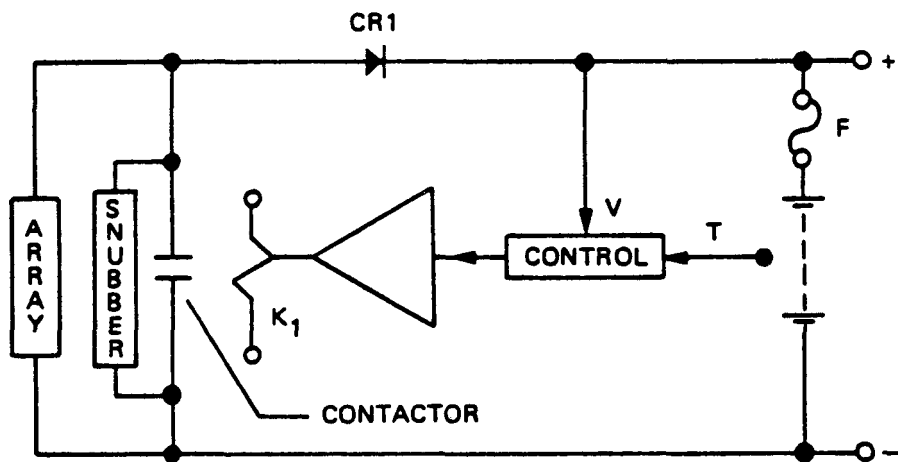
FIGURE 3.5-2 ON-OFF SHUNT CONTACTOR CONTROL
