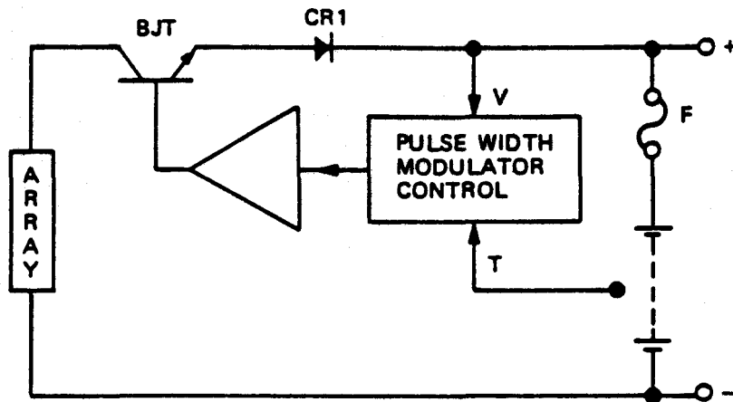
FIGURE 3.5-7 PULSE WIDTH MODULATOR SERIES CONTROL
