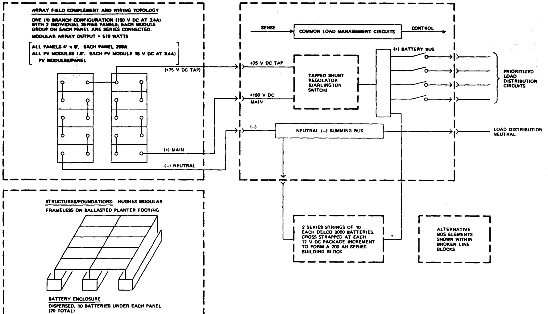
Figure 4.10-8 - Design concept VII 1/2 PU baseline PV system.
