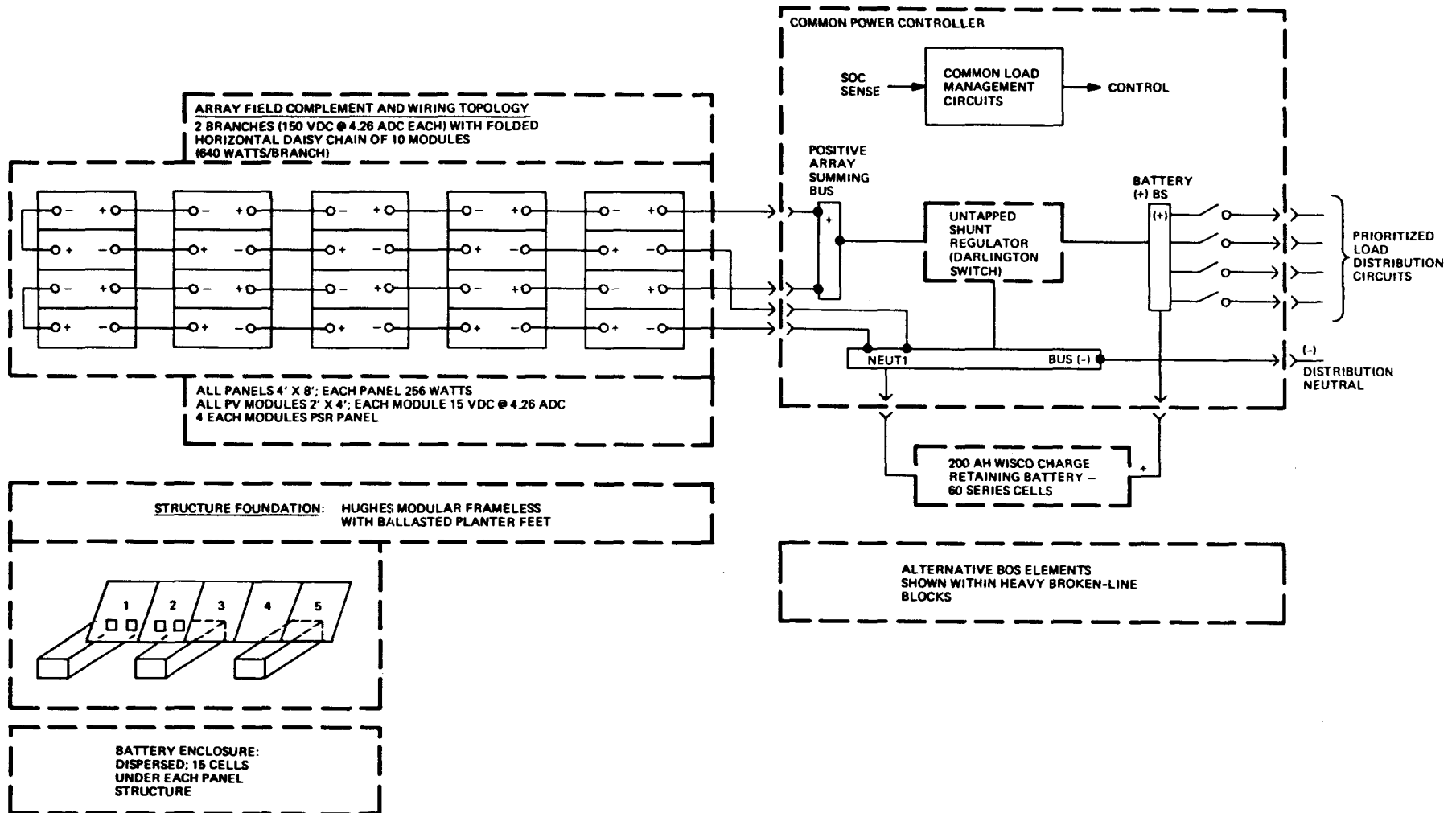
Figure 4.10-2 - Design concept I baseline IPU PV system.
