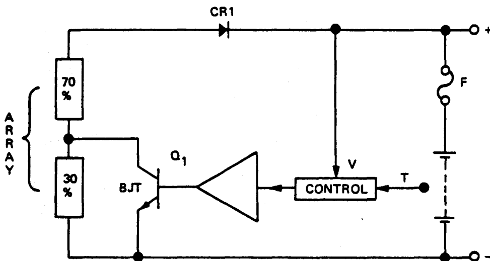
FIGURE 3.5-4 ON-OFF SHUNT BJT CONTROL (TAPPED)
