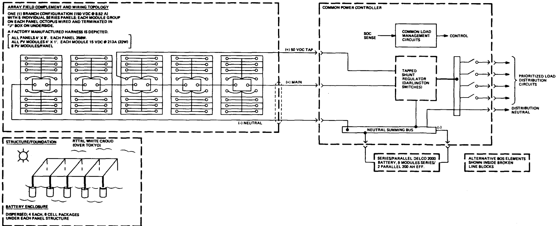
Figure 4.10-5 - Design concept IV baseline IPU PV system.
