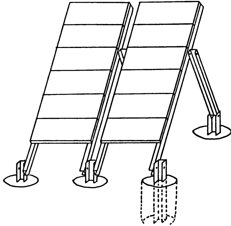
Post Hold Concrete Pier Structure/Foundation FIGURE 3.3-3
