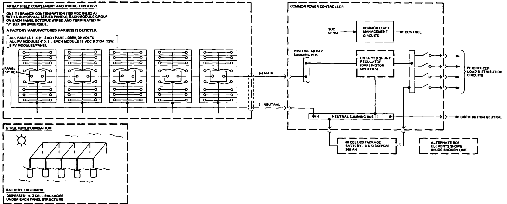
Figure 4. 10-4 - Design concept III baseline IPUS.
