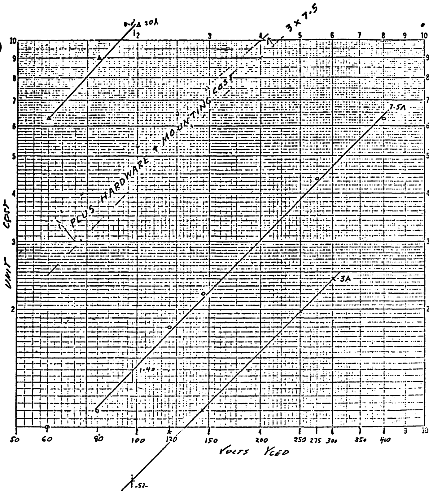
FIGURE IV-9. TRANSISTOR COST-VS-RATING
