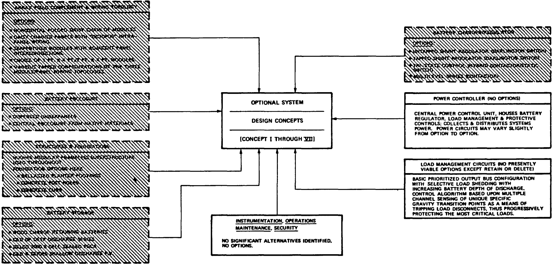
SELECTED BOS OPTIONS AND ALTERNATIVES FOR CONCEPTUAL DESIGN OF BASELINE I.P.W. P.V. SYSTEM.
