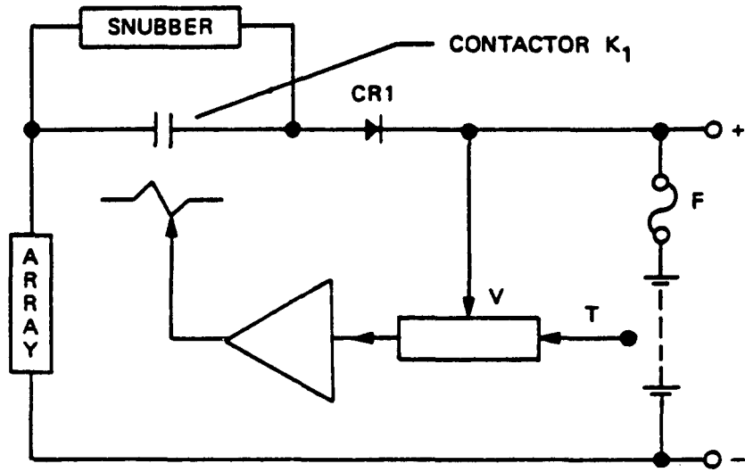
FIGURE 3.5-5 ON-OFF SERIES CONTACTOR CONTROL
