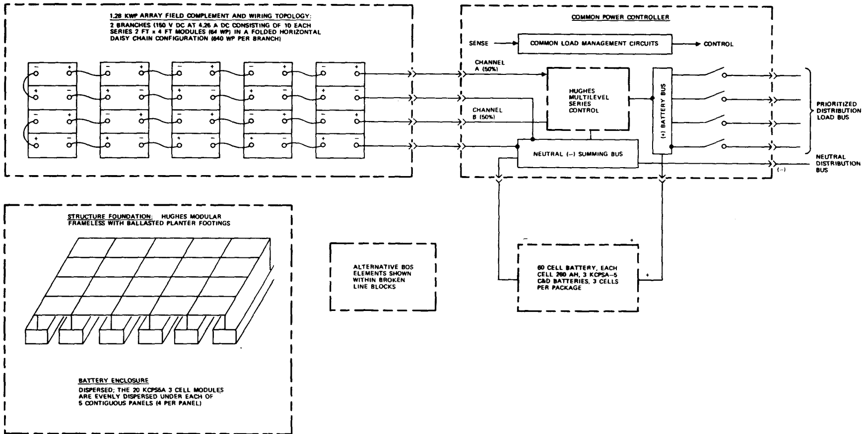
Figure 4. 10-7 - Design concept VI baseline 1 PU PV system.
