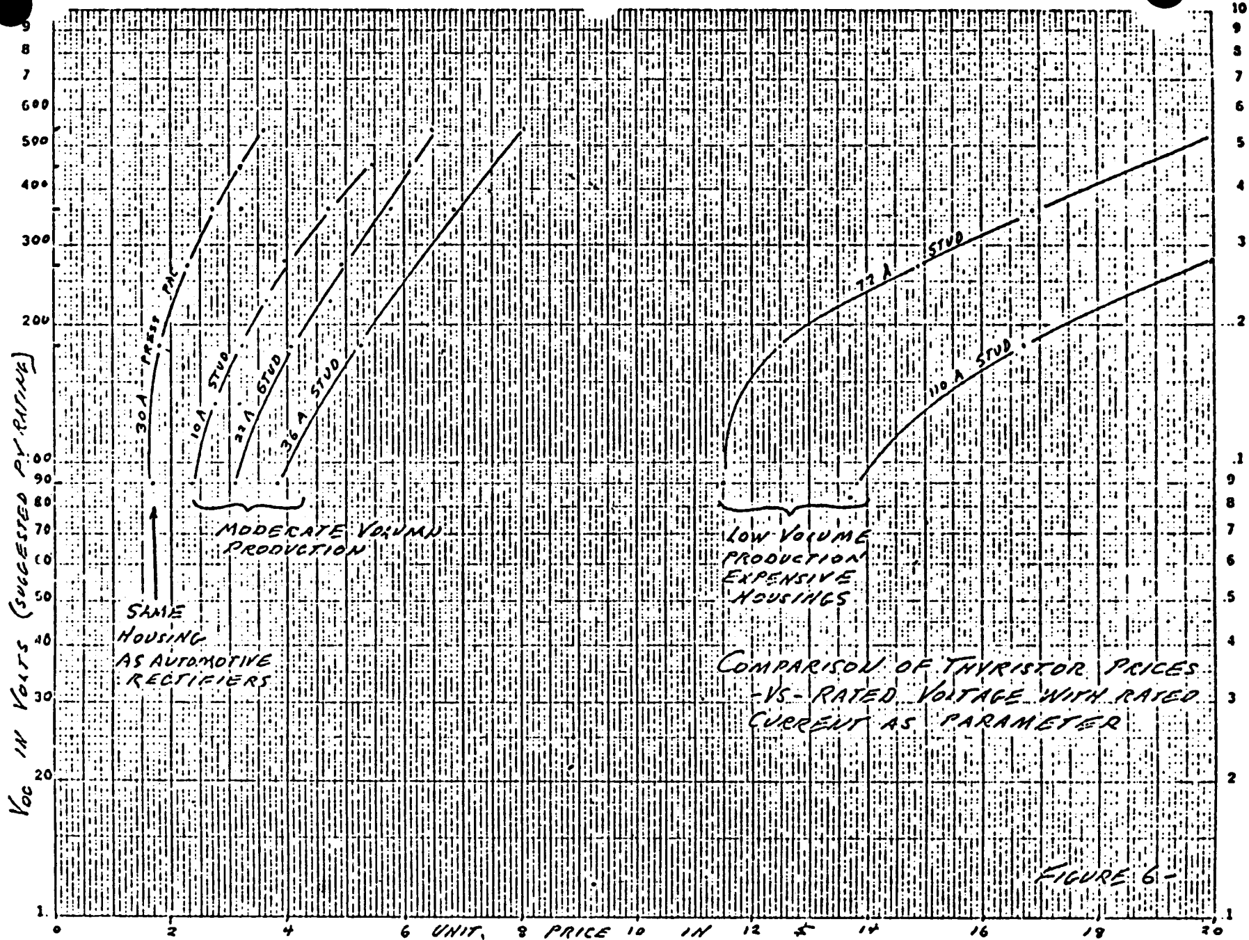
FIGURE IV-8. COMPARISON OF THYRISTOR PRICES-VS-RATED VOLTAGE WITH RATED CURRENT AS PARAMETER
