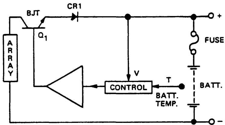
FIGURE 3.5-1 SERIES LINEAR BJT CONTROL
