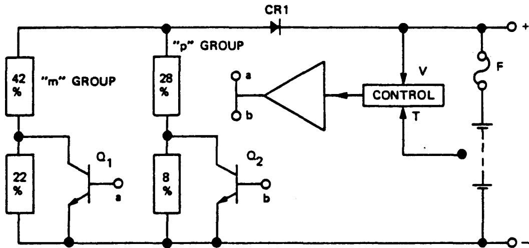
FIGURE 3.5-6 TRI-STATE CONTROL
