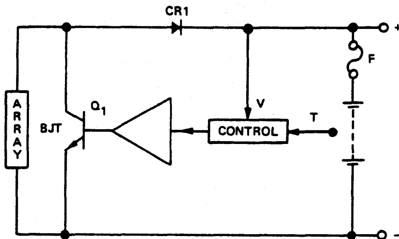
FIGURE 3.5-3 ON-OFF SHUNT BJT CONTROL
