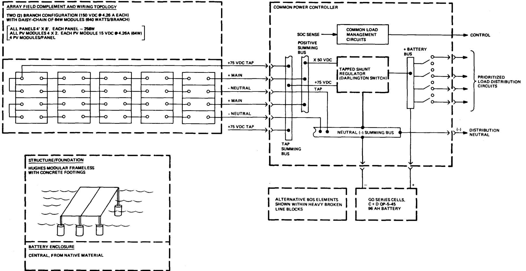
Figure 4, 10-3 - Design concept II baseline IPU PV system.
