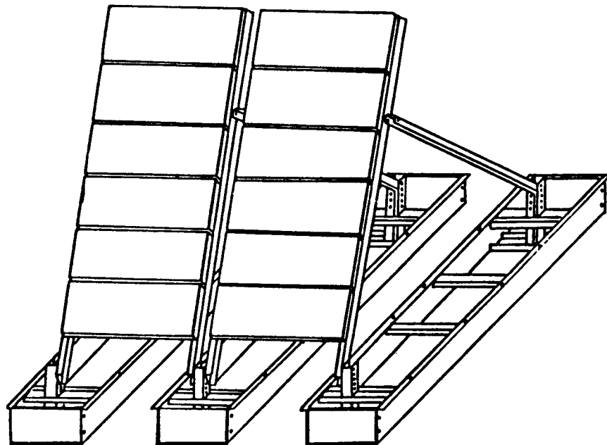
Ballasted Planter Structure/Foundation FIGURE 3.3-4
