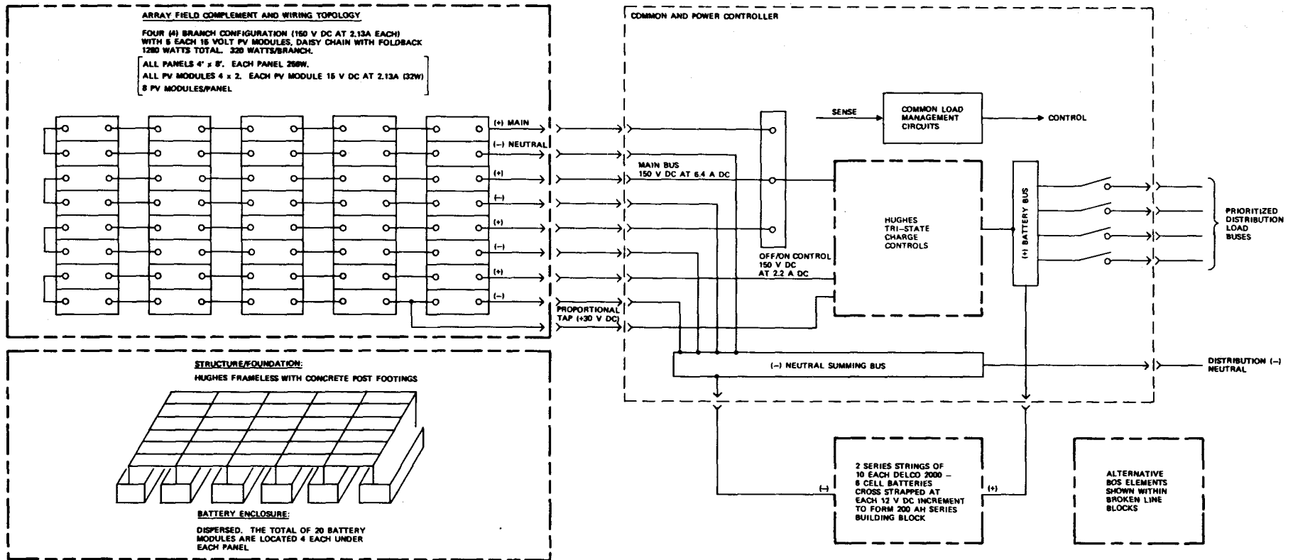
Figure 4.10-6 - Design concept V baseline 1 PU PV system.
