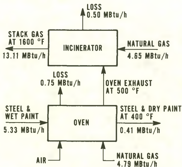
FIGURE 4. Conventional paint drying oven and fume incinerator.
