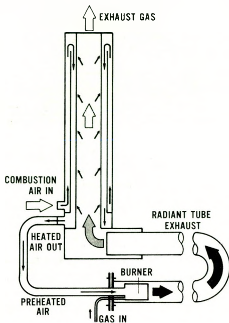
FIGURE 9. Diagram of a small radiation-type recuperator fitted to a radiant tube burner.
