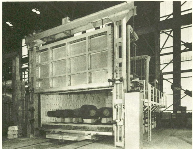
FIGURE 17. A car bottom furnace with ceramic fiber insulation. Courtesy of Olson Industries Corporation.
