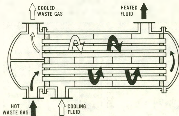
FIGURE 8. Diagram of convective-type recuperator.
