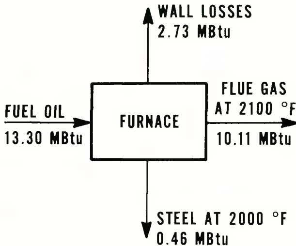
FIGURE 1. Batch fired furnace (first heat balance).
