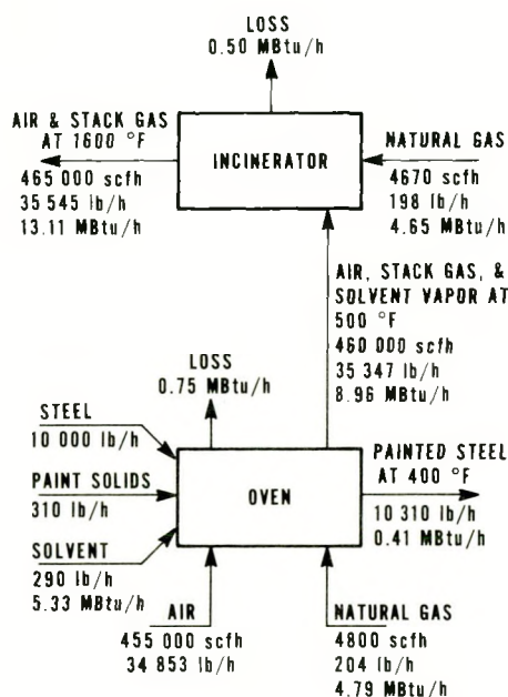
FIGURE 13. Heat balance for a paint drying oven and fume incinerator.
