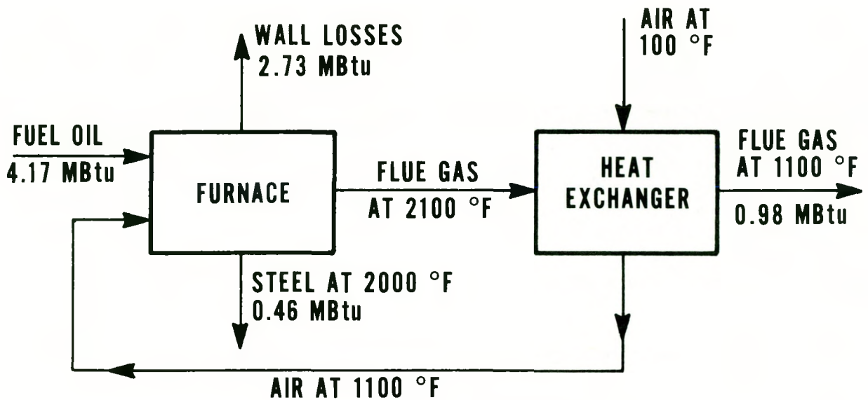
FIGURE 3. Batch furnace with preheated combustion air (third heat balance).
