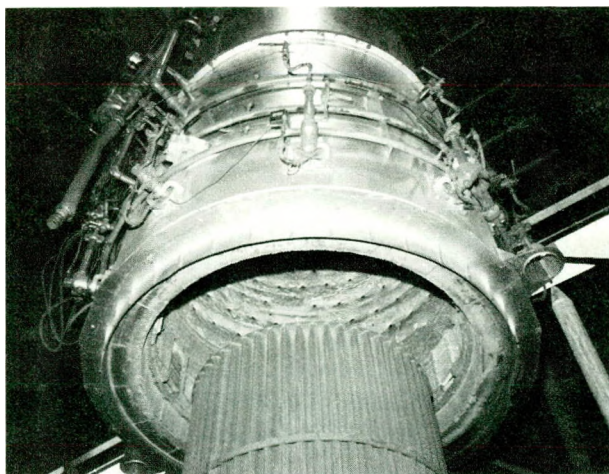
FIGURE 19. A bell, or pedestal, furnace. Reprinted from INDUSTRIAL HEATING, February 1975.
