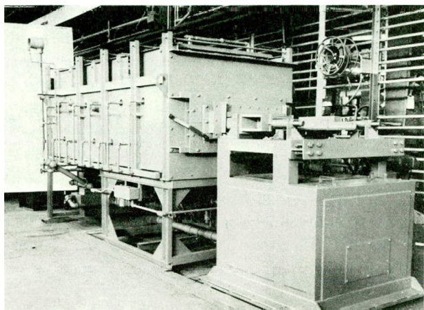
FIGURE 21. A shaker hearth furnace. Courtesy of American Gas Furnace Co.
