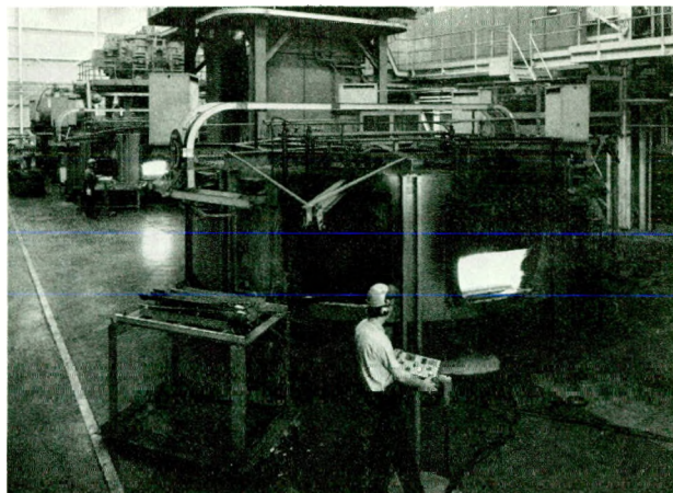
FIGURE 20. A rotary hearth furnace, electrically heated, with endothermic gas atmosphere. Courtesy of Flynn and Dreflein Engineering Co.
