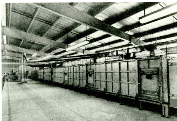
FIGURE 23. A kiln for the drying and curing of automobile exhaust control catalyst. Reprinted from INDUSTRIAL HEATING, September 1975.
