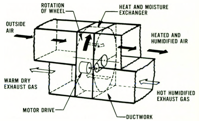
FIGURE 10. Heat and moisture recovery using a heat wheel type regenerator.
