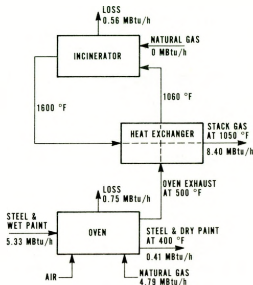
FIGURE 5. Paint drying oven, fume incinerator, and heat exchanger.
