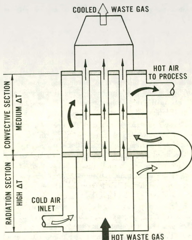
FIGURE 7. Diagram of combined radiation- and convective-type recuperator.
