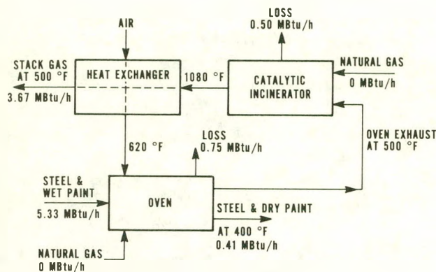
FIGURE 6. Paint drying oven, catalytic incinerator, and heat exchanger.
