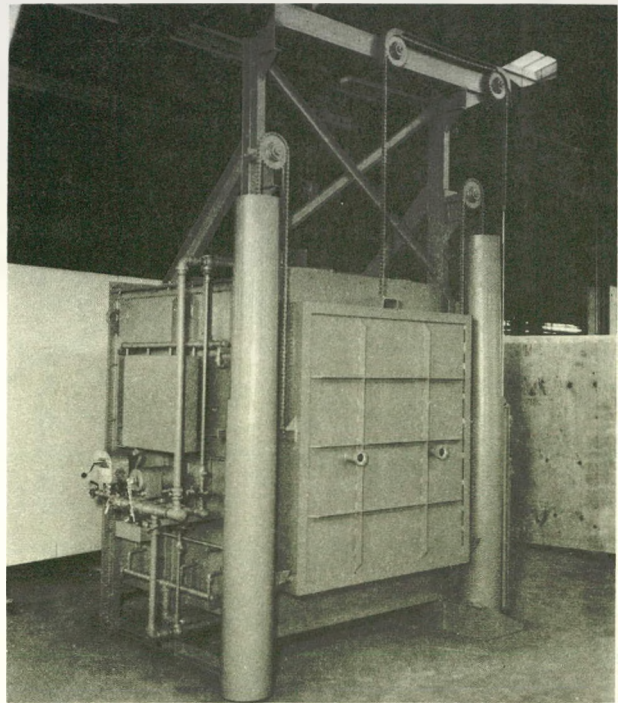
FIGURE 16. A gas fired box furnace. Courtesy of American Gas Furnace Co.
