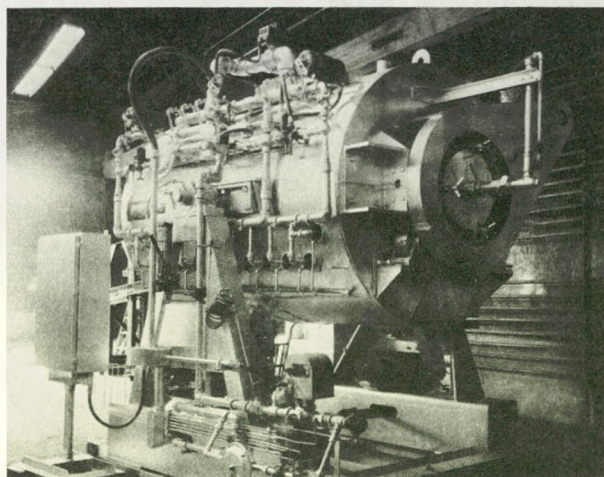
FIGURE 22. A batch type rotary carburizer. Courtesy of American Gas Furnace Co.
