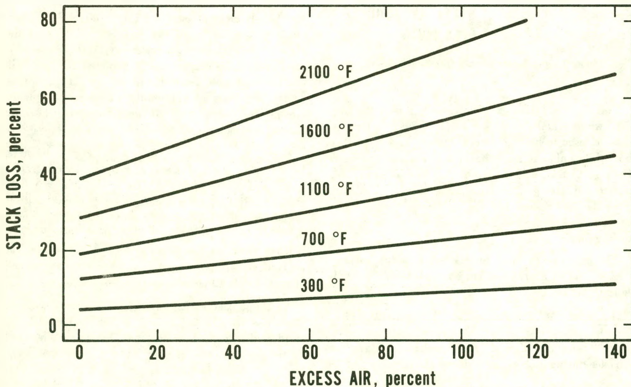
FIGURE 2. Stack loss (wasted fuel energy in stack gases) versus excess air, at various stack gas temperatures.
