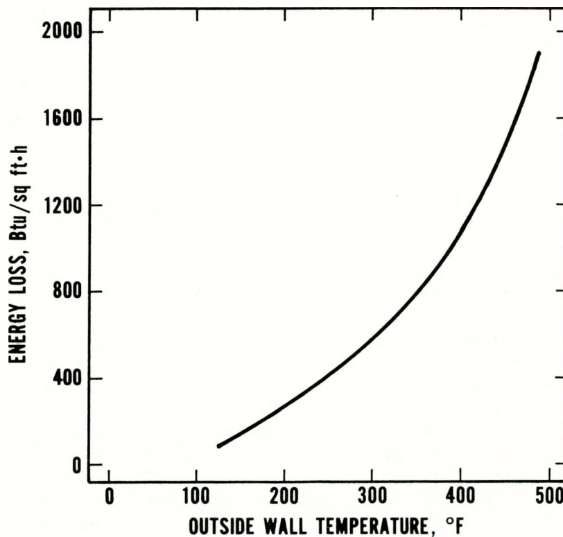
FIGURE 11. Energy loss from furnace walls versus outside wall temperature.
