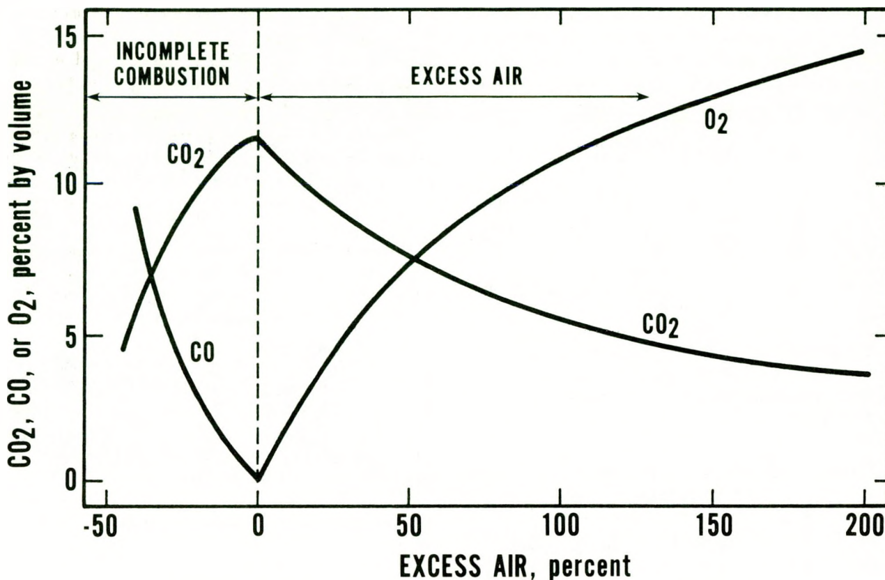
FIGURE 15. Effect of excess air on flue gas analysis for combustion of natural gas.
