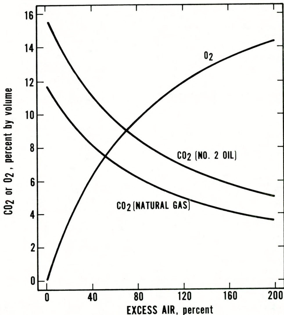
FIGURE 14. Excess air determined from CO 2 and O 2 content of dry flue gas.
