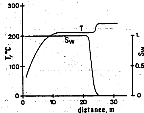
Fig. 1. One-dimensional, porous medium column. Temperature and saturation profiles for q_{inj} = 2.75 \times 10^{-3} \text{ kg/sm}^2 , k = 5 \times 10^{-13} \text{ m}^2 .
