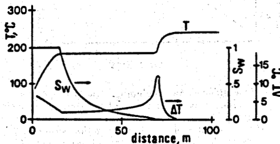
Fig. 5. One-dimensional, fractured medium column. Profiles of temperature and saturation in the fractures and temperature difference between outermost matrix elements and fractures for q_{inj} = 3e-4 \text{ kg/sm}^2 , k=5e-13 \text{ m}^2 .
