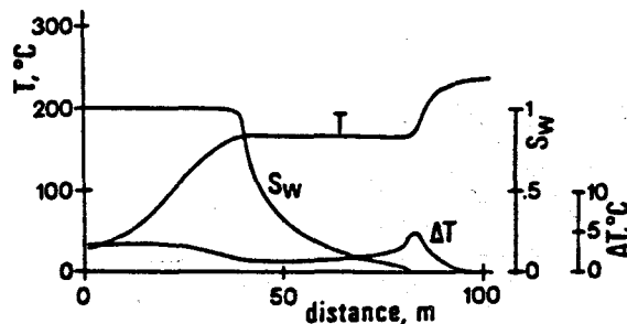
Fig. 7. One-dimensional radial, fractured-porous medium model (injection rate = 2.78 kg/s, k=5 \times 10^{-13} \text{ m}^2 ). Variation with radial distance of temperature and liquid saturation in the fractures, and temperature difference between the outermost matrix elements and fractures.
