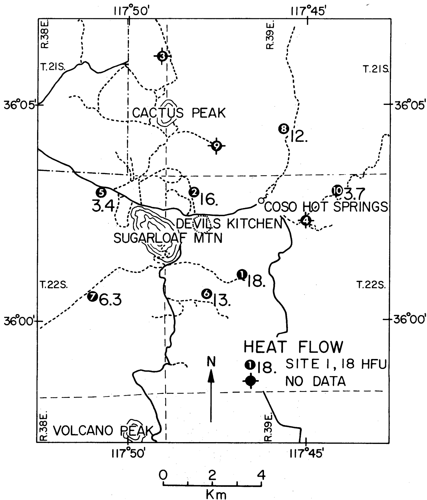
Figure 9. Borehole locations with heat flow determinations in units of \mu\text{cal}/\text{cm}^2\text{-sec.} . The symbol \odot indicates that no geothermal gradient was obtainable from the borehole.
