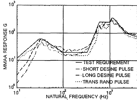
Figure 2: Comparison of SRS for Test Requirement and Three Different Test Specifications
