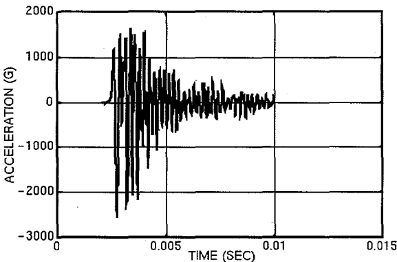
Figure 8: Acceleration History for a Typical Test Specification
