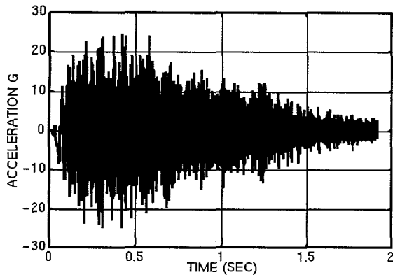
Figure 1: Acceleration History for Response to Launch Ignition Environment (Single Flight)
