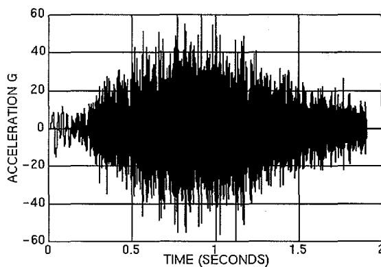
Figure 5: Acceleration History for Transient Random Test Specification
