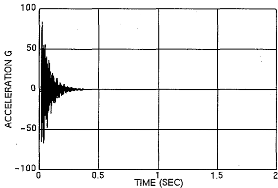
Figure 3: Acceleration History for Short Duration Decayed Sinusoid Test Specification
