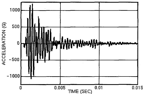
Figure 6: Acceleration History for Severe Field Environment
