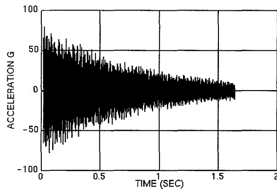
Figure 4: Acceleration History for Long Duration Decayed Sinusoid Test Specification
