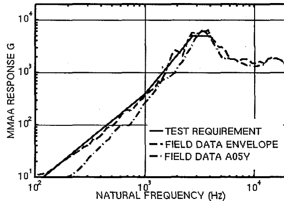
Figure 7: Comparison of SRS for Field Environment and Test Requirement
