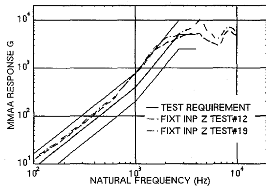
Figure 9: Comparison of SRS for Test Requirement and Two Best Effort Test Specifications
