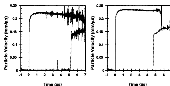
FIGURE 4. Particle velocity waveforms for fine HMX (left side) and C & H confectioners (fine) sugar (right side). The shock transmission times through the compacts are quite close with the sugar being slightly faster, the same as in the coarse materials. The transmitted waves have risetimes of \approx 100 \text{ ns} . Impact velocities were 0.279 mm/ \mu\text{s} (HMX Shot 982) and 0.299 mm/ \mu\text{s} (sugar Shot 1020).
