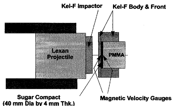
FIGURE 2. Schematic of the sugar experiments. Kel-F cell was impacted by a Kel-F faced projectile. Stirrup magnetic gauges were located on both sides of the sugar compact. Stirrup gauges are single element gauges with a 10-mm long active end that is situated perpendicular to the magnetic field lines.
