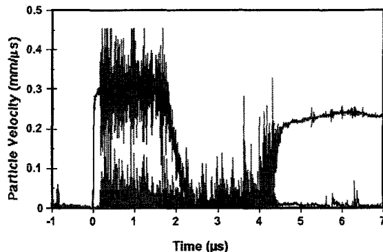
FIGURE 7. Particle velocity waveforms from coarse sugar Shot 1014 with an impact velocity of 0.4 mm/μs. Both the original record and the smoothed record are shown. Notice that the noise stops as soon as all the crushing is complete, i.e., the transmitted wave reaches near the maximum particle velocity in the back gauge.
