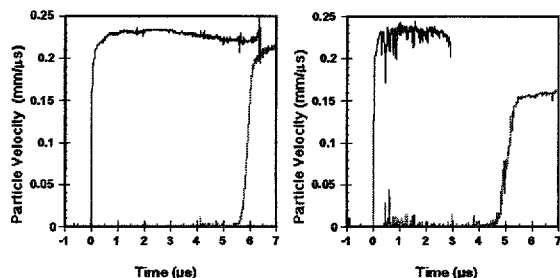
FIGURE 3. Particle velocity waveforms for coarse HMX (left side) and C & H granulated (coarse) sugar (right side). The shock transmission times through the compacts are quite close with the sugar being slightly faster. The transmitted waves are disperse, each with risetimes > 0.5 \mu\text{s} . Impact velocities were 0.288 mm/ \mu\text{s} (HMX Shot 912) and 0.295 mm/ \mu\text{s} (sugar Shot 1015).
