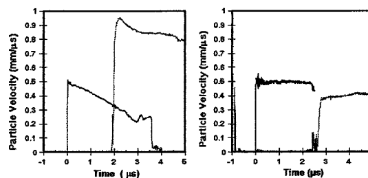
FIGURE 5. Particle velocity waveforms for coarse HMX (left side) and C & H granulated (coarse) sugar (right side). The shock transmission time through the HMX is faster because of the reaction and the wave front buildup. Obviously the HMX waveforms result from reaction occurring in the HMX compact. Impact velocities were 0.696 mm/ \mu\text{s} (HMX Shot 913) and 0.700 mm/ \mu\text{s} (sugar Shot 1017).
