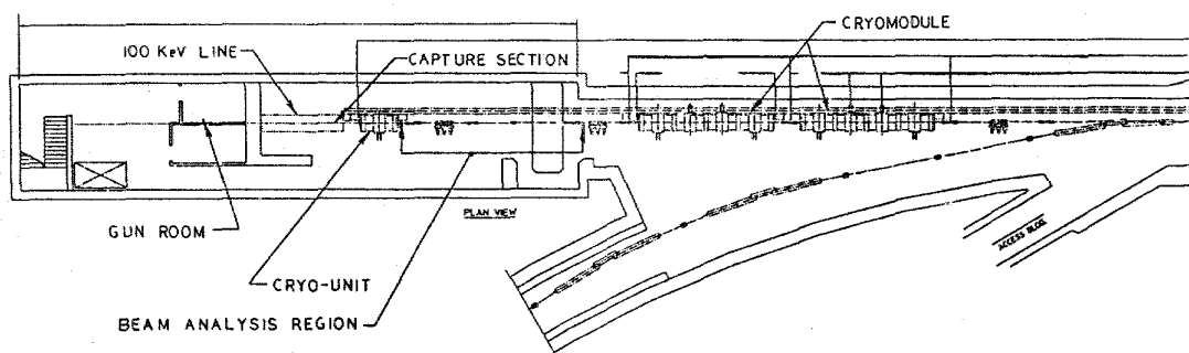
Figure 1 General layout of the CEBAF injector. Either of two guns can be used to provide a 100 keV beam that is chopped, bunched and accelerated to 500 keV in the room temperature section. The cryounit increases the energy to over 5 MeV and the 2 cryomodules produce a 45 MeV beam for injection into the rest of the linac.
