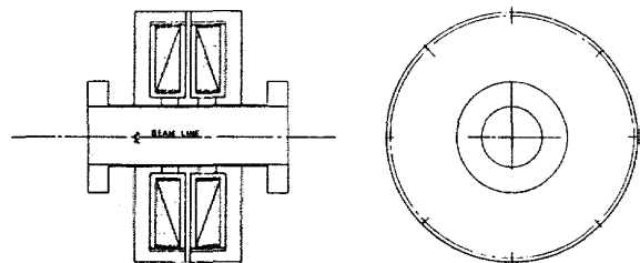
Figure 4 Details of the focusing coils used for the 100 keV line.
