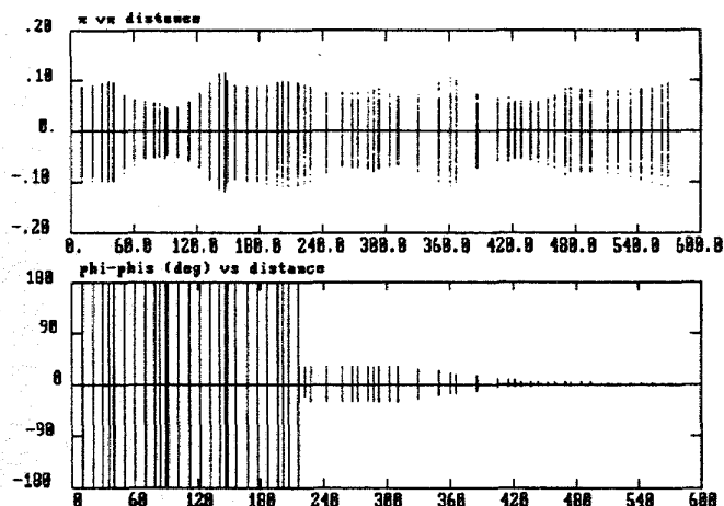
Figure 2 PARMELA calculations of the beam radius and longitudinal phase space for the 100 keV line.
