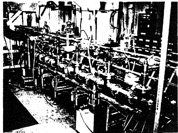
Figure 3 Photograph of the 100 keV line.
