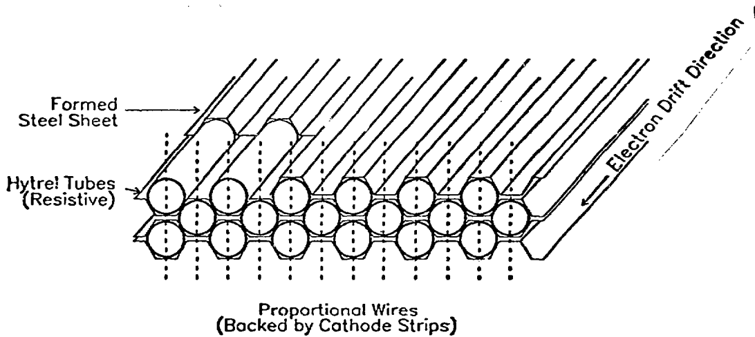
Fig. 2. Closeup of Honeycomb Pattern in Drift Chamber
