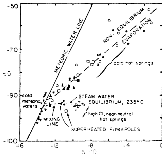
Figure 6.--Diagram showing relations between deuterium and ^{18}O for water and steam samples from LVNP and vicinity. ●, Bumpass Hell; □, lower Little Hot Springs Valley;
