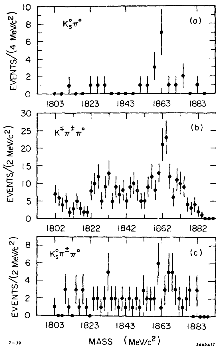
Fig. 14. Beam-energy-constrained mass distribution from the Mark II experiment with various D decays.
