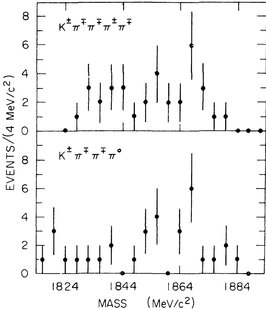
Fig. 15. Charged D decays to K^{\pm} \pi^{\mp} \pi^{\mp} \pi^{\pm} \pi^{\mp} and K^{\pm} \pi^{\mp} \pi^{\mp} \pi^{\circ} (beam-constrained).
