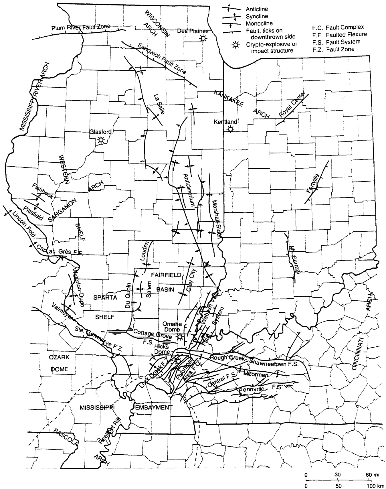
Figure 12 Selected structural features in Illinois (modified from Treworgy 1981).
