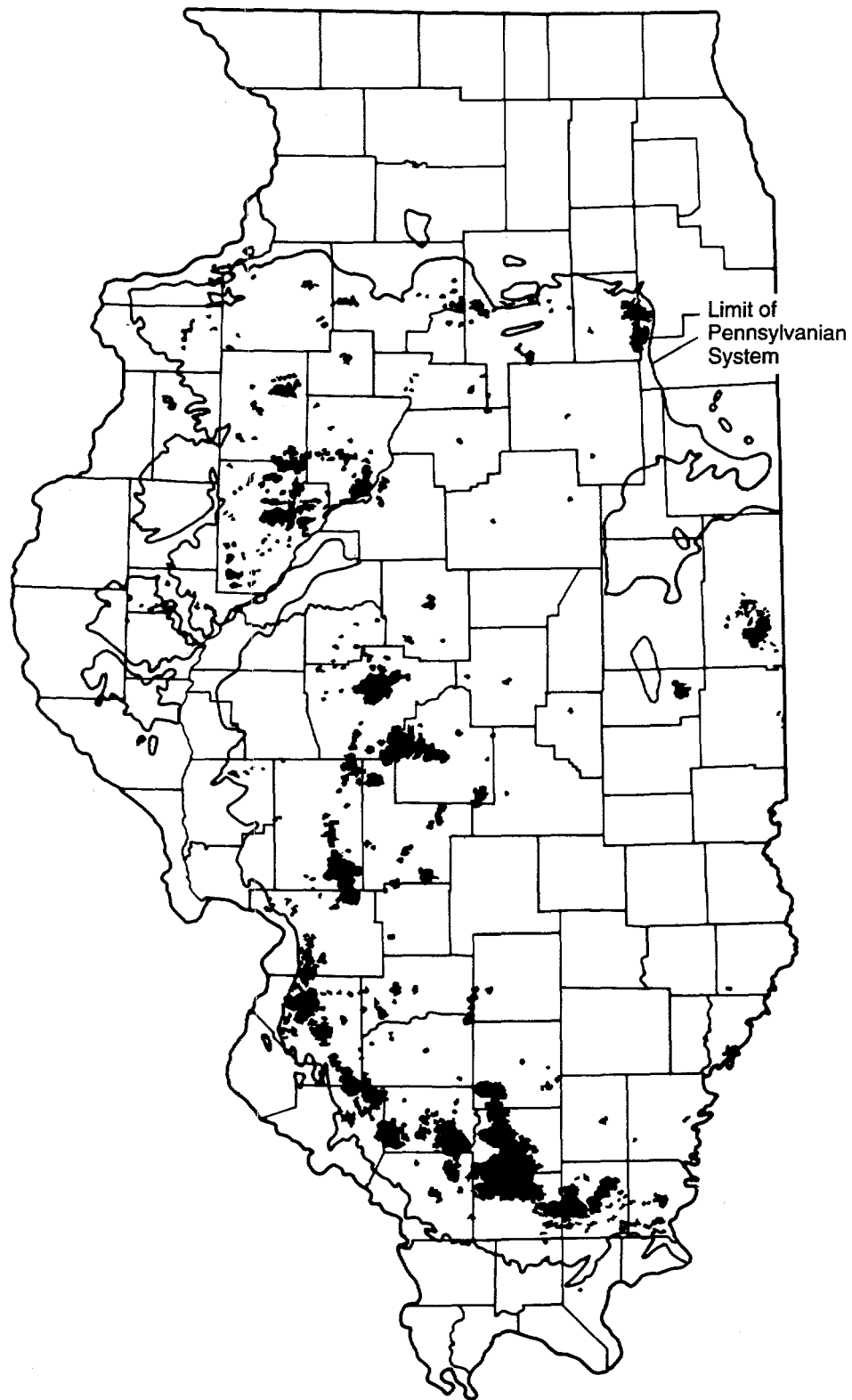
Figure 6 Locations of coal mines.
