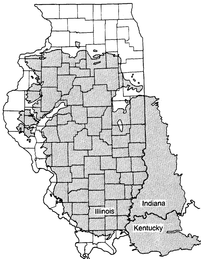
Figure 1 Illinois Basin, or Eastern Interior Coal Field.
