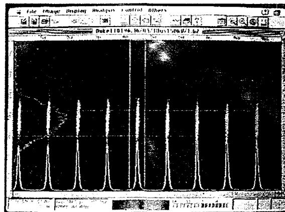
Figure 2: Dual-sweep streak camera image of the SER from the OK-4 at \lambda = 450 nm and for a beam energy of 500 MeV. The vertical sweep covers 800 ps while the horizontal axis is 10 \mu s. These are single-bunch data taken turn by turn. The measured bunch length at 150 kV rf gap voltage and I_B = 1.6 ma is 160 ps (FWHM).
