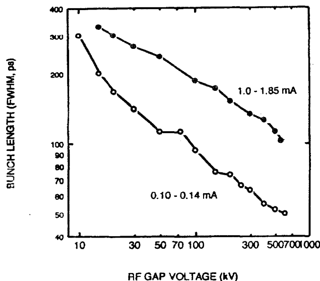
Figure 4: Plot of the variation of beam bunch length with rf gap voltage. The two sets of data are from low current (0.10-0.14 mA) and medium current (1.0-1.85 mA) runs.
