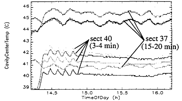
Figure 5: Rf cavity temperature variation in two sectors.
