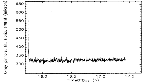
Figure 6: Constant horizontal beam size, 100-mA store, after CB instability compensation.
