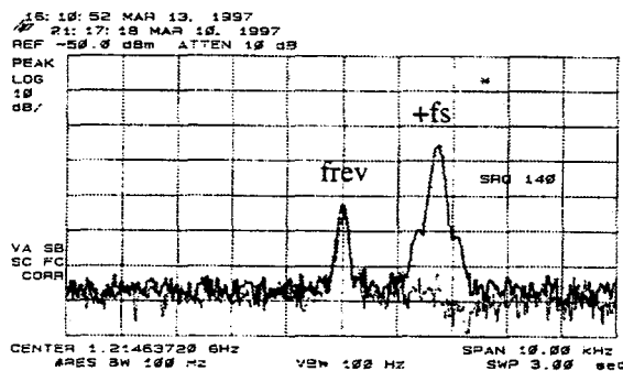
Figure 7: Rf cavity signals centered on 1214.64 MHz.
