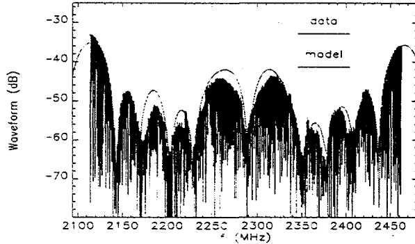
Figure 2: Unstable beam spectrum, 4x12 bunch pattern.
