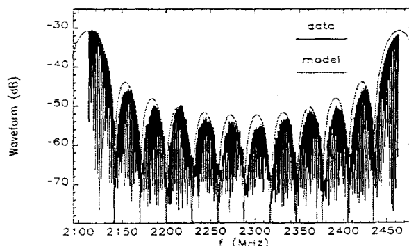
Figure 1: Stable beam spectrum, 4 \times 12 bunch pattern.
