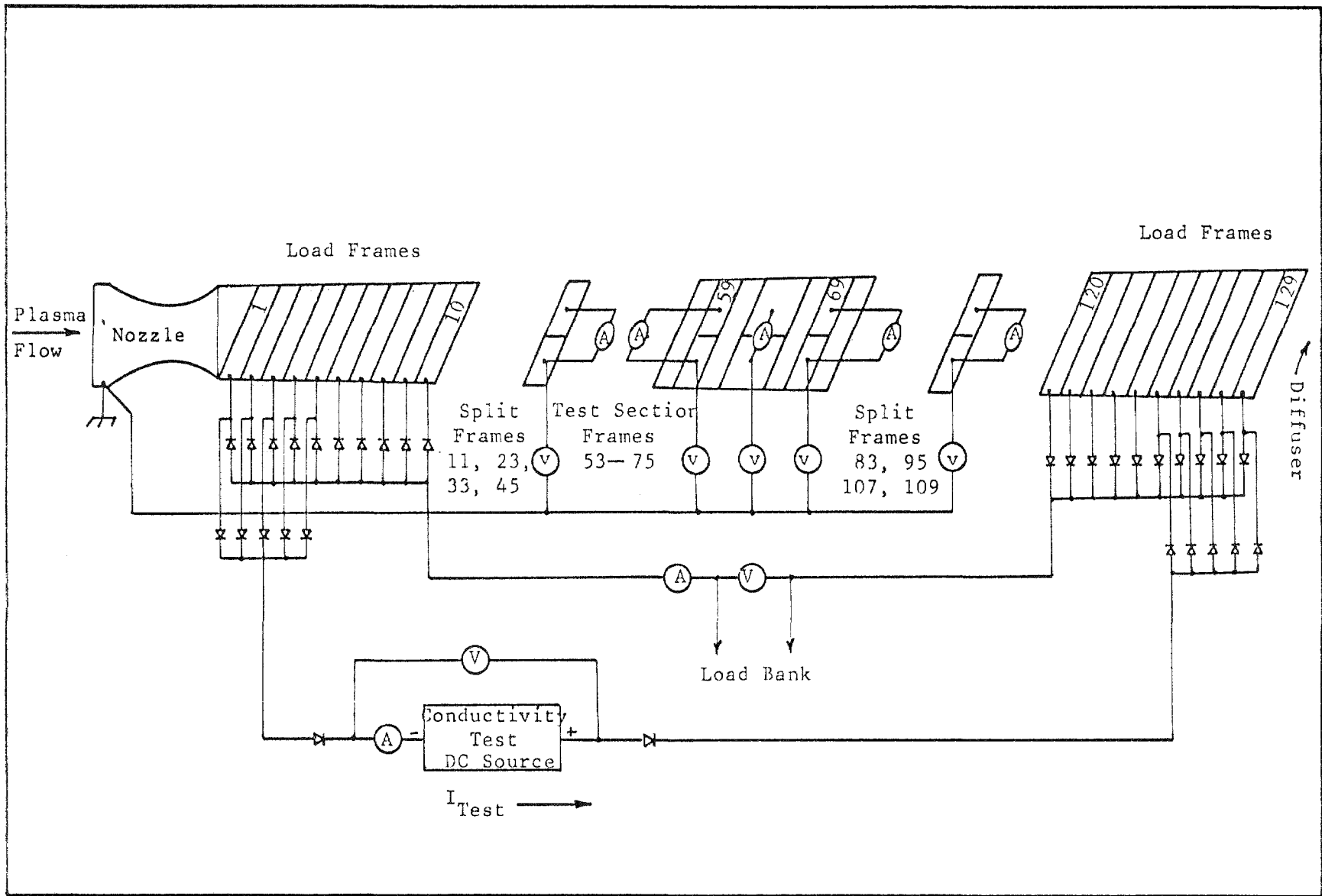
Fig. 13 MHD Channel Test Set-Up for Conductivity Measurements
