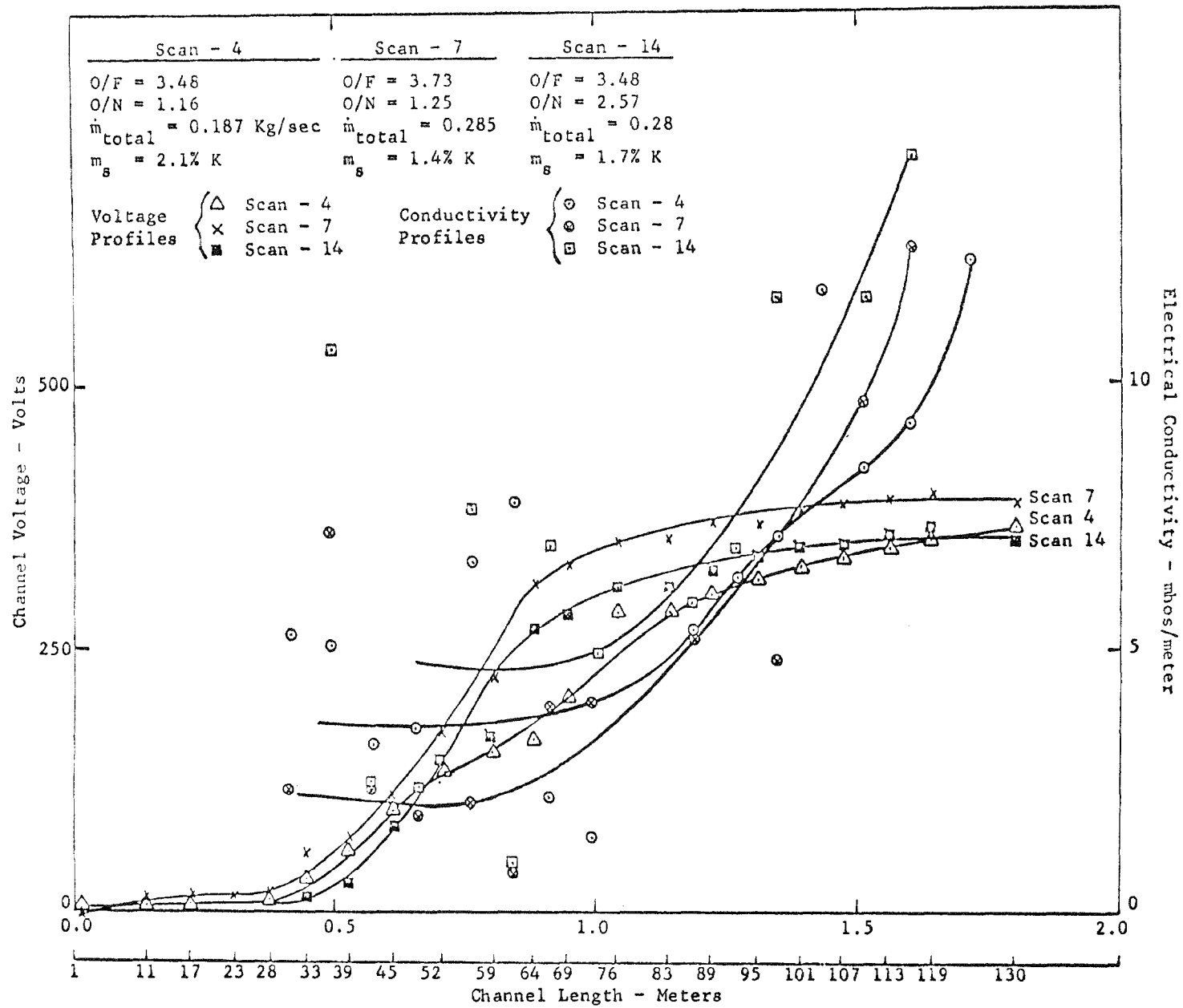
Fig. 14 Voltage Distribution and Plasma Conductivity Profile in the Channel
