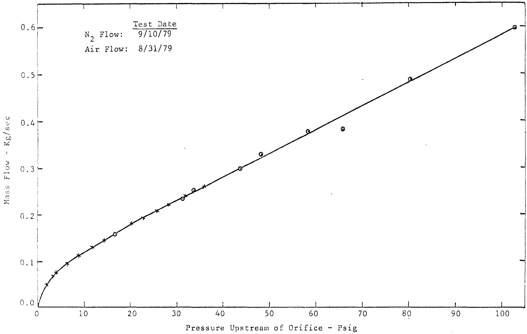
Fig. 8 Air and N 2 Flow Calibration Using New Flow Meter
