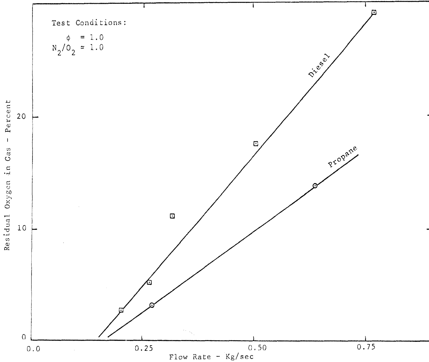
Fig. 12 Variation of Residual Oxygen Present at the Combustor Exit with Gas Flow Rate
