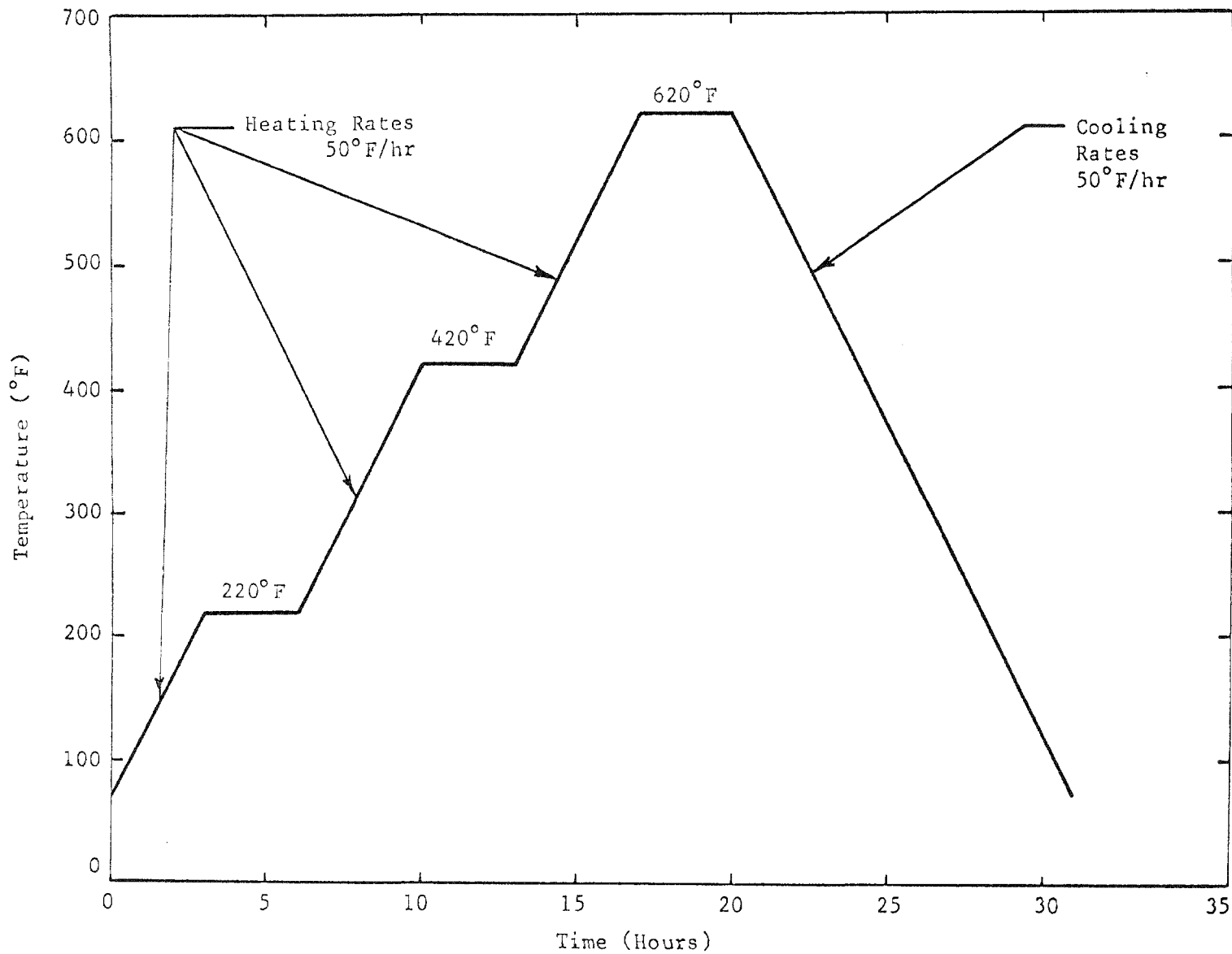
Fig. 5 Heat Treatment for Ceramic Liner (Temperature - Time History)
