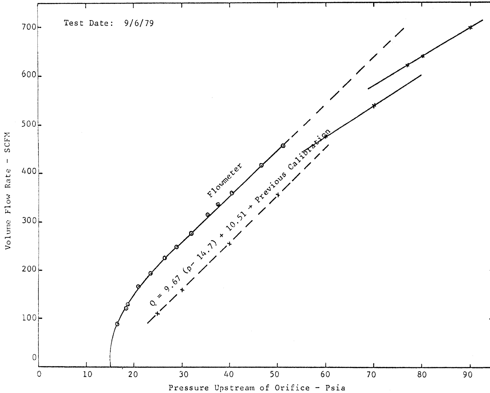
Fig. 7 Nitrogen Flow Calibration Using New Flow Meter
