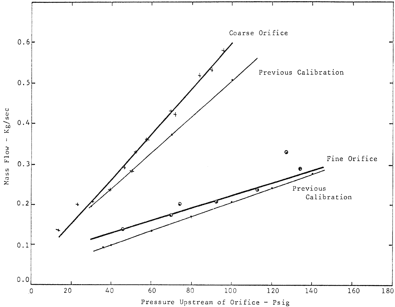
Fig. 6 Oxygen Flow Calibration Using New Flow Meter
