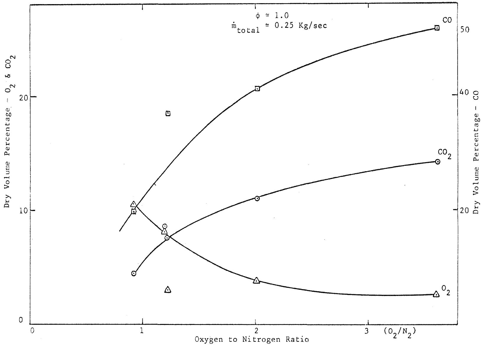
Fig. 11 Gas Composition at Combustor Exit for Various O_2/N_2 Ratios
