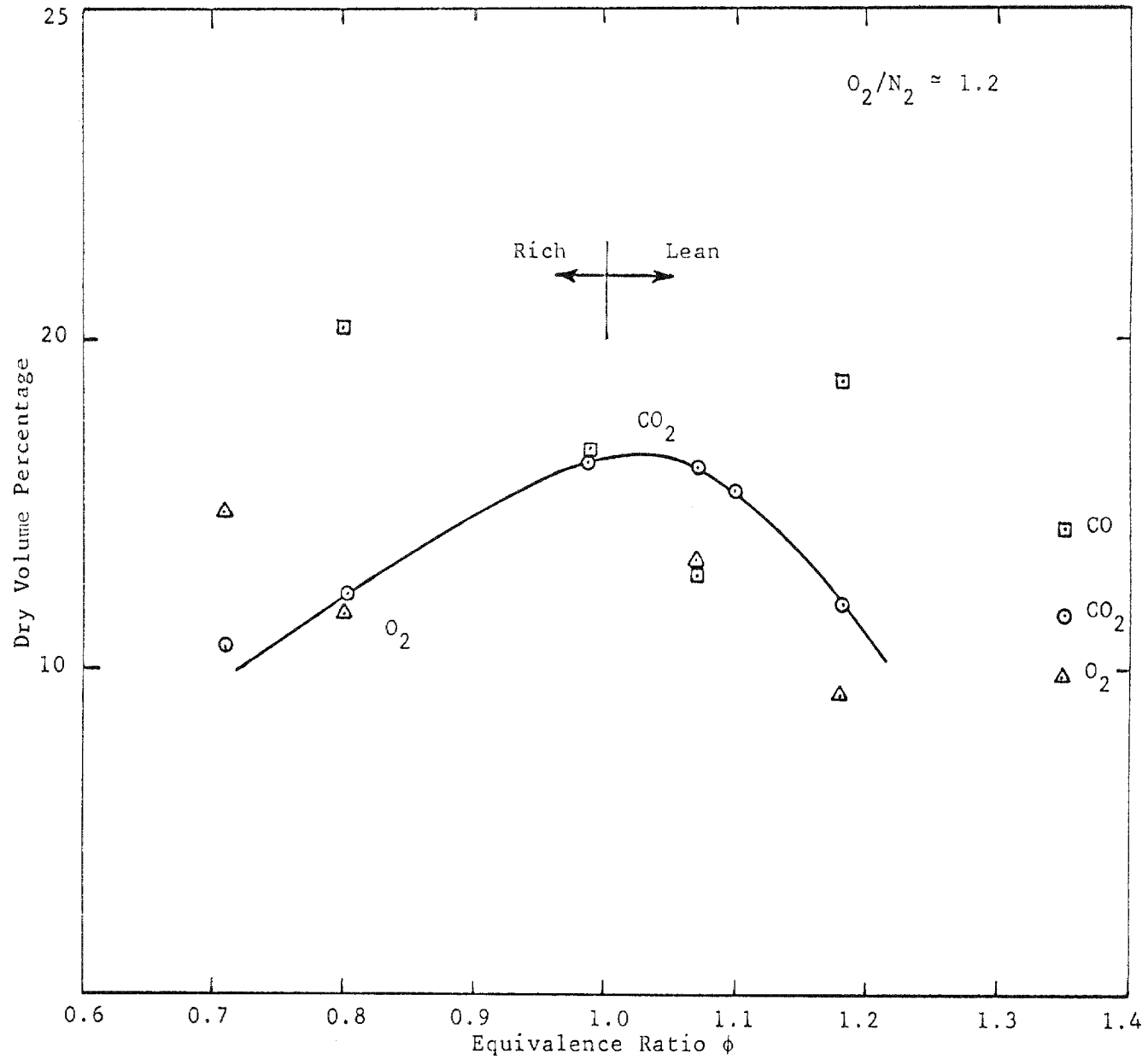
Fig. 10 Gas Composition at Combustor Exit for Various Equivalence Ratios
