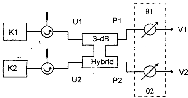
Figure 2: Two klystron-two sector feeding through a hybrid.
