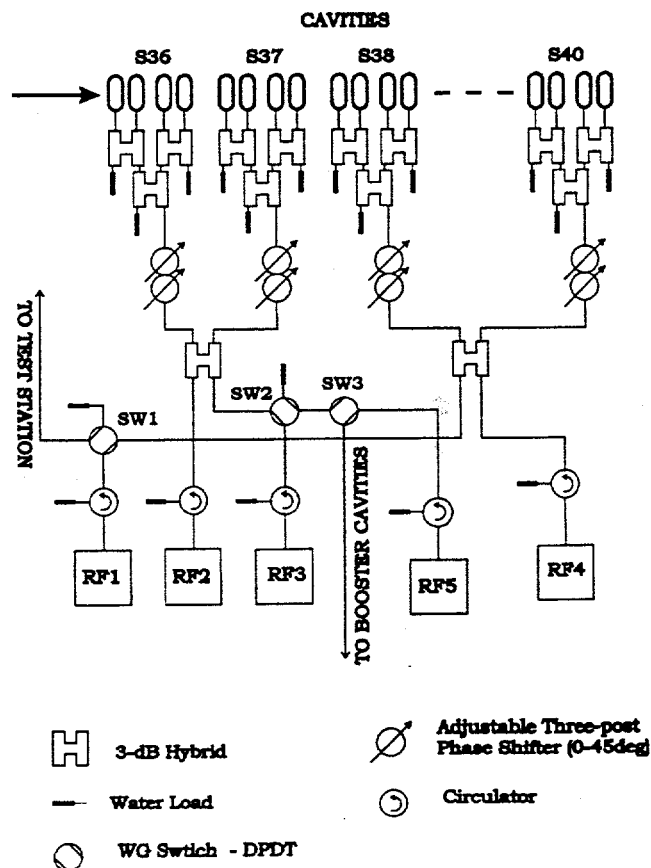
Figure 1: Reconfigurable waveguide switching system.
