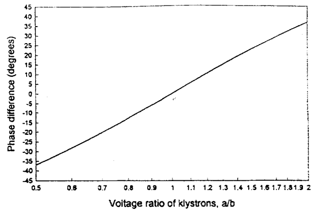
Figure 3: Phase difference between two outputs vs. the input power imbalance.
