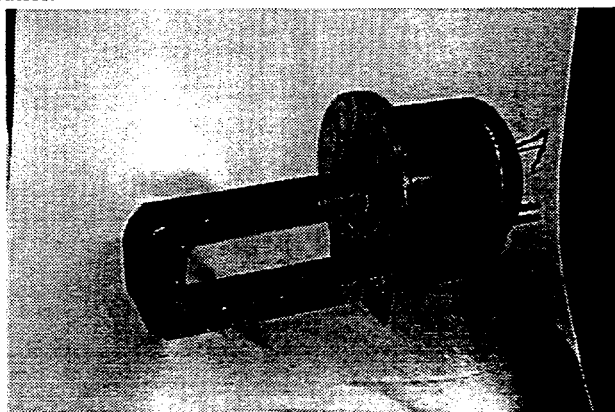
Figure 3: Ferrite tuner for the 9.77-MHz fundamental frequency cavity.
