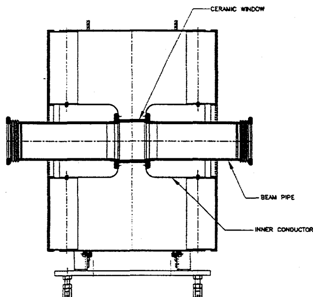
Figure 2: Harmonic cavity structure.
