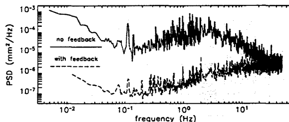
Figure 2: Horizontal power spectral density ('DC' mode).
