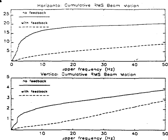
Figure 4: Cumulative rms beam motion above 10mHz ('Highpass' mode).
