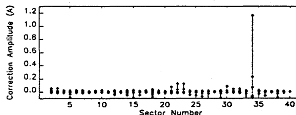
Figure 5: Glitching power supply identified on-line using BPM data alone.
