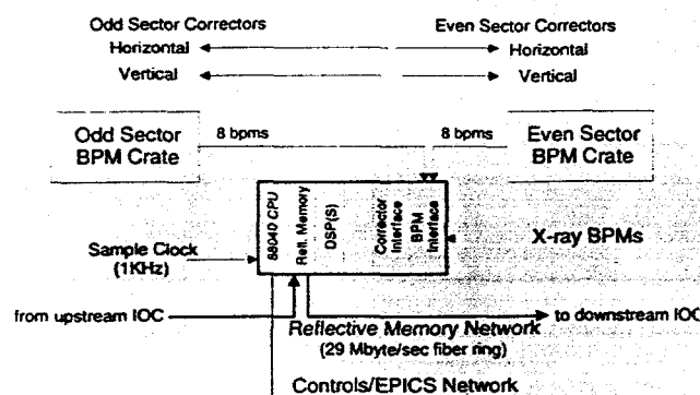
Figure 1: Architecture of a typical orbit feedback crate.
