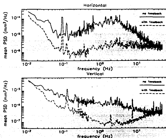
Figure 3: Power spectral density ('Highpass' mode).
