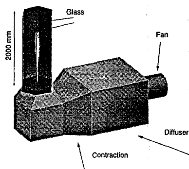
Figure 1: Sketch of the test facility
