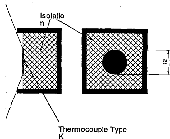
Figure 2: Sketch of the black plate sensor
