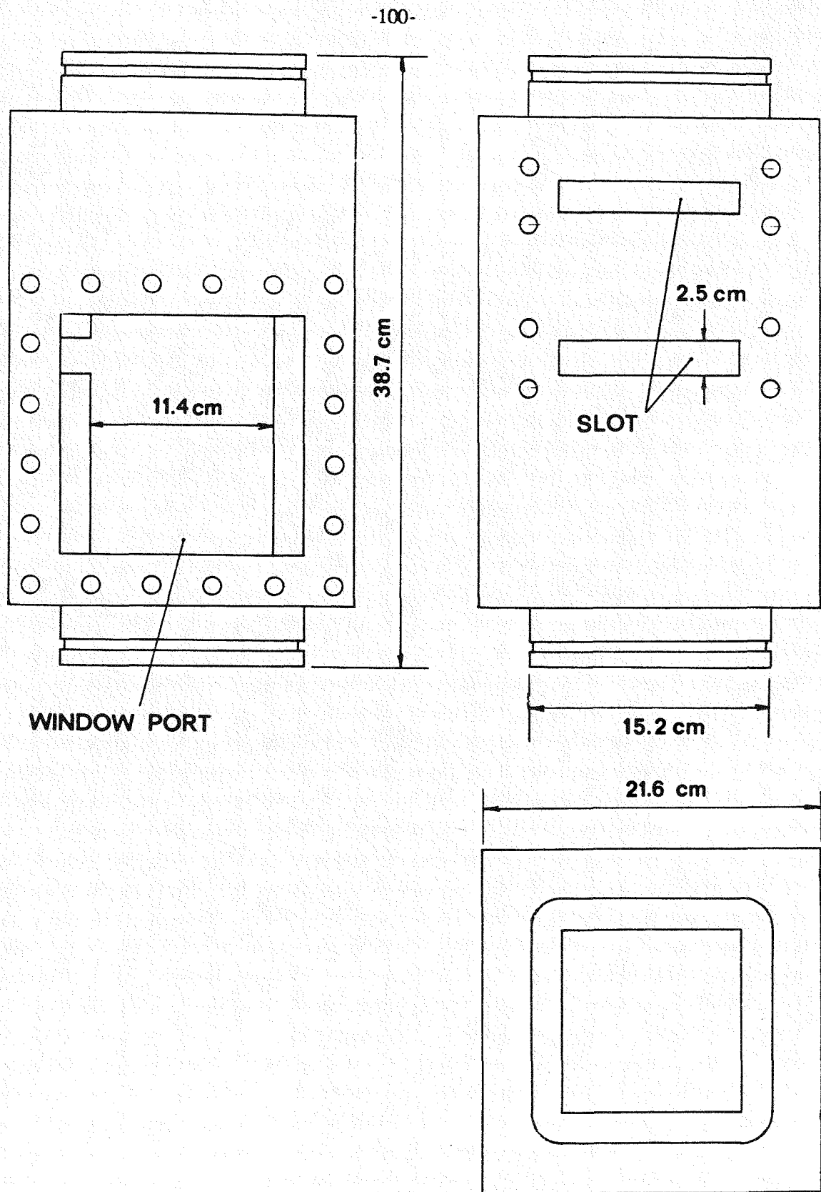
Figure 2.4 Test section.
