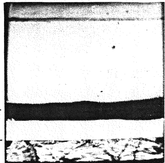
Figure 4.3 Single-scale Richtmyer-Meshkov instability at a continuous interface. Air/SF 6 M_s = 1.32 , close end wall configuration.
