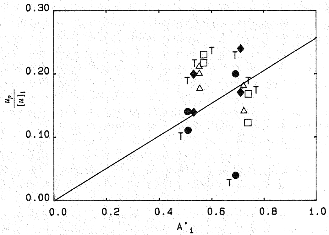
Figure 6.9 Wall vortex penetration speed, long time configuration. Incident shock Mach number: ● : 1.12. ◆ : 1.32, △ : 1.48, □ : 1.66. T: indicates the thicker interface for each test gas at a given Mach number in Table 5.3.
