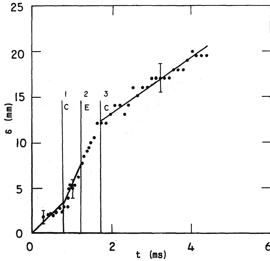
Figure 5.17 Time evolution of the thickness of the TMZ for the plane discontinuous interface between air and \text{SF}_6 . M_s = 1.32 , close end wall configuration.
