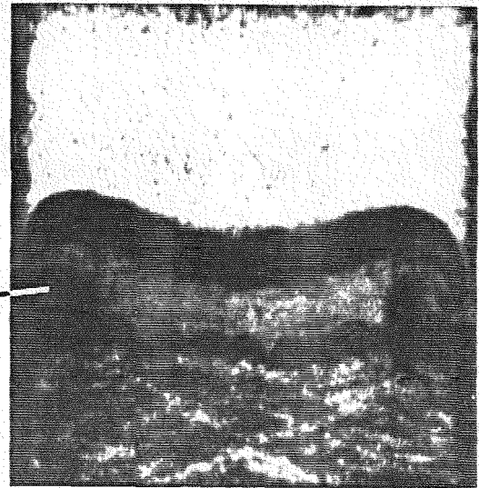
Figure 5.20 Richtmyer-Meshkov instability of a plane continuous interface between air and \text{SF}_6 . M_s = 1.32 , long time configuration.
