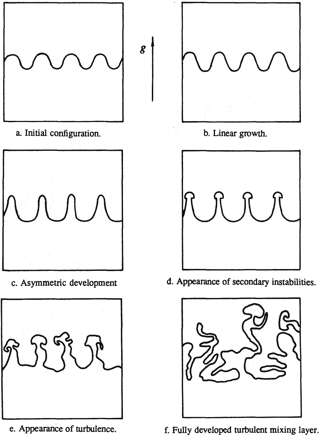
Figure 3.3 Evolution of single-scale perturbations for Rayleigh-Taylor instability.
