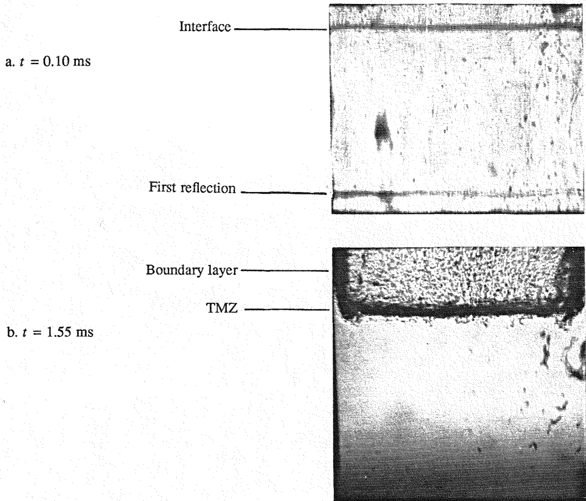
Figure 5.11 Richtmyer-Meshkov instability of a plane discontinuous interface between air and helium. M_s = 1.30, 1.32 , close end wall and long time configurations.
