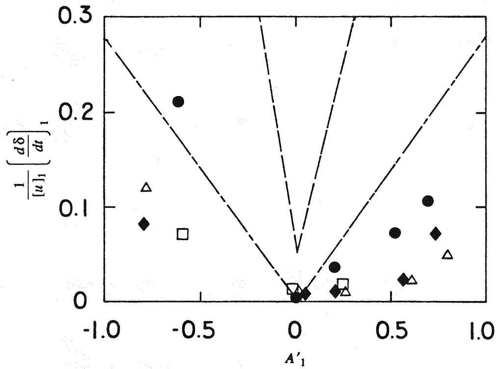
Figure 5.26 Correlation of reshock shock growth rates for the discontinuous interface experiments in the long time configuration. Incident shock Mach number: ●: 1.12, ◆: 1.32, △: 1.48, □: 1.66.—: Zaitsev et al. (1985), — — — : Equation (3.23).
