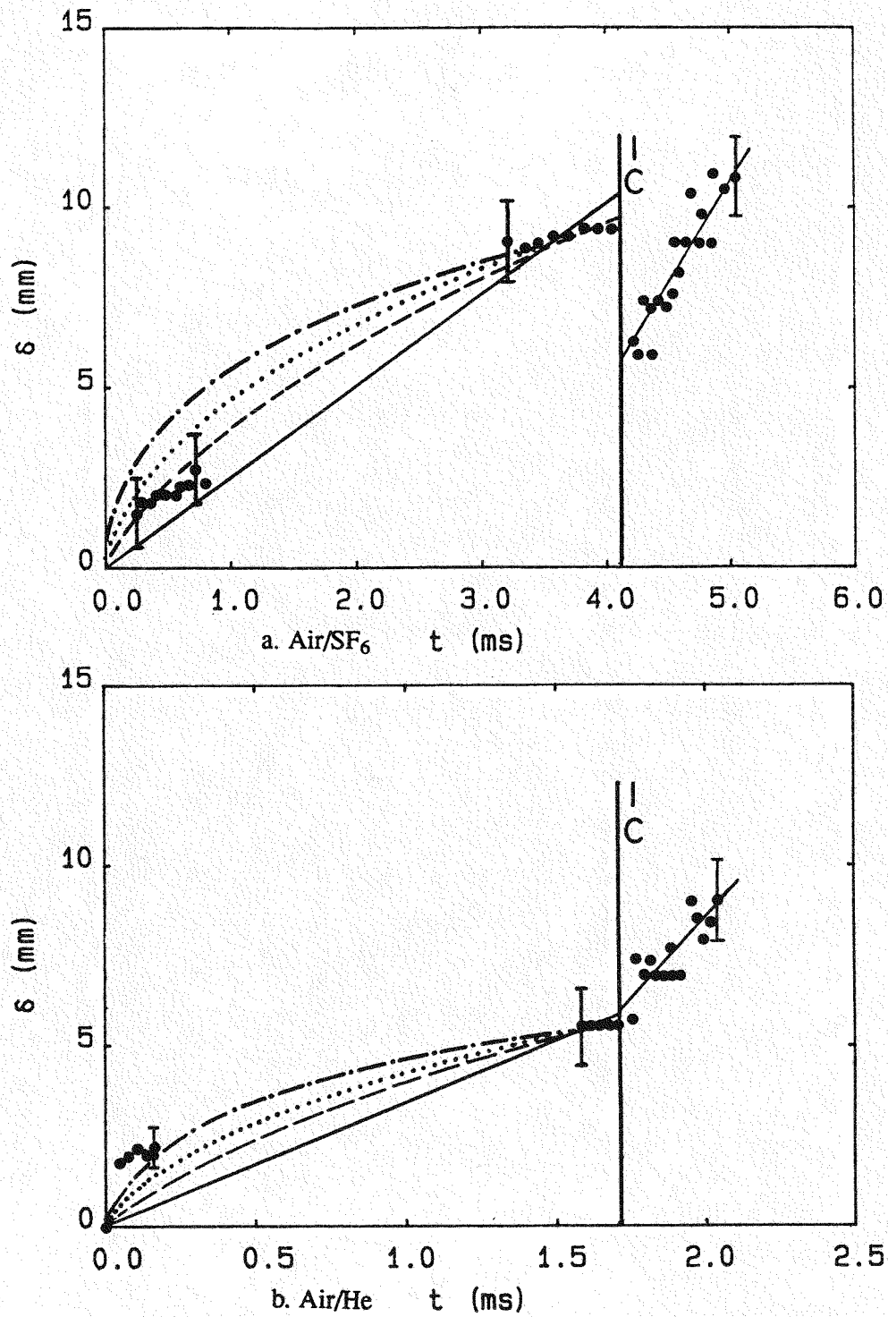
Figure 5.24 Time evolution of the thickness of the TMZ for two discontinuous interface experiments. Long time and close end wall configurations. — : linear profile ( \alpha = 1 ), - - - : \alpha = 2/3 , - - - : \alpha = 1/2 , - - - : \alpha = 1/3 .
