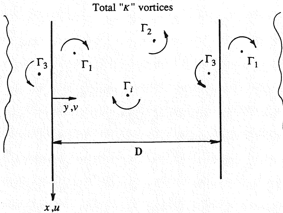
Figure D.1 Infinite system periodic in the y -direction, consisting of periodic cells of width D each with " \kappa " vortices.
