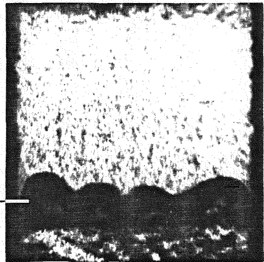
Figure 4.5 Single-scale Richtmyer-Meshkov instability at a continuous interface. \text{Air/SF}_6 M_s = 1.32 , long time configuration.
