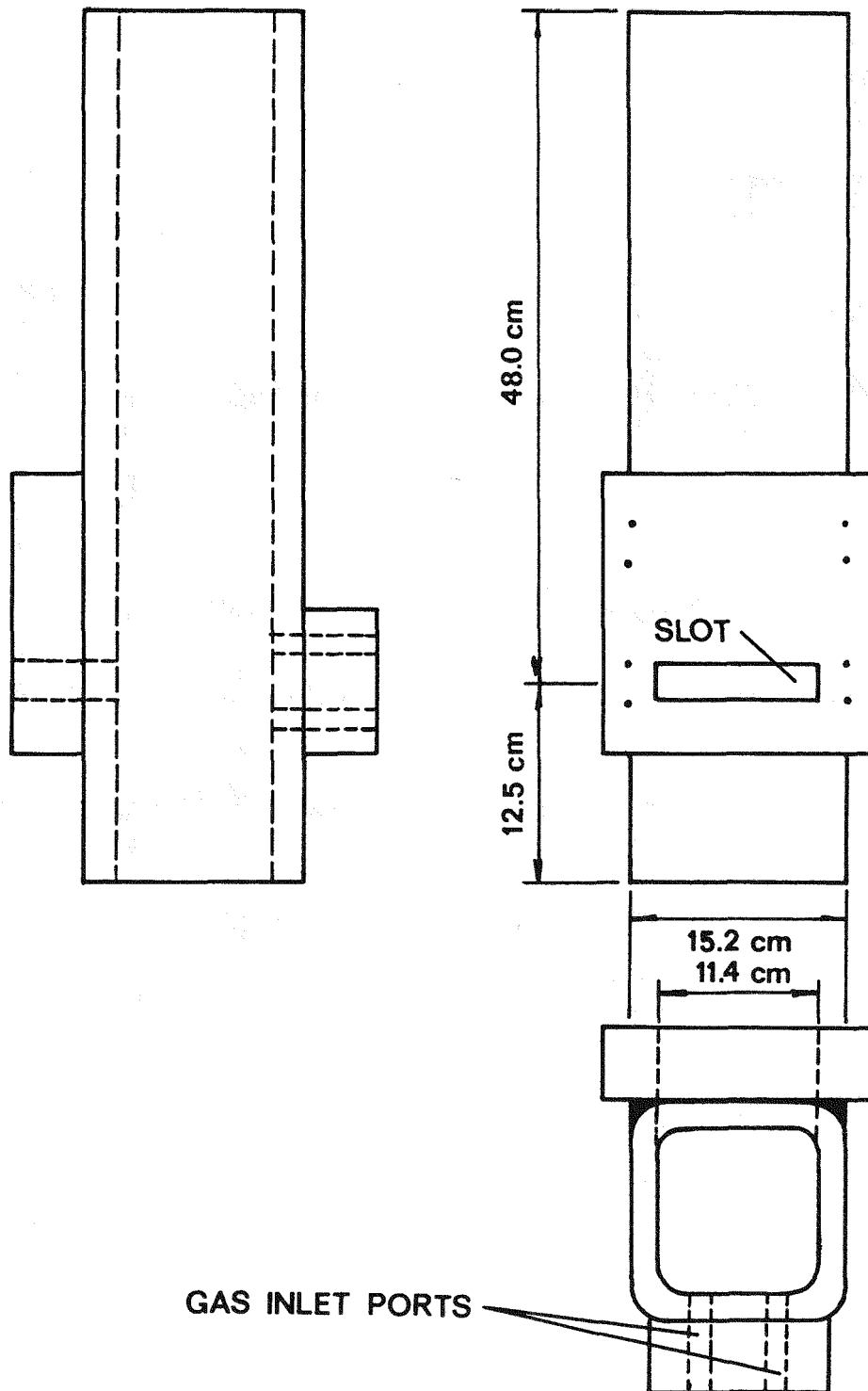
Figure 2.5 Interface section.
