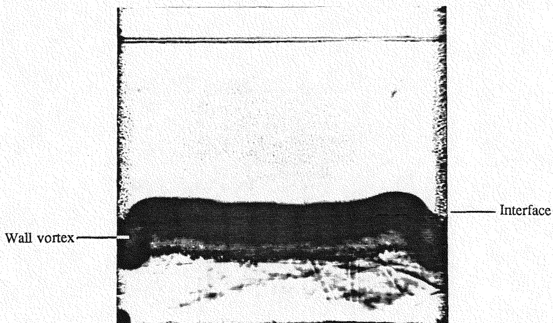
Figure 5.22 Richtmyer-Meshkov instability of a plane continuous interface between air and \text{SF}_6 . M_s = 1.32 , close end wall configuration, t = 1.91 ms. Note the \text{SF}_6 -containing boundary layers visible on the side walls of the tube and the random acoustic field below the interface.
