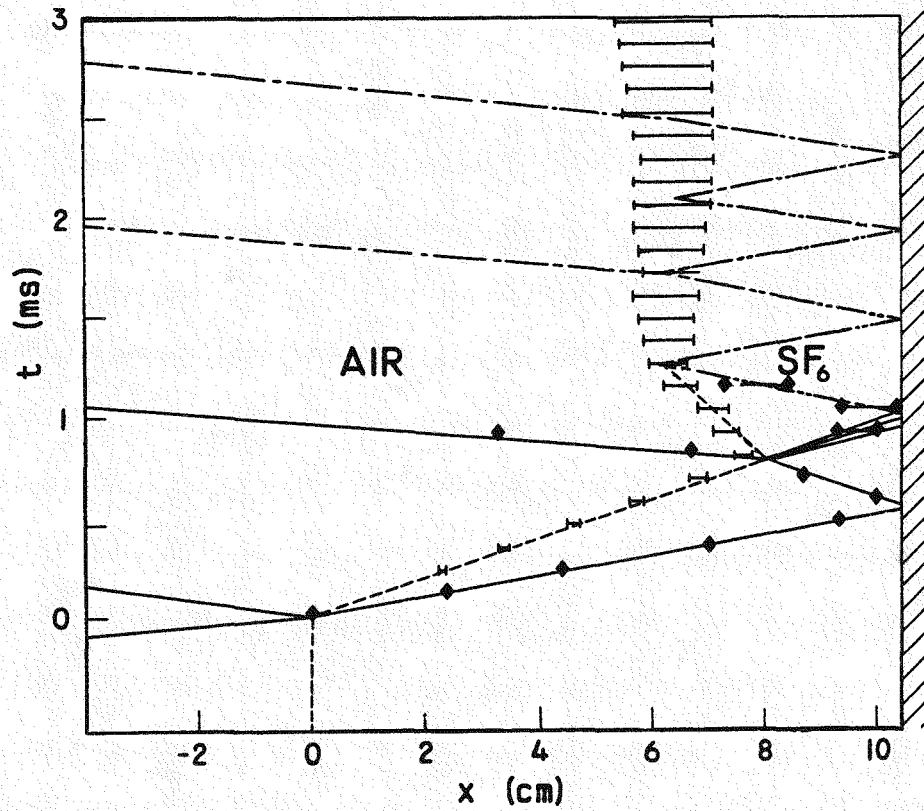
Figure 5.4 Wave diagram for the interaction of a M_s = 1.32 shock wave with a plane discontinuous interface between air and \text{SF}_6 , close end wall configuration. The interface trajectory is indicated by: — theory, —♦— experiment. The wave trajectories are indicated by: — theory, —♦— experiment, —·— deduced.
