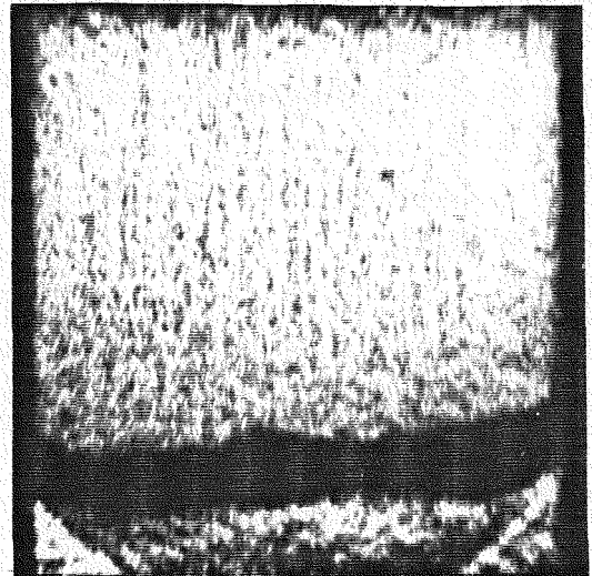
Figure 4.4 Single-scale Richtmyer-Meshkov instability at a continuous interface. \text{Air/SF}_6 M_s = 1.32 , long time configuration.
