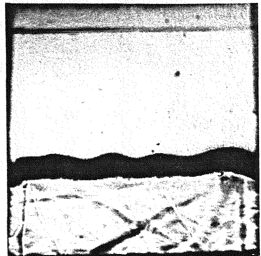
Figure 4.7 Single-scale Richtmyer-Meshkov instability at a continuous interface. Air/SF 6 M_s = 1.32 , close end wall configuration.
