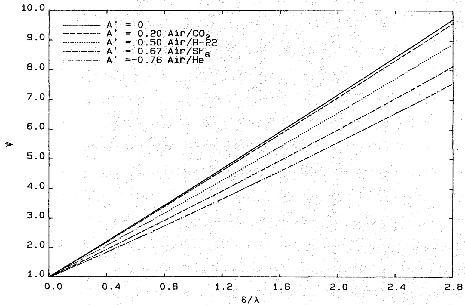
Figure 3.5 Growth reduction factor.
