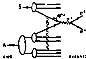
Fig. 4. Induced radiation from the interaction of the active antiquark with target spectators in the Drell-Yan process. The inelastic interactions are suppressed at parton energies which are large compared to a scale set by the length of the target. 14
