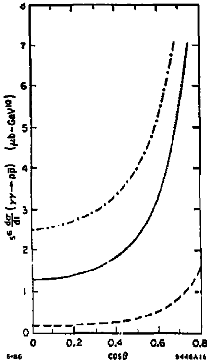
Fig. 13. QCD prediction for the scaling and angular distribution for \gamma + \gamma \rightarrow p + p calculated by Farrar et al. 24 The dashed-dot curve corresponds to \frac{1}{Q_0^2} = 0.0016 and a maximum running coupling constant \alpha_s^{\text{max}} = 0.8 . The solid curve corresponds to \frac{1}{Q_0^2} = 0.016 and a maximum running coupling constant \alpha_s^{\text{max}} = 0.5 . The dashed curve corresponds to a fixed \alpha_s = 0.3 . The results are very sensitive to the endpoint behavior of the proton distribution amplitude. The CZ form is assumed.
