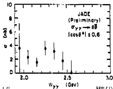
Fig. 15. Recent preliminary data from JADE 25 for \gamma + \gamma \rightarrow \beta + p .
