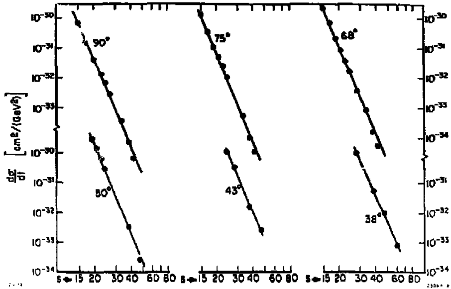
Fig. 7. Comparison of proton-proton scattering at fixed \theta_{cm} with the dimensional counting prediction. The best fit is s^{-2.7} . See ref. 18.
