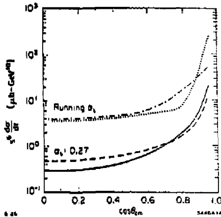
Fig. 14. QCD prediction for the scaling and angular distribution for \gamma + \gamma \rightarrow p + p calculated by Gunion, Sparks, and Millers. 25 CZ distribution amplitudes 4 are assumed. The solid and running curves are for real photon annihilation. The dashed and dot-dashed curves correspond to one photon spacelike, with \frac{Q_1^2}{Q_0^2} = 0.1 .
