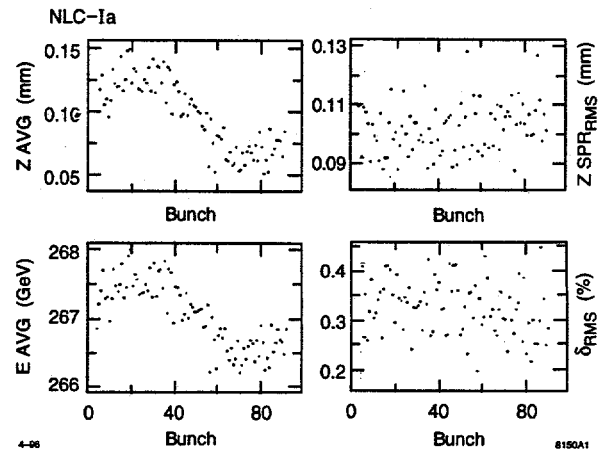
Figure 1: Bunch centroid position, rms bunch length, average bunch energy, and rms energy spread, as a function of bunch number in a train of 90 bunches, for NLC-Ia.
