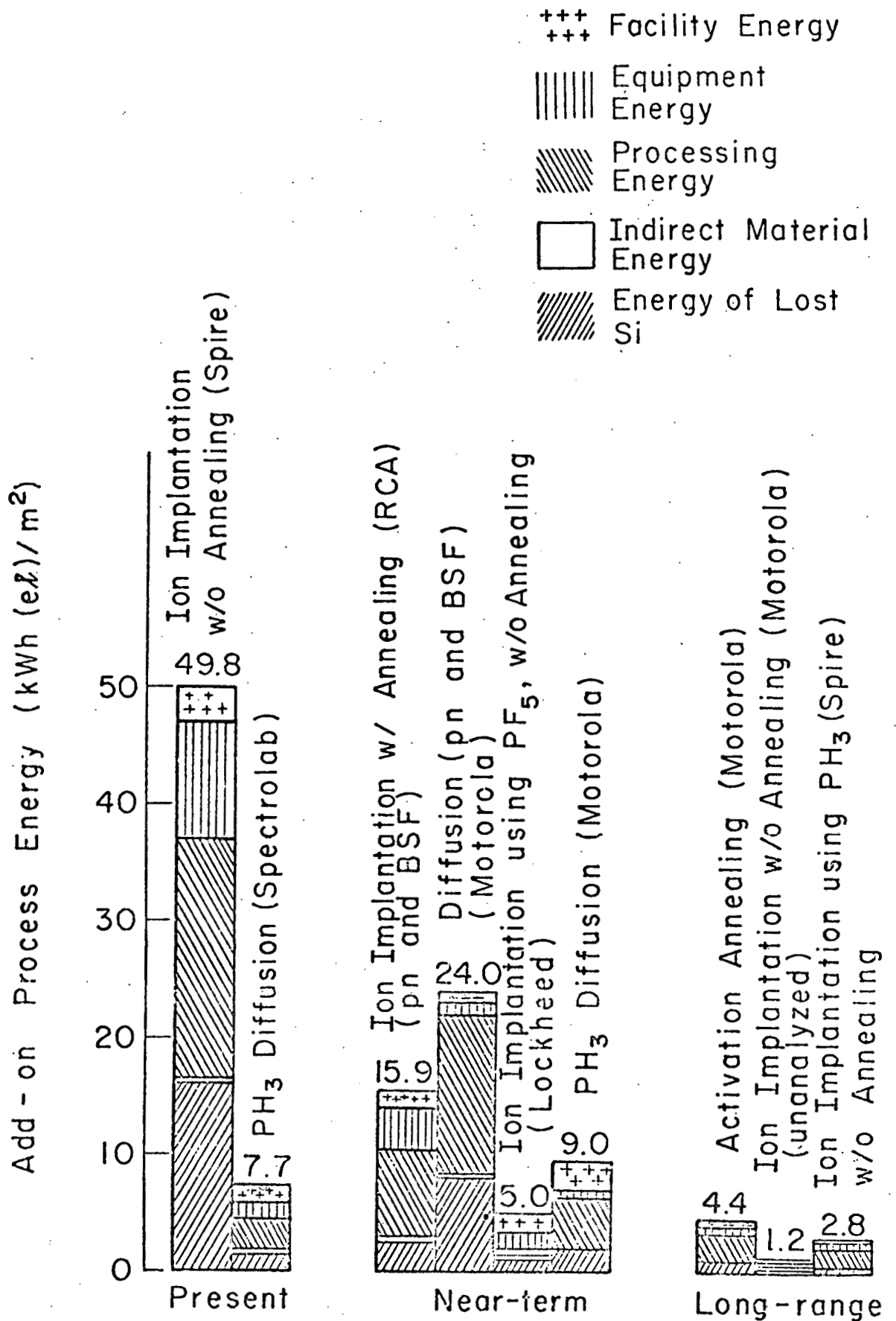
Figure 1: Junction Formation Process Add-On Energies
