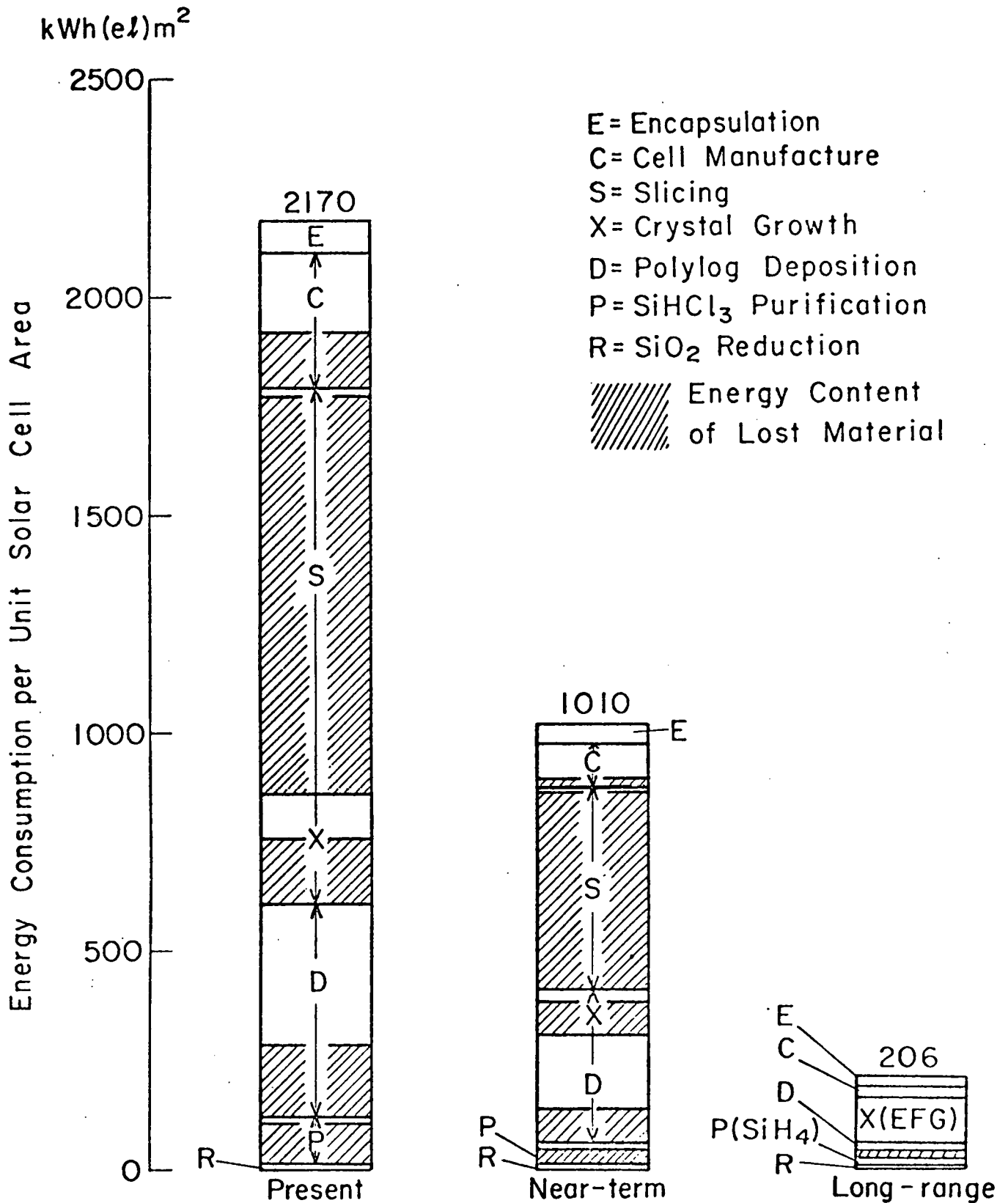
Figure 2: Processing Energy Components For Module Manufacturing
