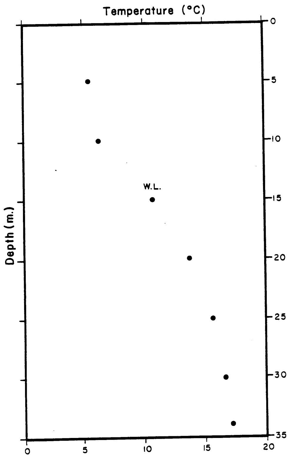
Figure 8. Temperature - depth profile, Hailey Hot Springs area; data from well 2N-18E-18acc
