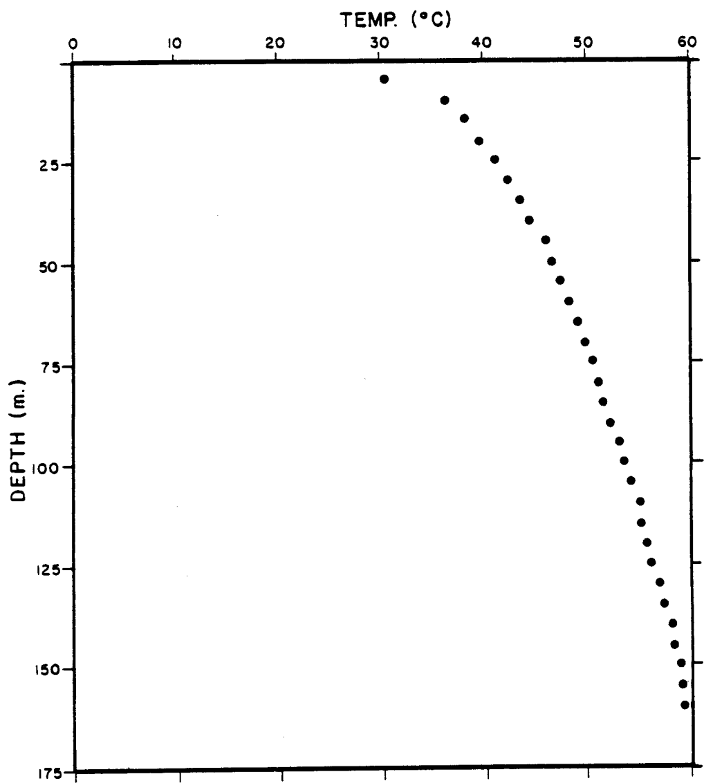
Figure 11. Temperature - depth profile, Guyer Hot Springs area; data from well 4N-17E-15aac
