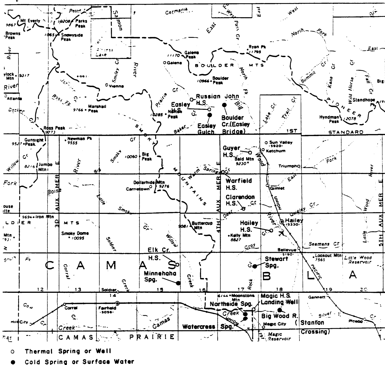
Figure 16. Isotope sample locations in the Wood River drainage area
