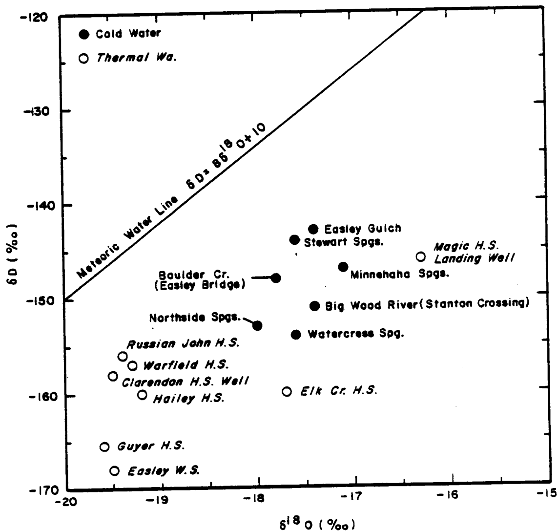
Figure 15. Isotopic composition of selected thermal and nonthermal waters from the Wood River drainage area
