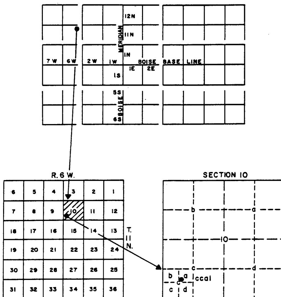
FIGURE 3. Diagram showing the well-and spring-numbering system. (Using well 11N-6W-10ccal.)
