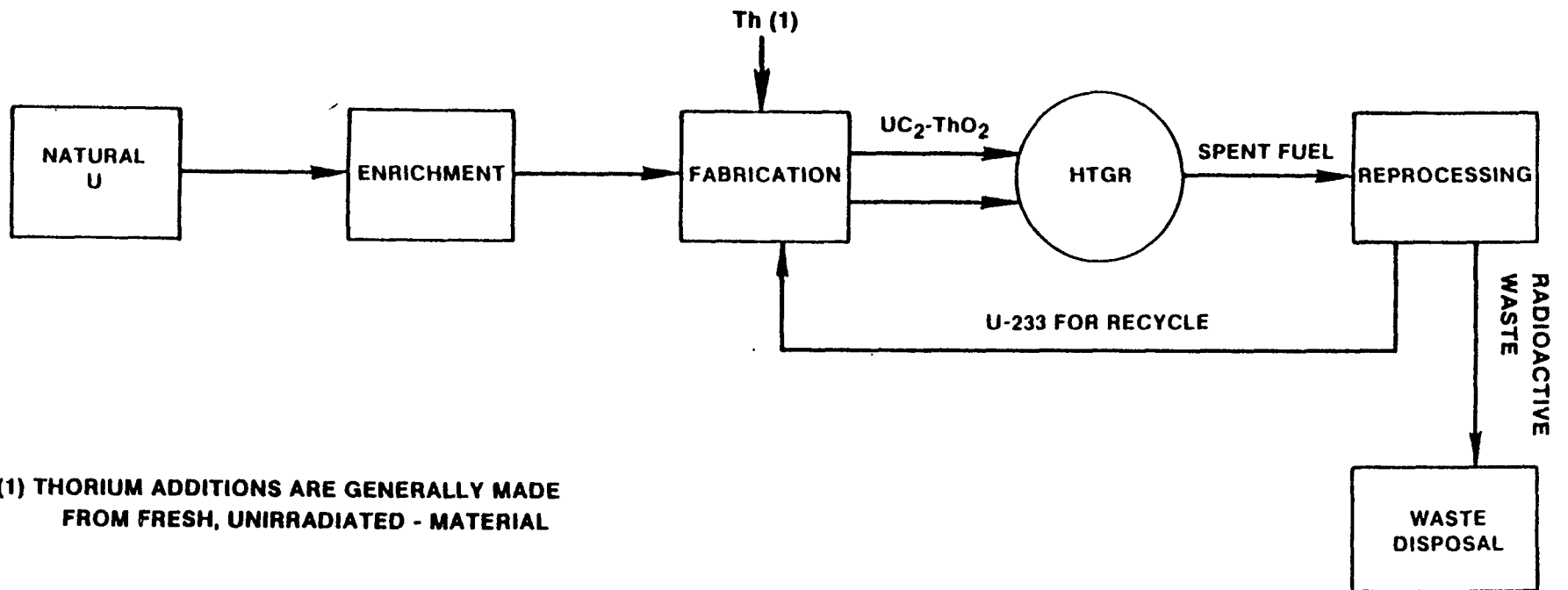
(B) U-233 RECYCLE (HTGR-U5 (DE)/U/Th-20%)
