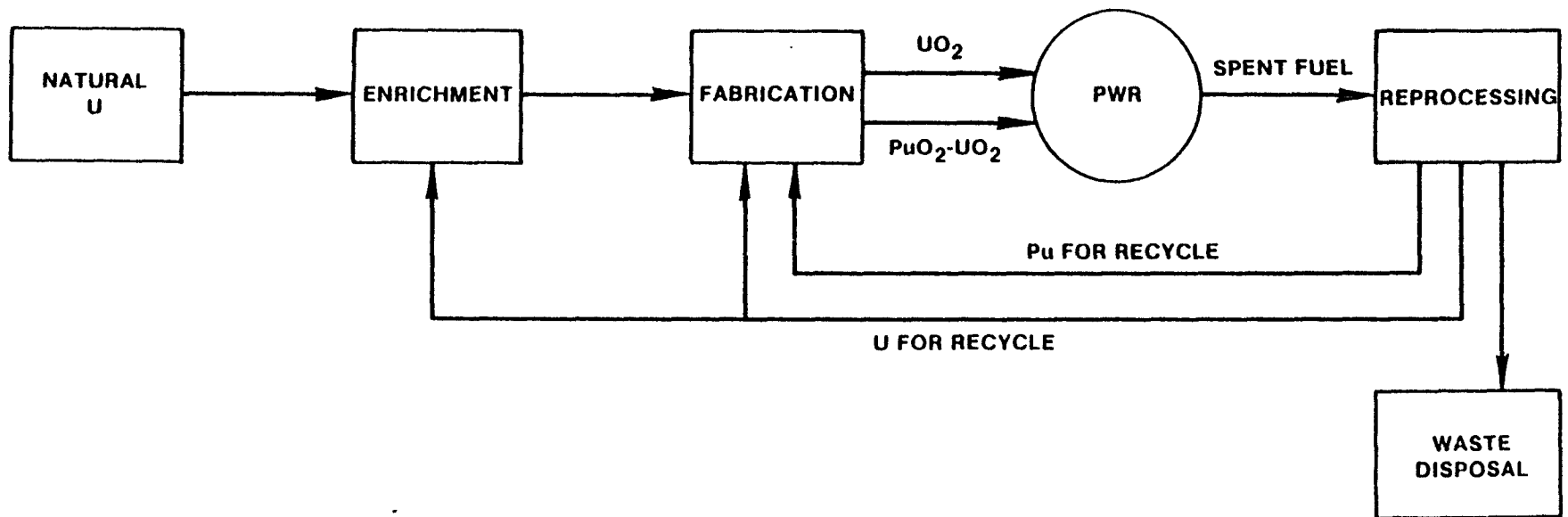
(B) PLUTONIUM AND URANIUM RECYCLE (PWR-U5(LE) + Pu(RE)/U)
