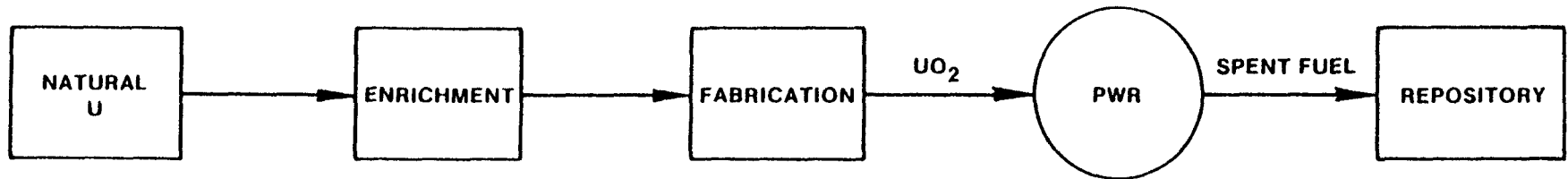
FIGURE E-1 LWR FUEL CYCLE
