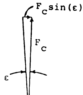
(b) Chordwise Centrifugal Force
