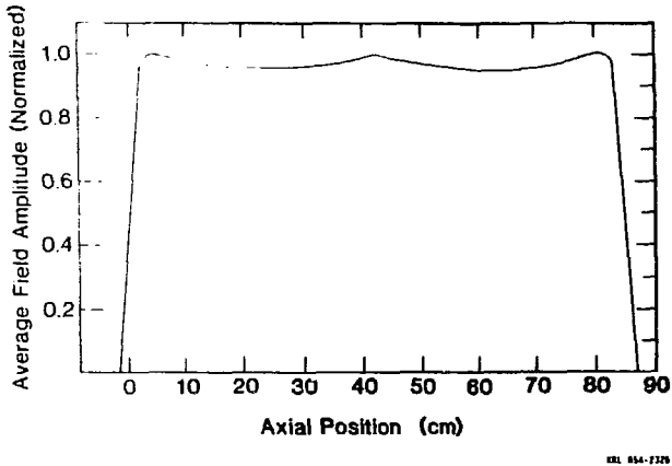
Fig. 2 Longitudinal field variations measured by bead pull perturbation techniques.
