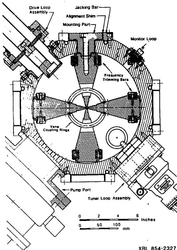
Fig. 1 Composite cross sectional view of the RFQ.
