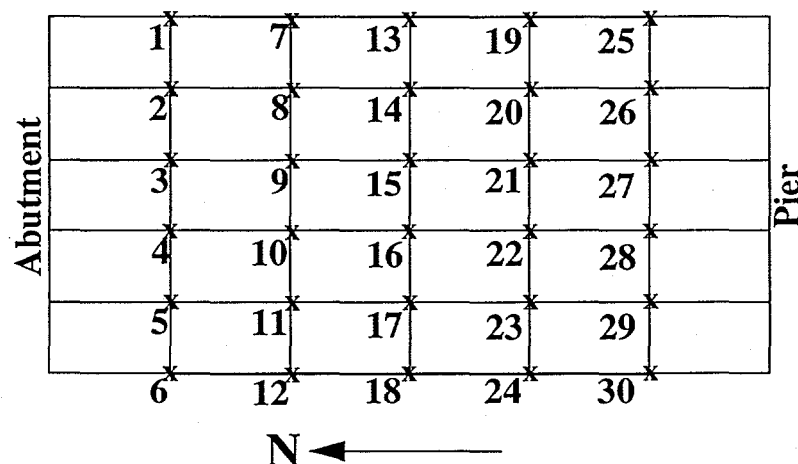
Figure 6: Accelerometer and Impact Locations
