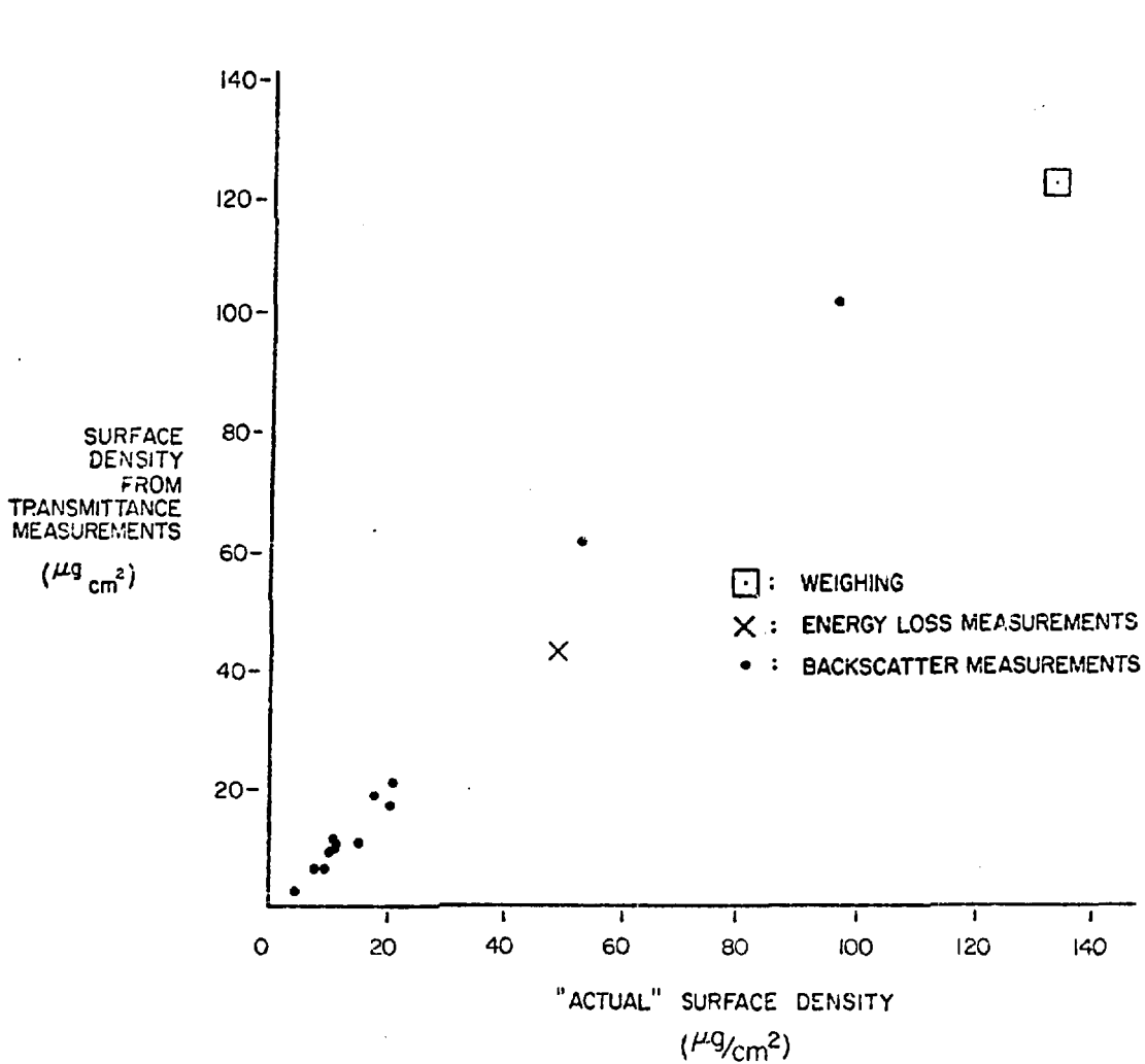
Fig. 1 Measurements by weighing, energy losses, and backscattering rates verify that the transmittance measurements provide useful indicators of surface densities of carbon foils (from private communication from B. Curnutte).
