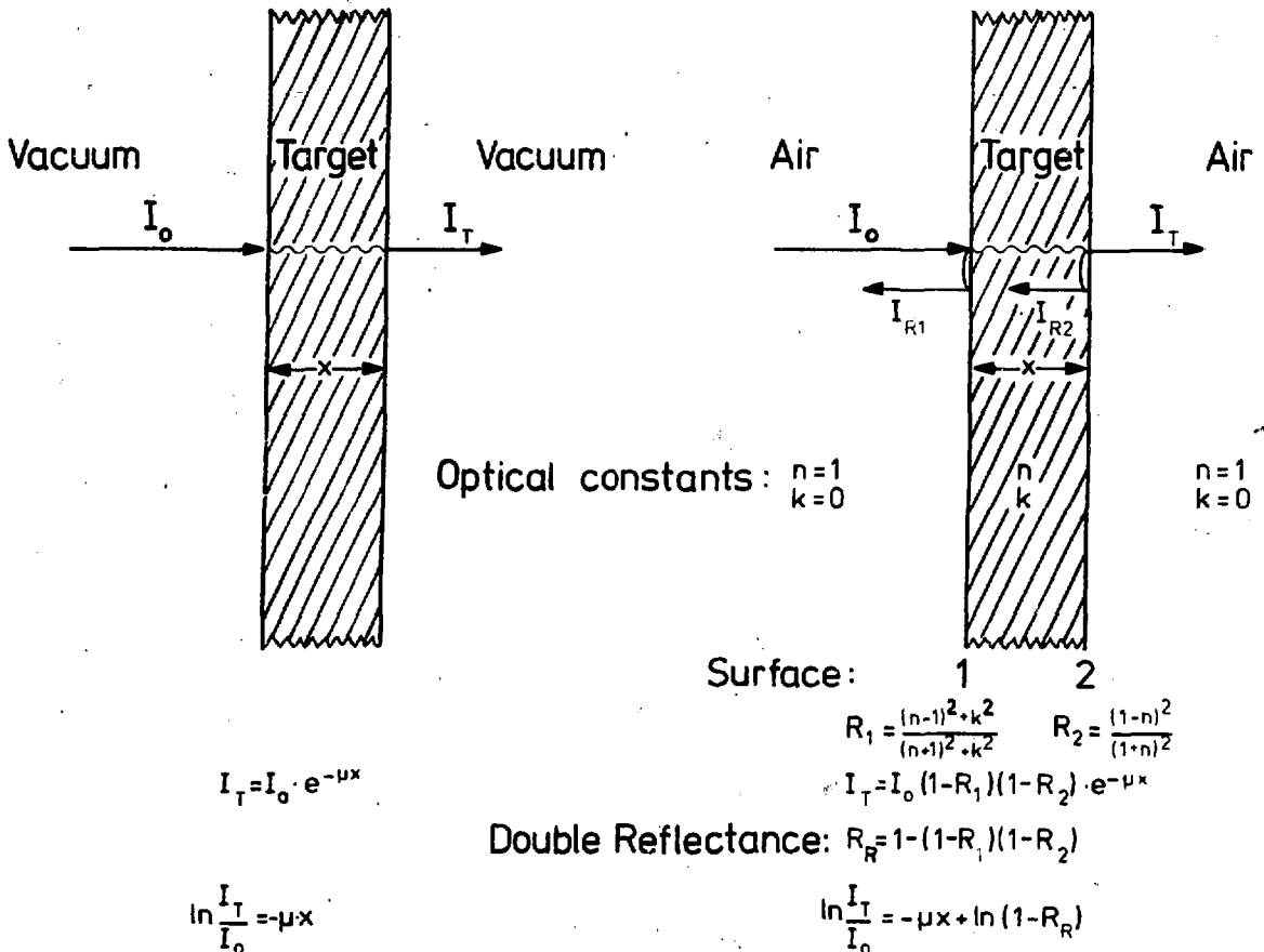
Fig. 1: Calculations of transmittance and double reflectance.
