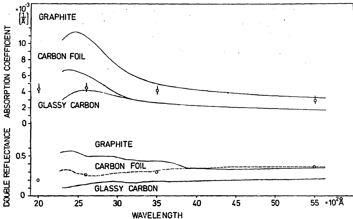
Fig. 3: Double reflectance and absorption coefficient as a function of wavelength.
