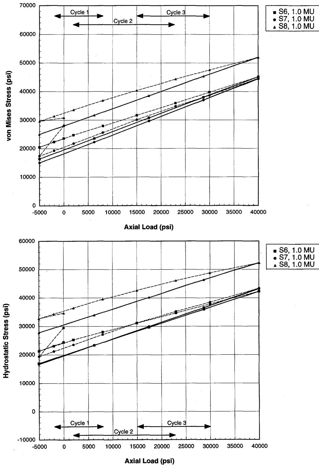
Figure 29. Von Mises and hydrostatic stress at the root of the last engaged box thread as a function of applied axial load for various coupling sizes.
