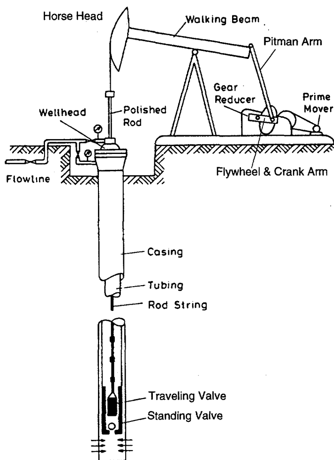
Figure 1. Illustration of sucker rod pump.
