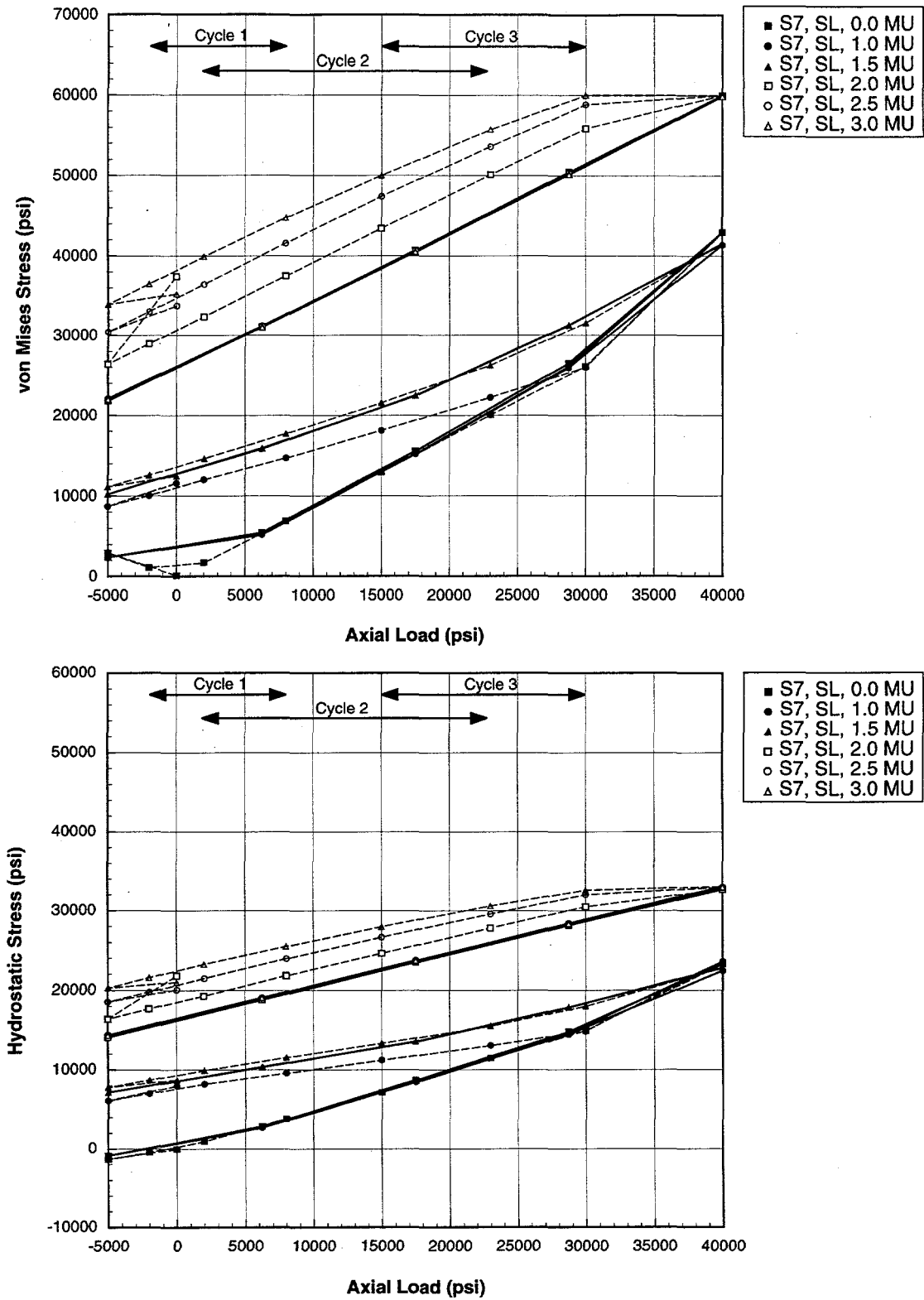
Figure 32. Von Mises and hydrostatic stress at the root of the last engaged box thread as a function of applied axial load for the Spiralock coupling with make-ups of 0.0, 1.0, 1.5, 2.0, 2.5, and 3.0.
