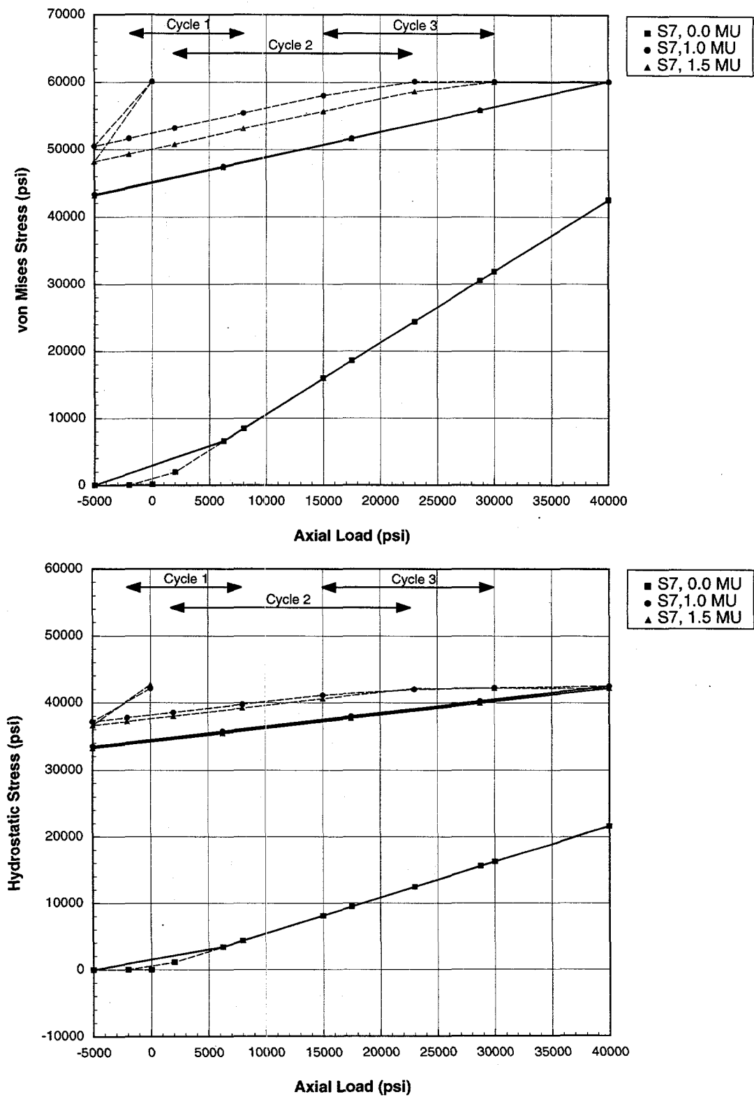
Figure 22. Von Mises and hydrostatic stress at the root of the first engaged pin thread as a function of applied axial load for various make-ups of the 7/8-inch API coupling.
