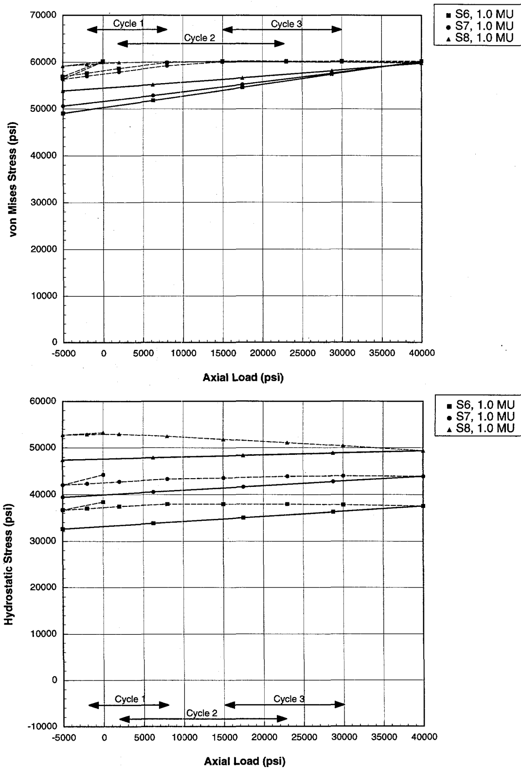
Figure 25. Von Mises and hydrostatic stress at the pin neck as a function of applied axial load for various coupling sizes.
