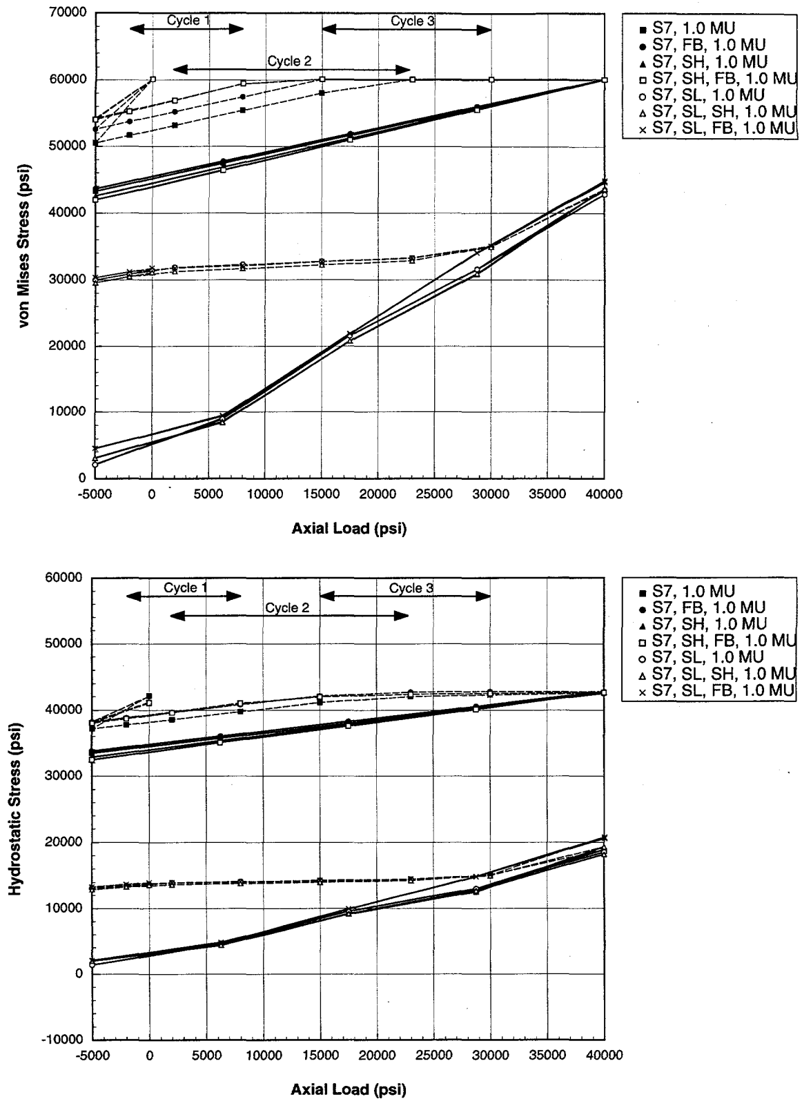
Figure 23. Von Mises and hydrostatic stress at the root of the first engaged pin thread as a function of applied axial load for various combinations of the Flexbar (FB), slimhole (SH), and Spiralock (SL) modifications to the base coupling (S7).
