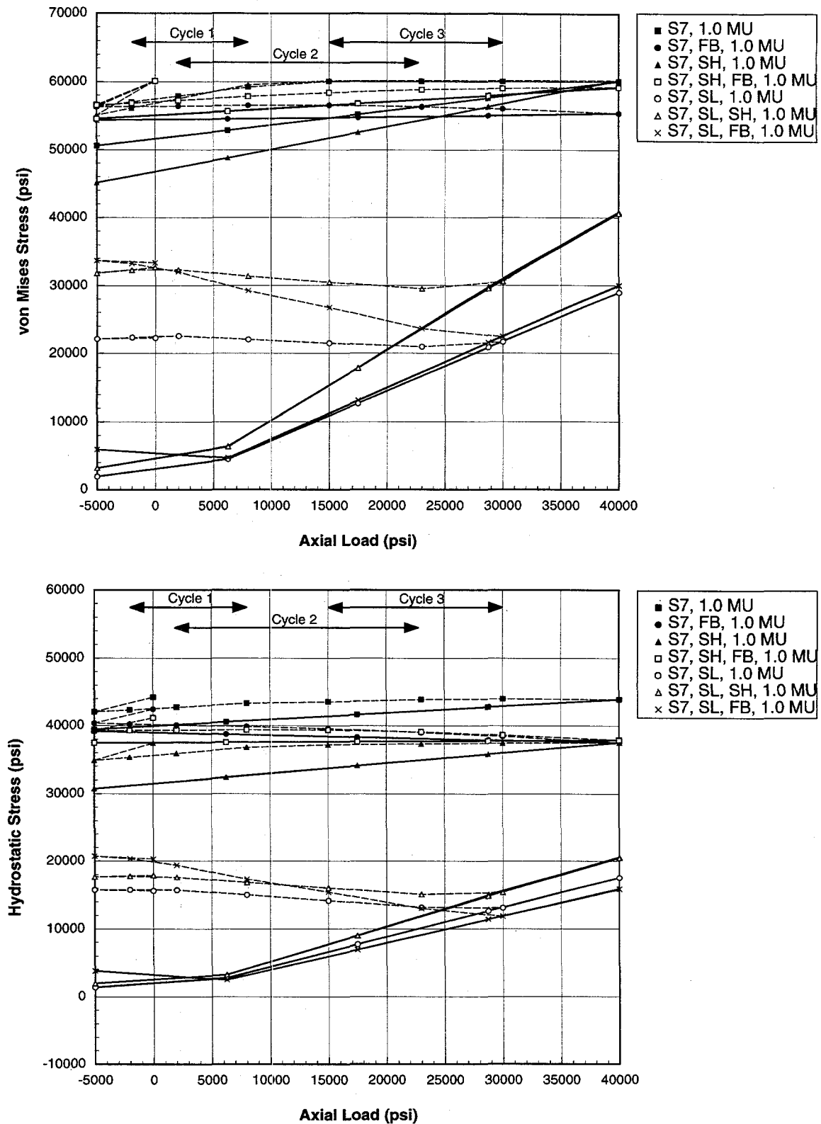
Figure 27. Von Mises and hydrostatic stress at the pin neck as a function of applied axial load for various combinations of the Flexbar (FB), slimhole (SH), and Spiralock (SL) modifications to the base coupling (S7).
