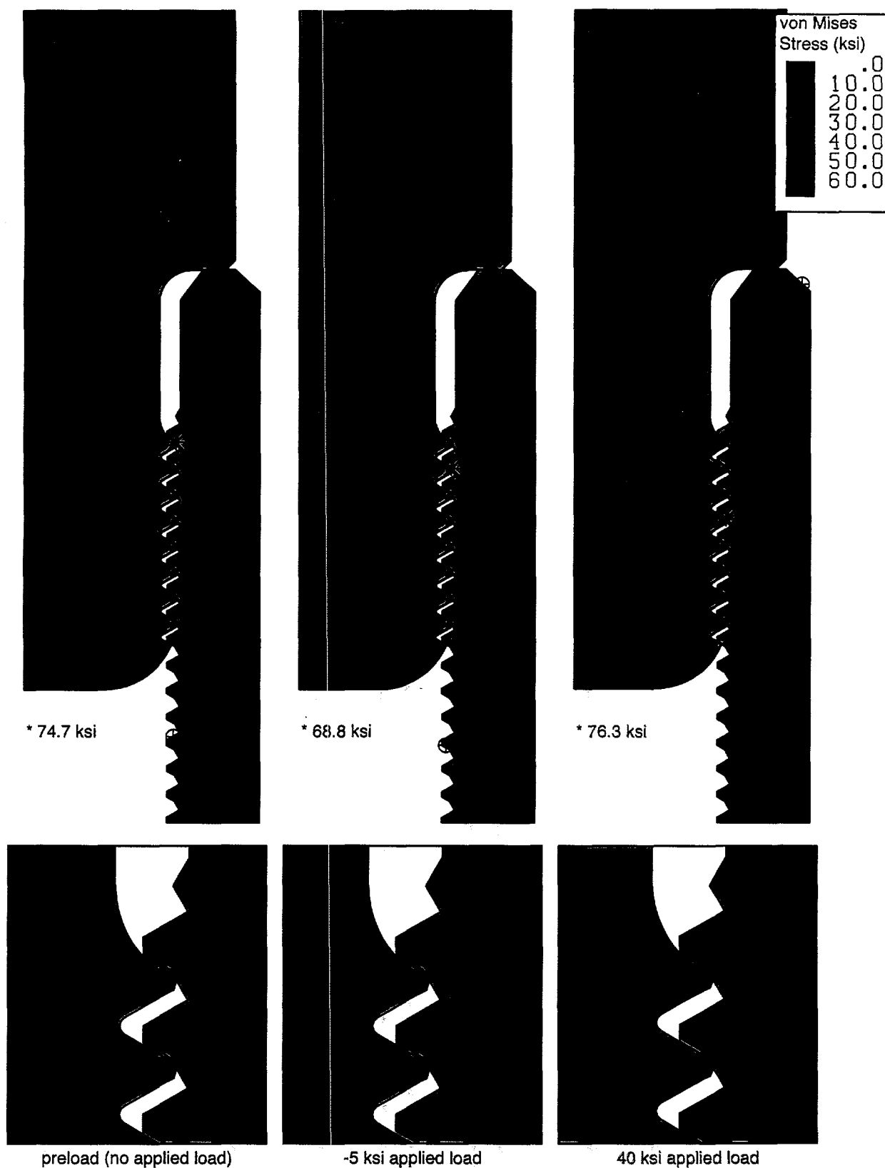
Figure 9. Von Mises stress distribution (ksi) in the 7/8-inch Spirallock coupling (Analysis 12) at preload, maximum compression, and maximum tensile loads.
