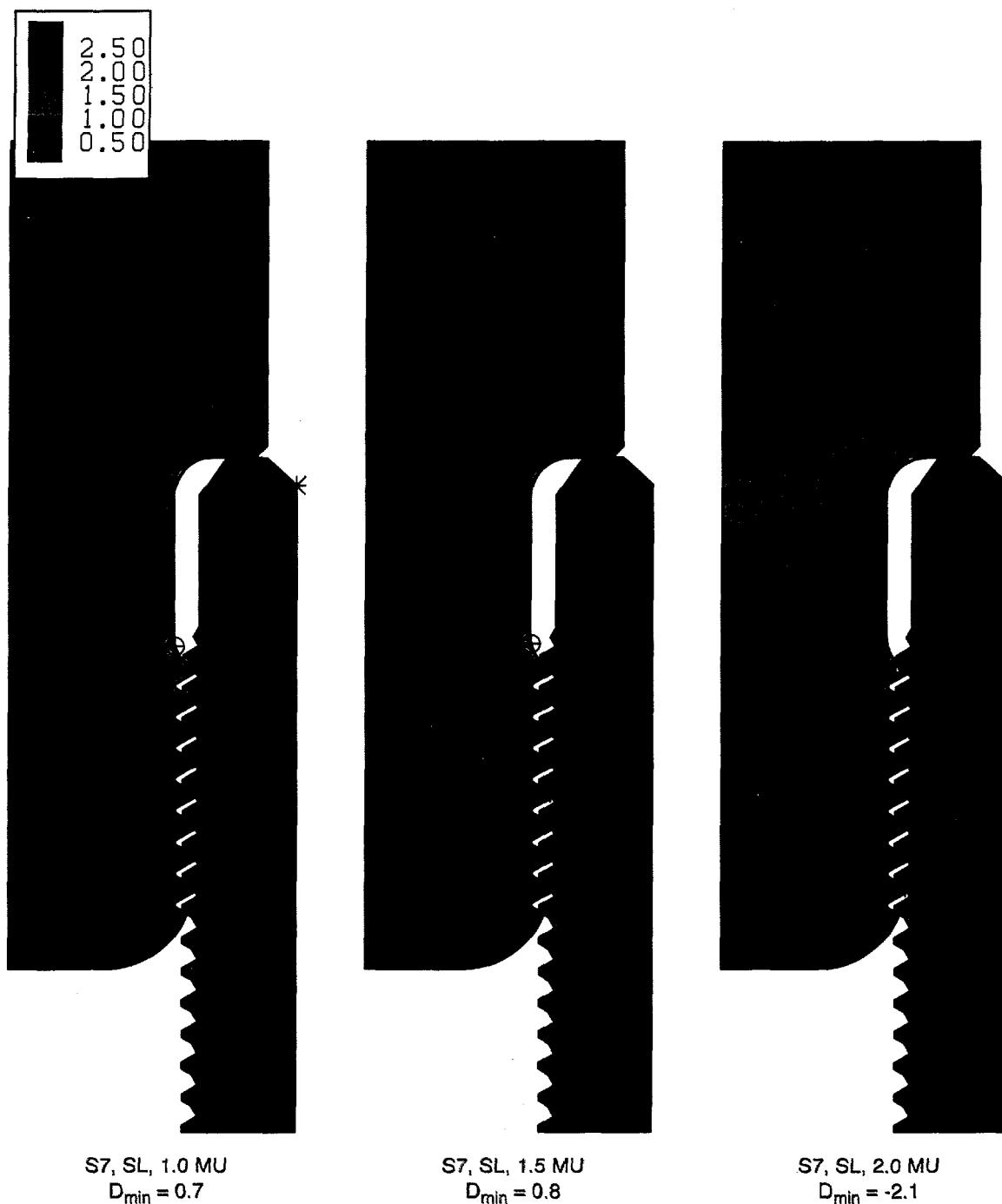
Figure 33. Fatigue safety factor distribution in the 7/8-inch Spirallock coupling (with make-ups of 1.0, 1.5, and 2.0) subjected to the full axial load range (-5 ksi to 40 ksi).
