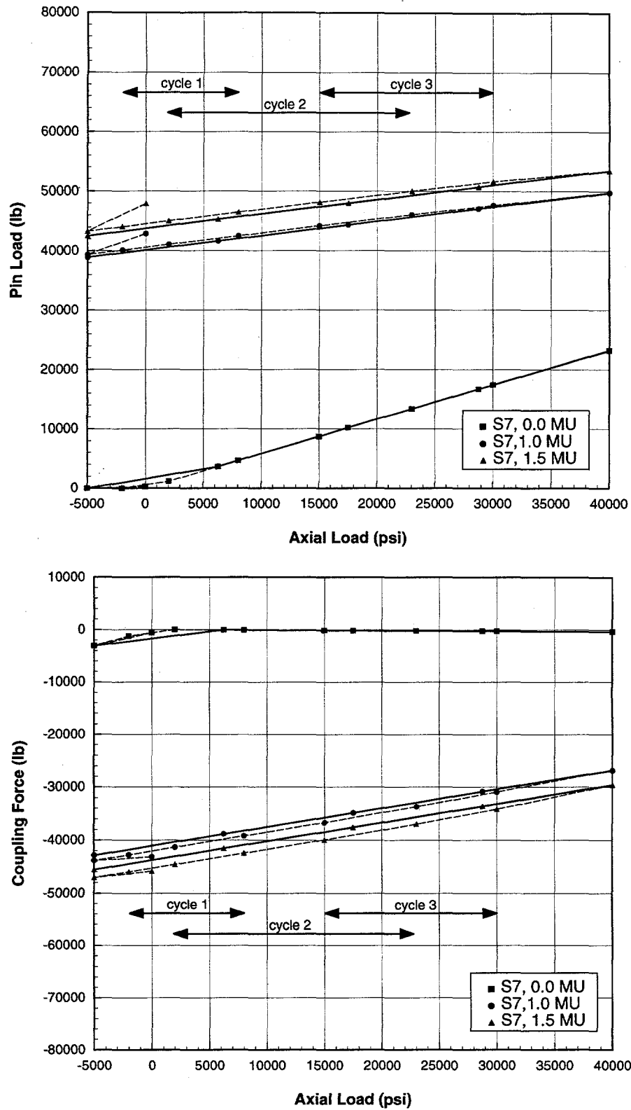
Figure 12. Pin load and coupling force as a function of axial load for the 7/8-inch standard API coupling size (S7) with make-ups of 0.0, 1.0, and 1.5.
