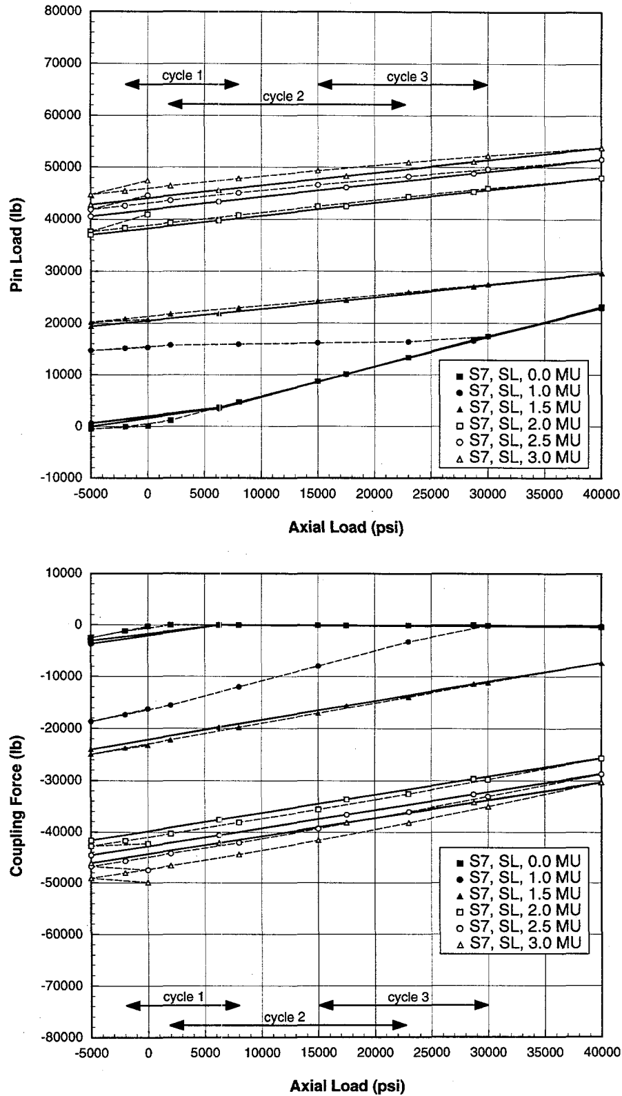
Figure 14. Pin load and coupling force as a function of axial load for the base geometry (S7) with Spirallock threads (SL) and make-ups of 0.0, 1.0, 1.5, 2.0, 2.5, and 3.0.
