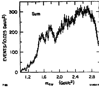
Fig. 9. Unsubtracted invariant 4\pi mass distribution. Shown is the sum of J/\psi \rightarrow \gamma\pi^+\pi^-\pi^+\pi^- and J/\psi \rightarrow \gamma\pi^+\pi^-\pi^0\pi^0 (Mark III).
