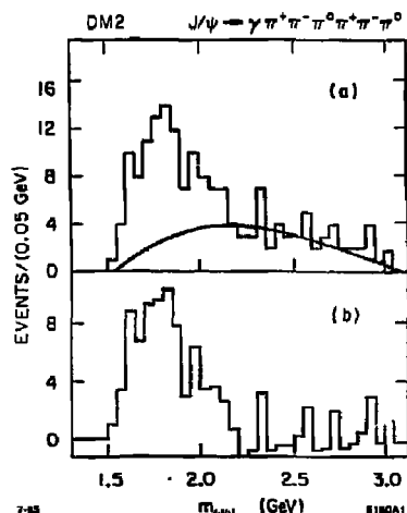
Fig. 12. (a) Invariant \omega\omega mass distribution (DM2). The curve is the background estimate. (b) Background subtracted \omega\omega mass distribution.
