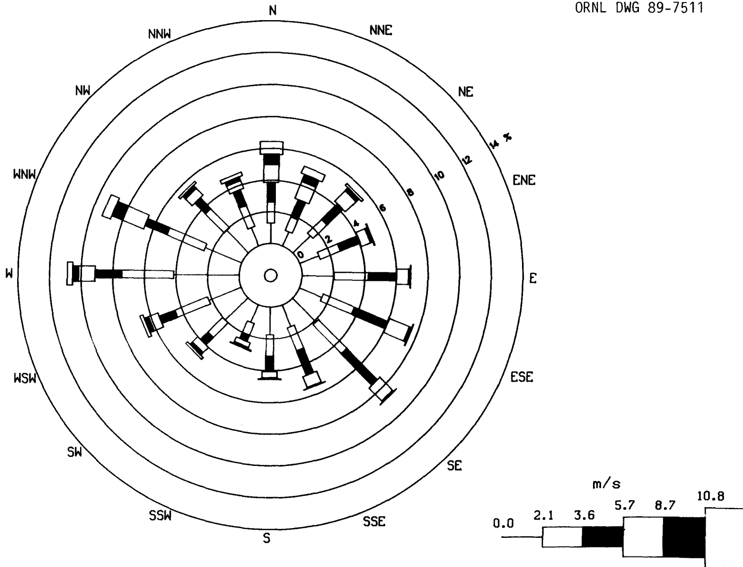
Fig. 3.2 Wind rose for Pueblo Depot Activity - Station 93058 for January 1, 1960-December 31, 1964
