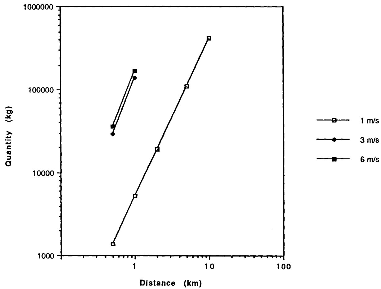
Fig. D.1. HD agent, continuous (evaporation) release.
