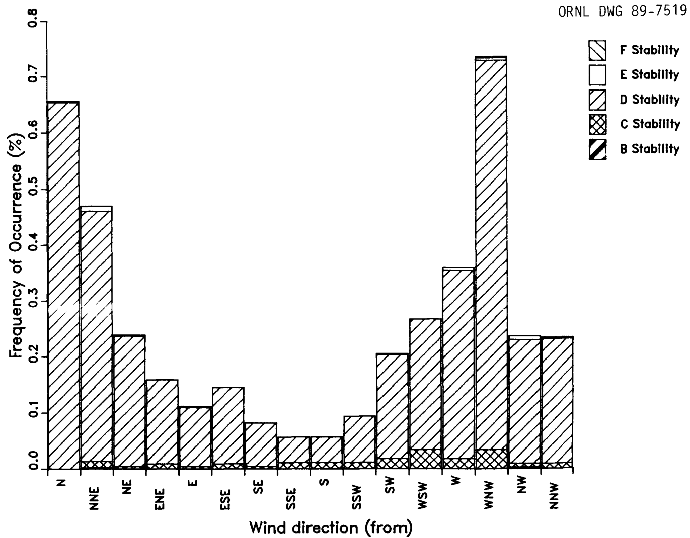
Fig. B.5 Distribution of wind directions and stabilities for winds 8.7-10.8 m/s (Pueblo data, 1960-1964)
