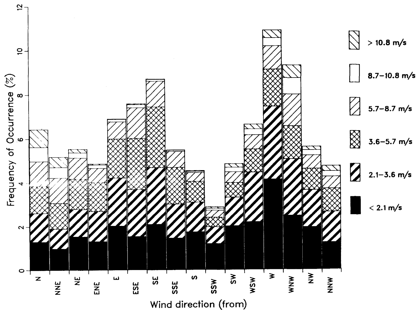
Fig. 3.3 Distribution of wind speeds and directions (Pueblo data, 1960-1964)
