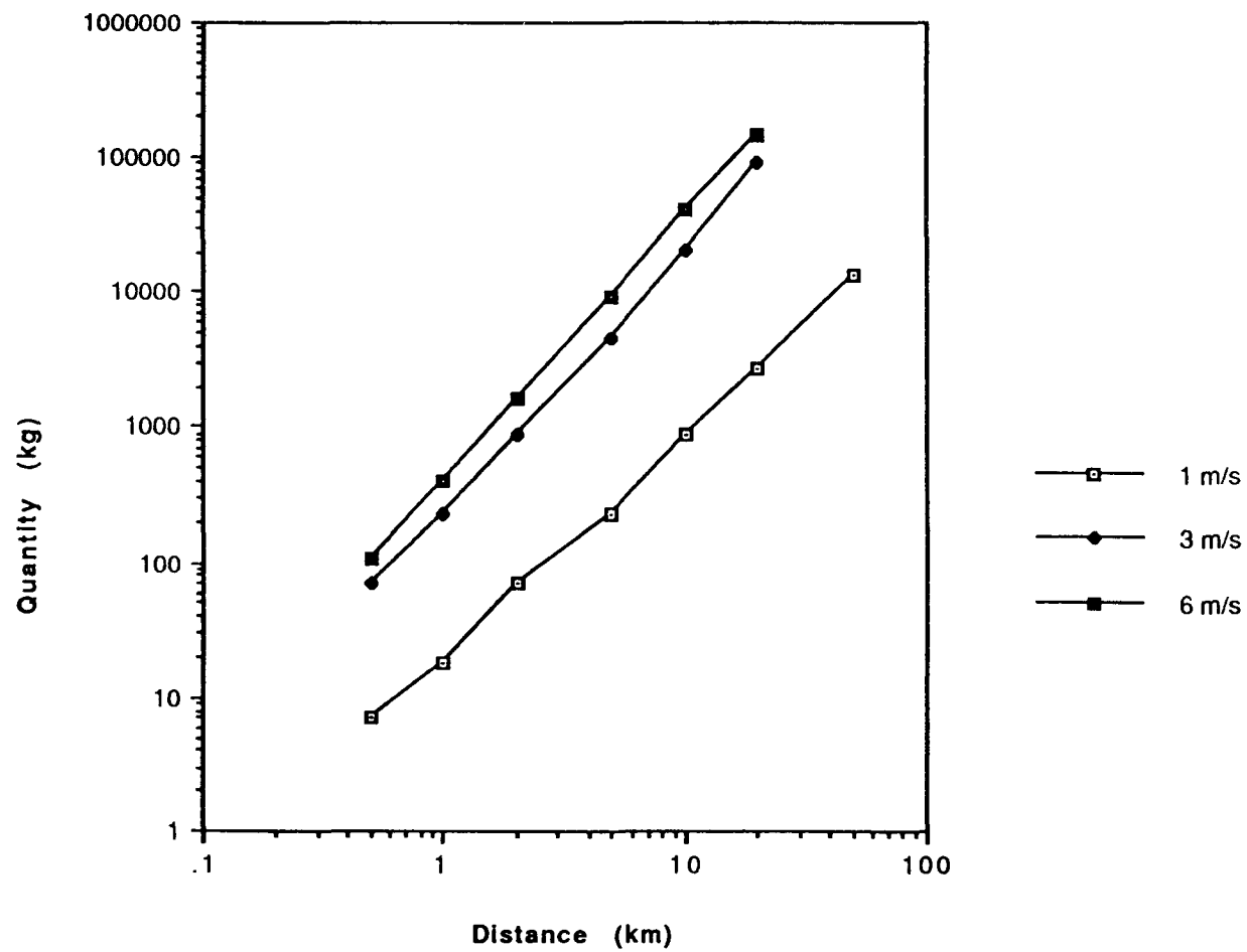
Fig. D.2. HD agent, semicontinuous release.
