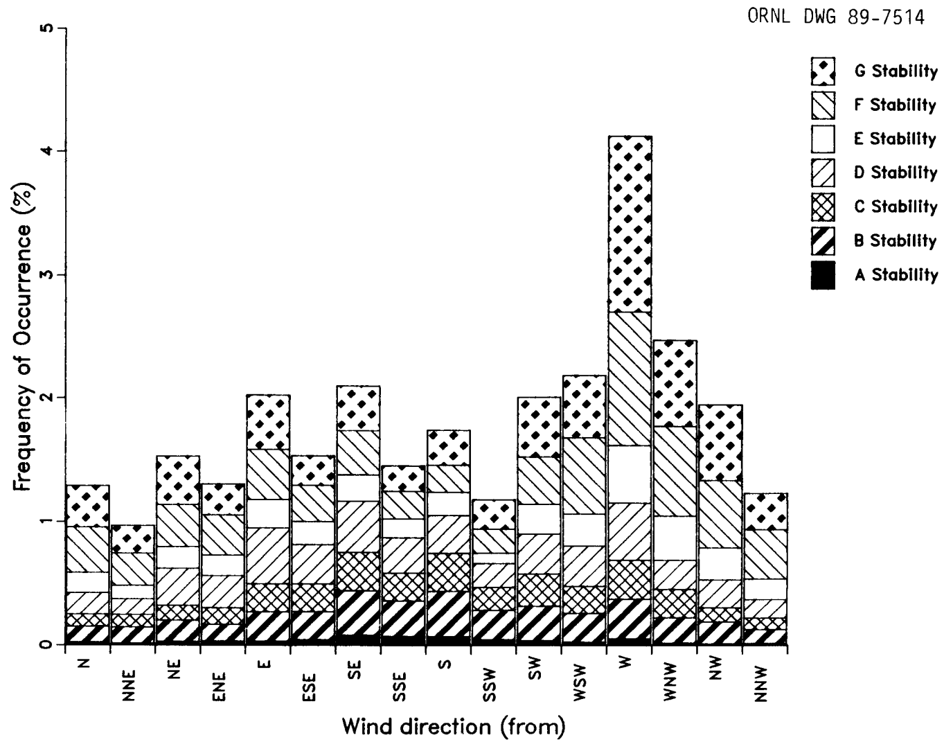
Fig. B.1 Distribution of wind directions and stabilities for winds <2.1 m/s (Pueblo data, 1960-1964)
