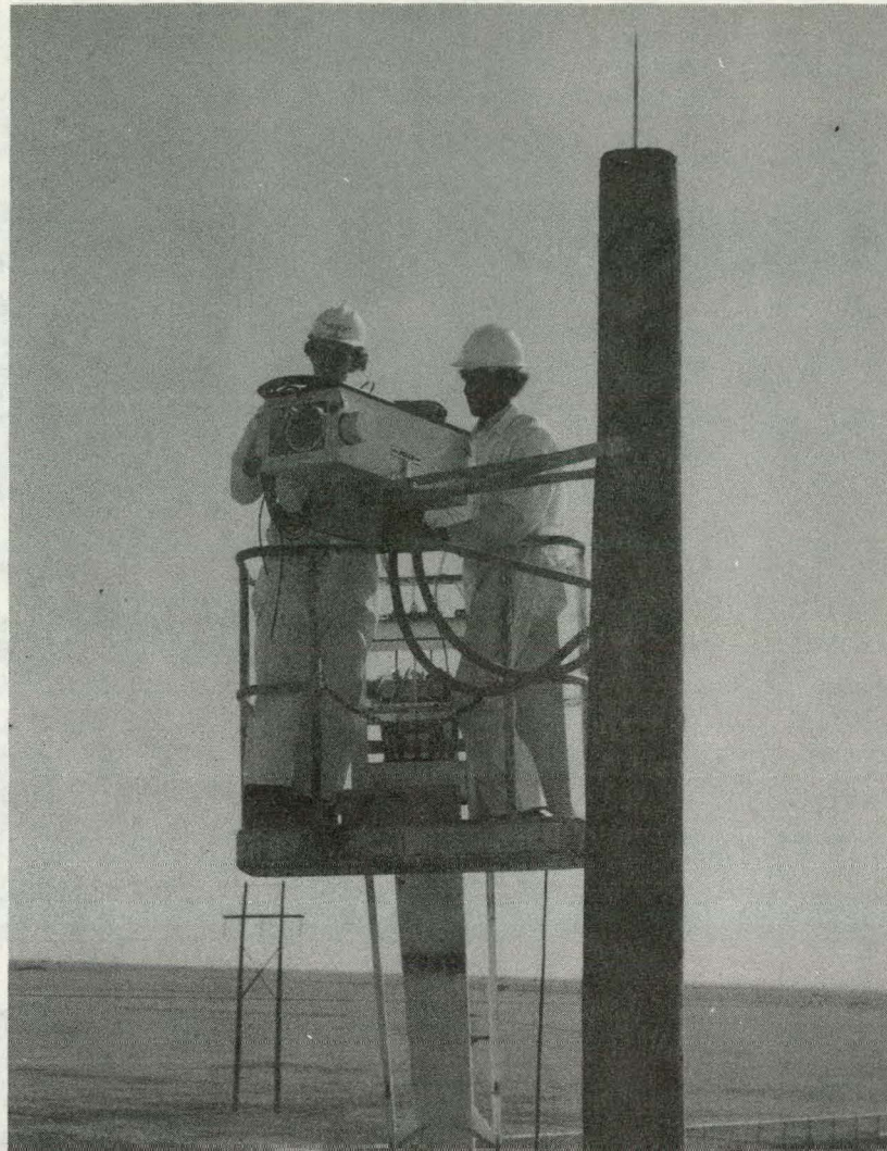
Figure B-2. Camera Installation
