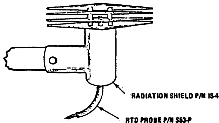
Figure 4. Temperature Sensor
