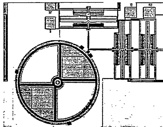
Figure 2. Two sets of linear comb-drive actuators driving the gear shown in Figure . This smaller gear drives a 1.6 mm diameter shutter in the lower left of the photo.
