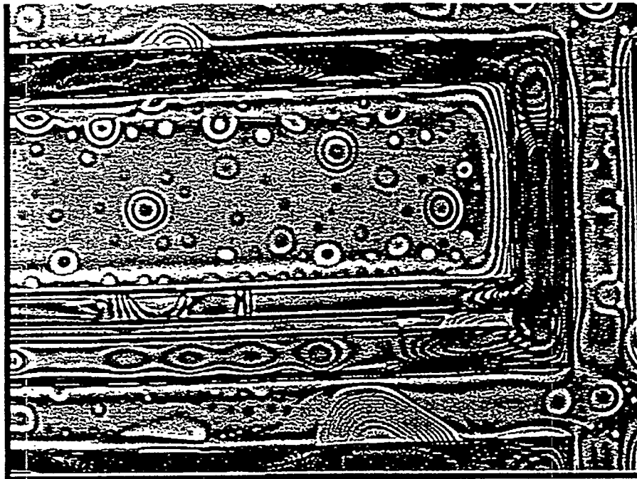
Figure 6. Example of chemical attack of the waveguide structure during the micromechanical release etch due to pinholes in the passivating nitride film. This device is non-functional due to the large number of pinholes.
