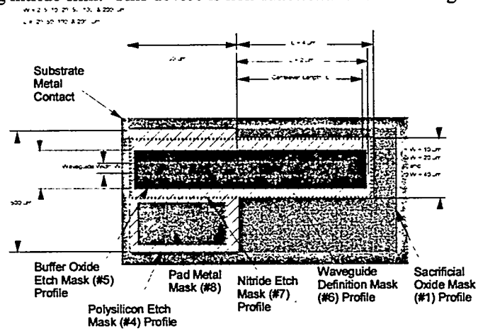
Figure 7. Layout, dimensions, and design rules of cantilevered waveguide test structures.
