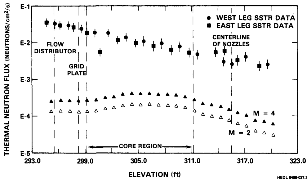
FIGURE 2. Thermal Neutron Fluxes in the TMI-2 Annular Gap. Overall experimental uncertainty is displayed at the 1 \sigma level. Neg 8501167-1
