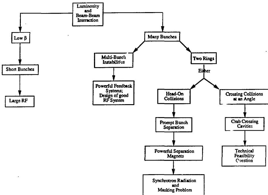
Fig. 1. Illustration of the alternatives that must be considered in the design of a high-luminosity electron-positron factory.
