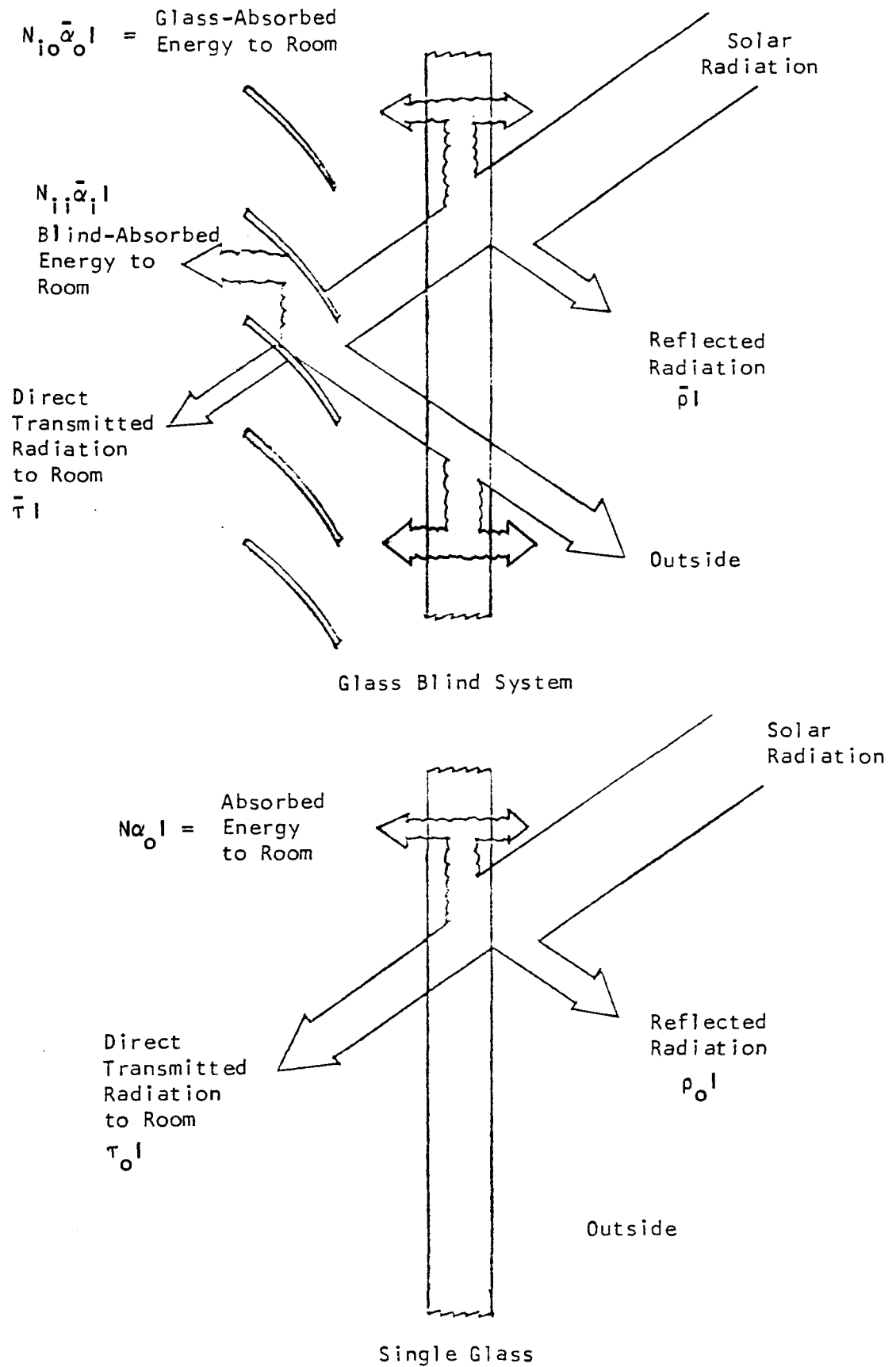
FIGURE 1. HEAT TRANSFER THROUGH SELECTED GLAZING SYSTEMS
