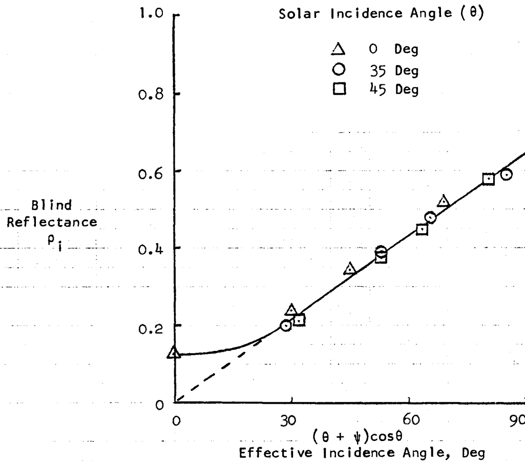
FIGURE 11. EFFECT OF SLAT ANGLE AND SOLAR INCIDENCE ON BLIND REFLECTANCE
