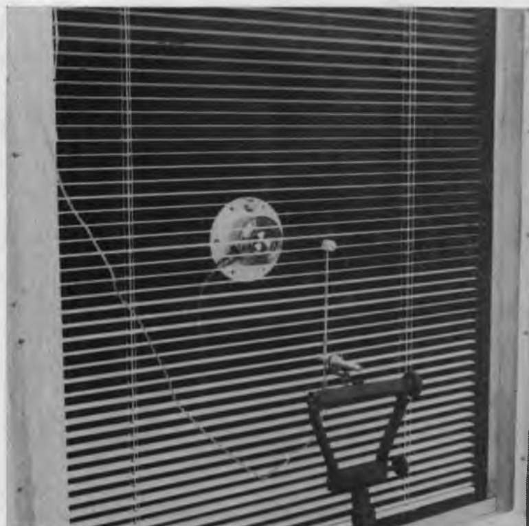
FIGURE 3. EXPERIMENTAL SETUP FOR MEASURING TRANSMITTANCE AND REFLECTANCE
