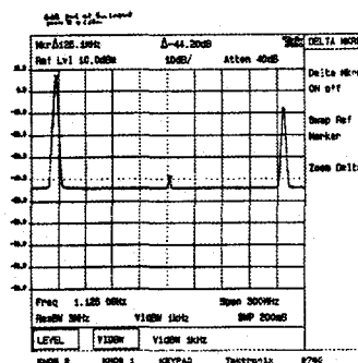
Fig. 6. Back-end kick QPSK spectrum (10dB/div).
