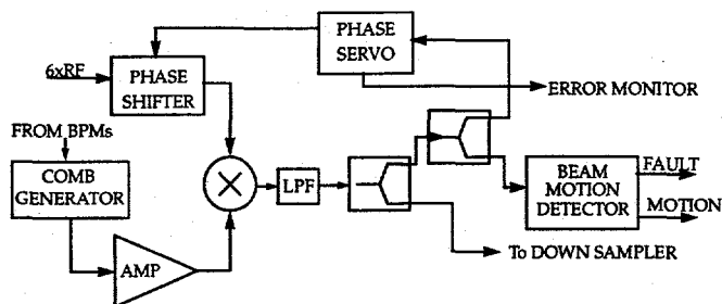
Fig. 3. Block Diagram of Front-end Module
