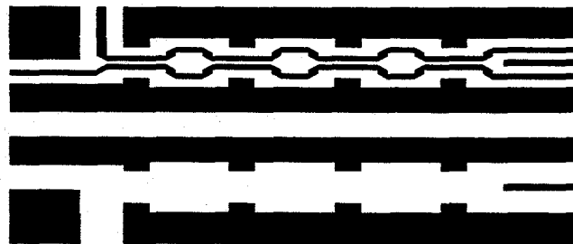
Fig. 2. Stripline Comb Generator.
