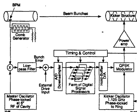
Fig. 1. Block Diagram of the Longitudinal Feedback System.
