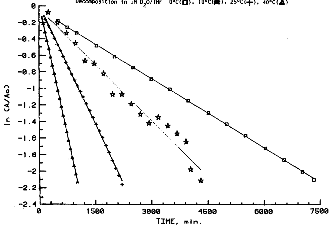
Figure I-16: m -Fluorophenyluranocene
