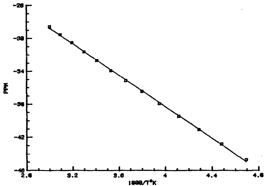
Figure 2-5: Plot of Chemical Shift vs. Inverse Temperature for (\text{COT})\text{UCl}_2 \cdot 2 \text{ THF}
