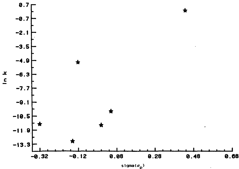
FIGURE 1-6: PLOT OF (C_6H_7X)_2U HYDROLYSIS RATE CONSTANTS VERSUS SIGMA PARA VALUES
