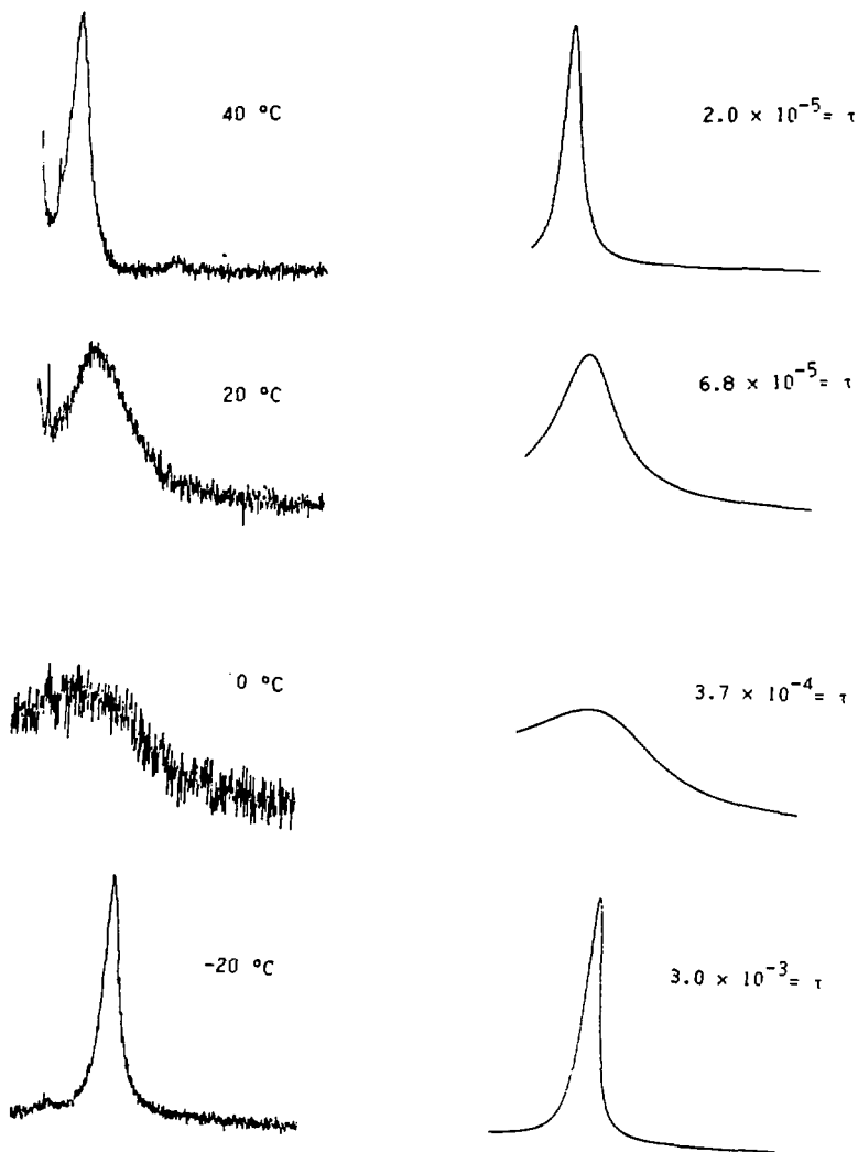
Figure 2-10: Line Shape Analysis for \text{PMe}_3 Exchange
