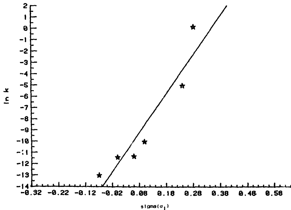
FIGURE 1-8: CORRELATION OF HYDROLYSIS RATE CON- STANTS OF (C_6H_7X)_2U WITH TAFT \sigma_1 CONSTANTS
