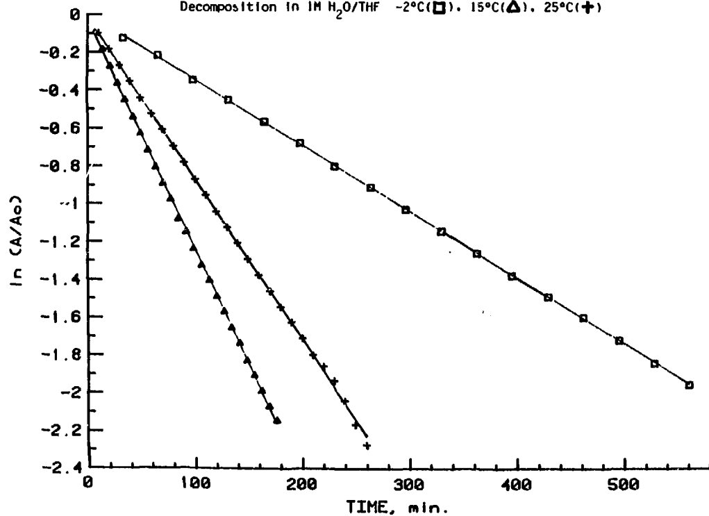
Figure 1-11: m -Fluorophenyluranocence
