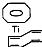
FIGURE 1-5
