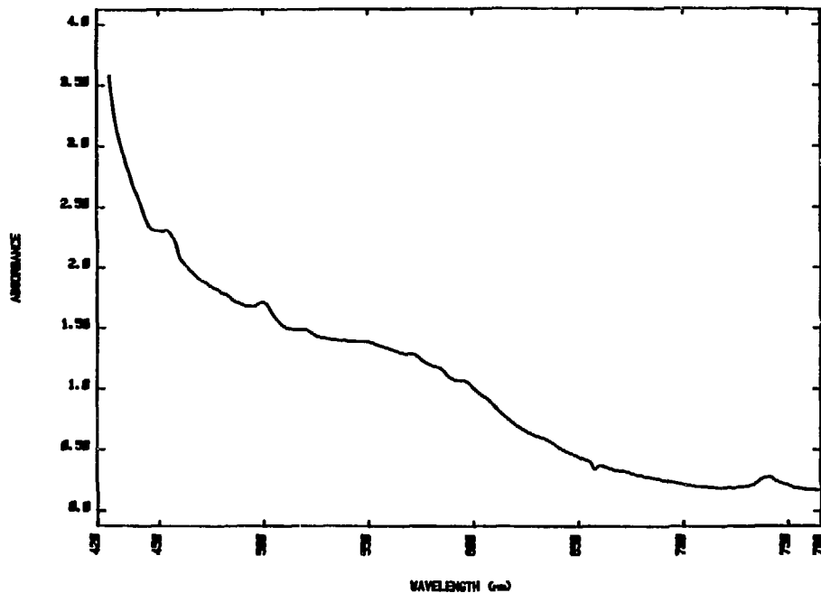
Figure 2-4: Visible Spectrum of (COT)UCI 2 -2 THF in THF
