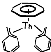
Figure 2-6: ([8]Annulene)thorium- \eta^3 -Dibenzyl
