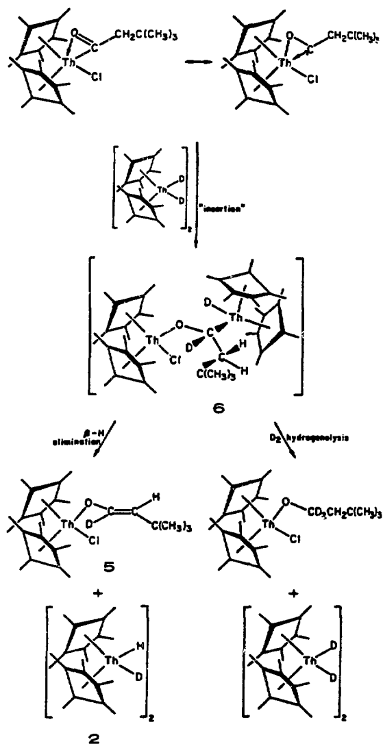
FIGURE 1-3
