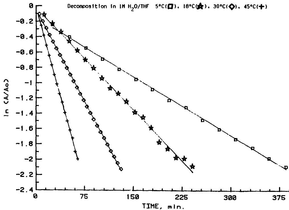
Figure I-12: m -Fluorophenyluranocene
