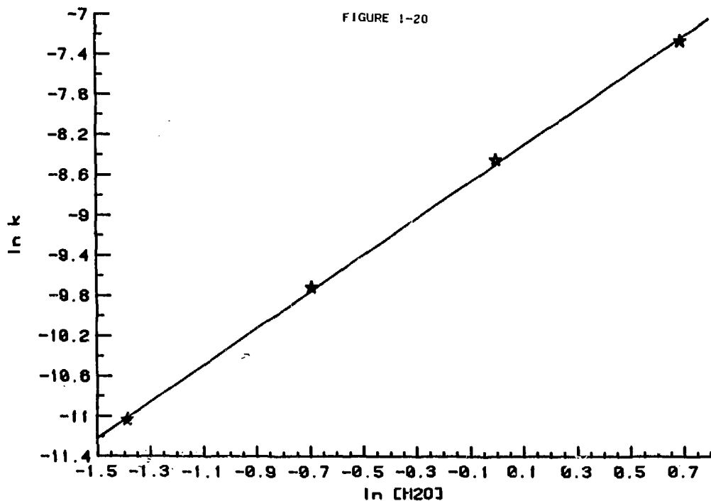
Plot of \ln k vs. [\text{H}_2\text{O}] to Determine Rate Order of Water in the Decomposition of m -Fluorophenyluranocene
