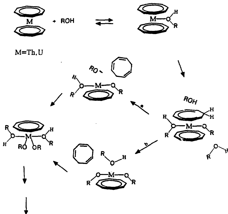
FIGURE 1-26
