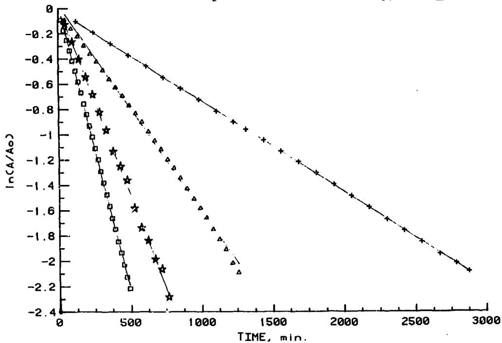
Figure 1-14: m -Fluorophenyluranocene
