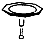
FIGURE 1-27
