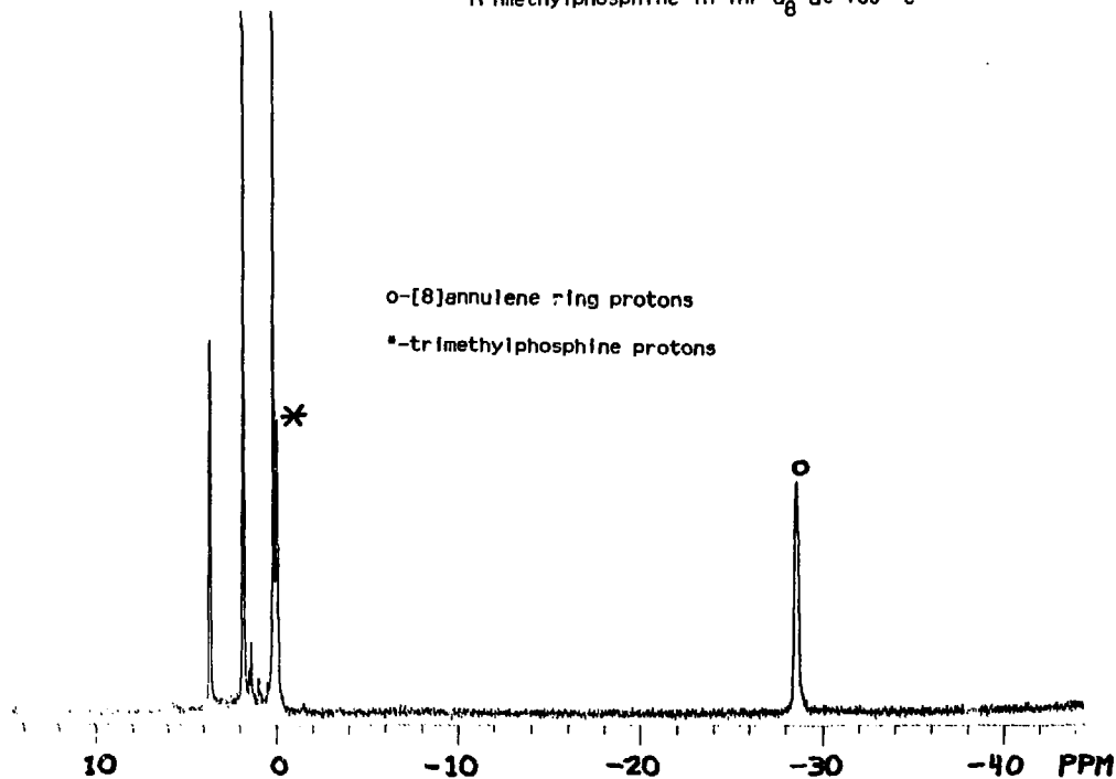
Figure 2-7: ^1\text{H} NMR of ([\text{8}]\text{Annulene})\text{uranium Dichloride} Trimethylphosphine in \text{THF-d}_8 at +60^\circ\text{C}
