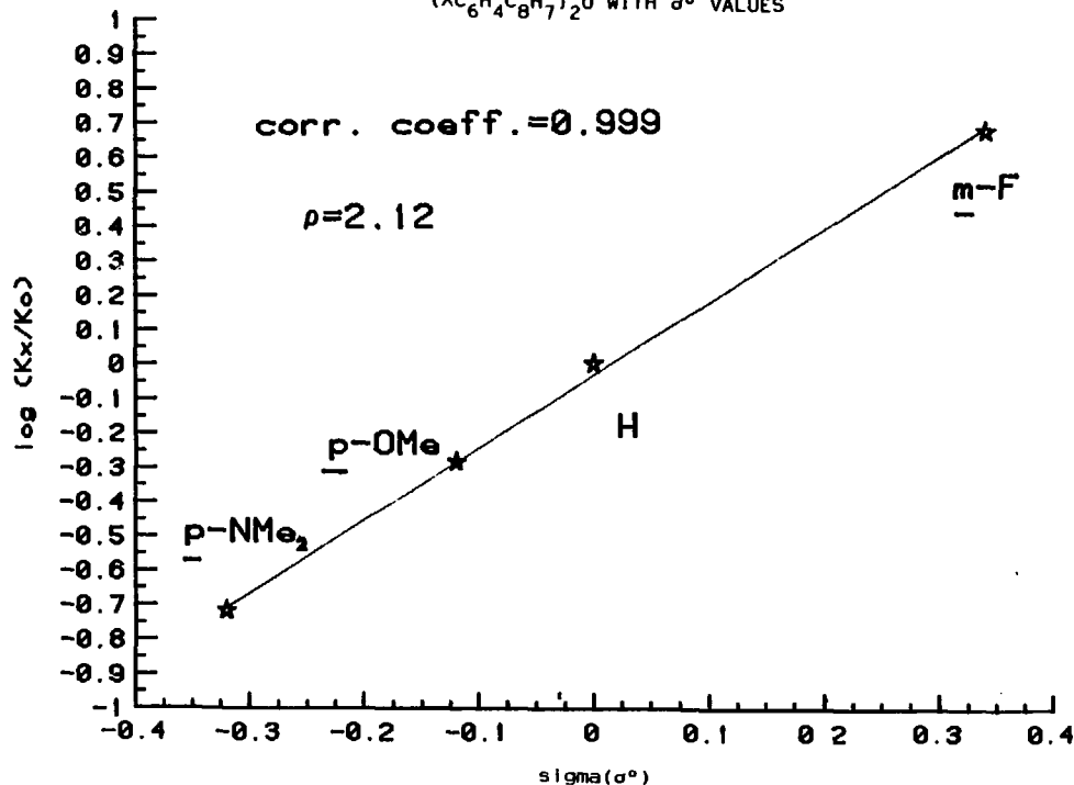
FIGURE 1-10: CORRELATION OF HYDROLYSIS RATE CONSTANTS OF (XC_6H_4C_6H_7)_2U WITH \sigma^\circ VALUES
