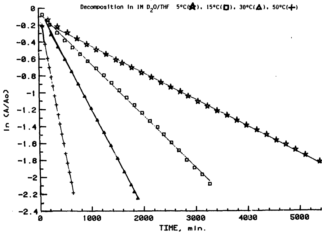
Figure 1-15: m -Fluorophenyluranocene
