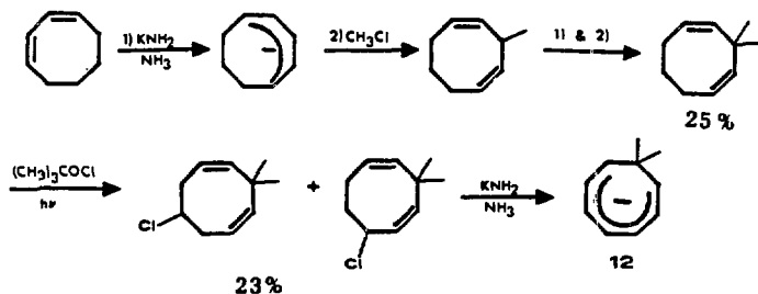
FIGURE 1-24
