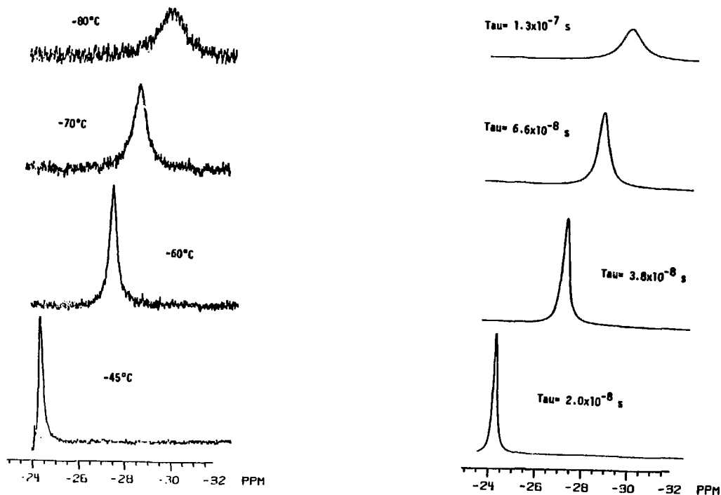
Figure 3-2: Line Shape Analysis for ortho -proton coalescence in 1,1'-Diphenyluranocene
