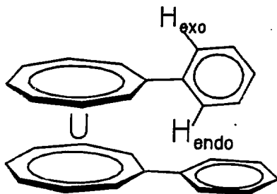
Figure 3-1: 1,1'-Diphenyluranocene, 1
